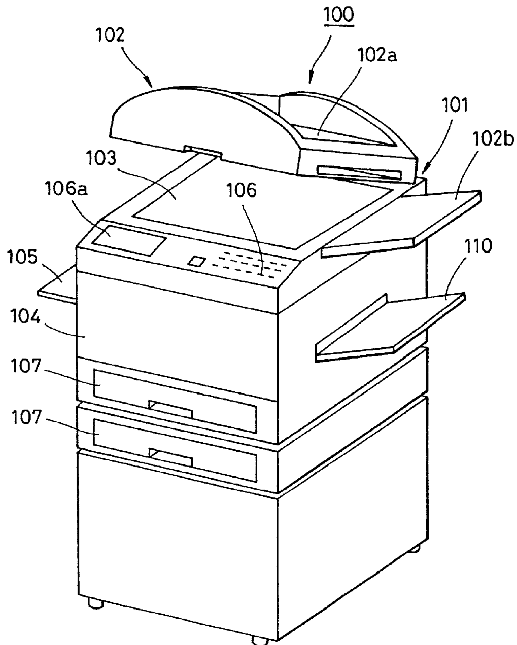
FIG. 8 PRIOR ART
