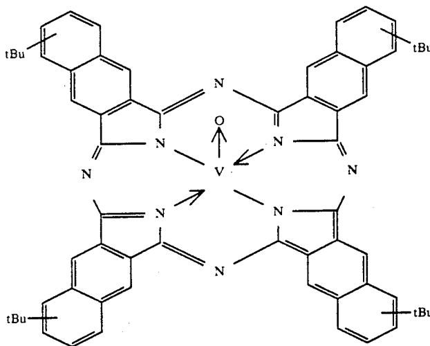
Vanadyl-tetra(t-butyl)naphthalocyanine
