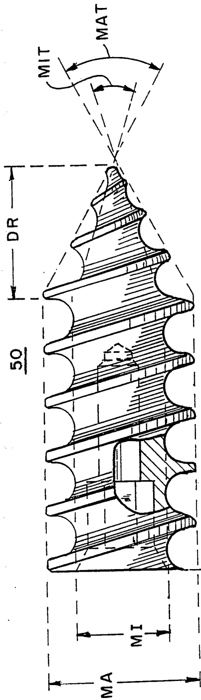
FIG. 3 (PRIOR ART)
