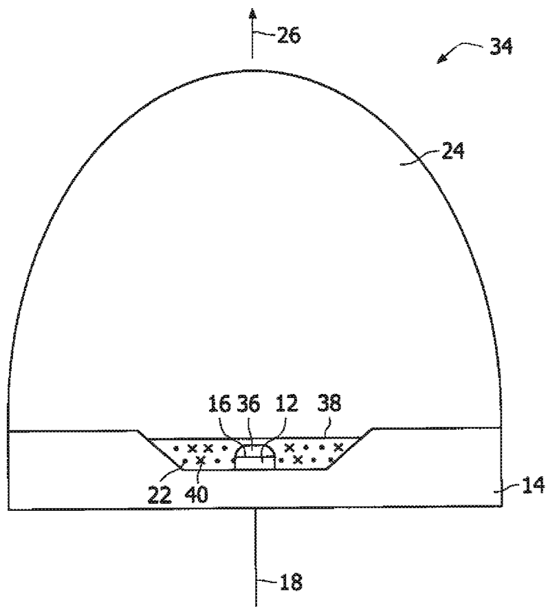
FIG. 1 (PRIOR ART)
