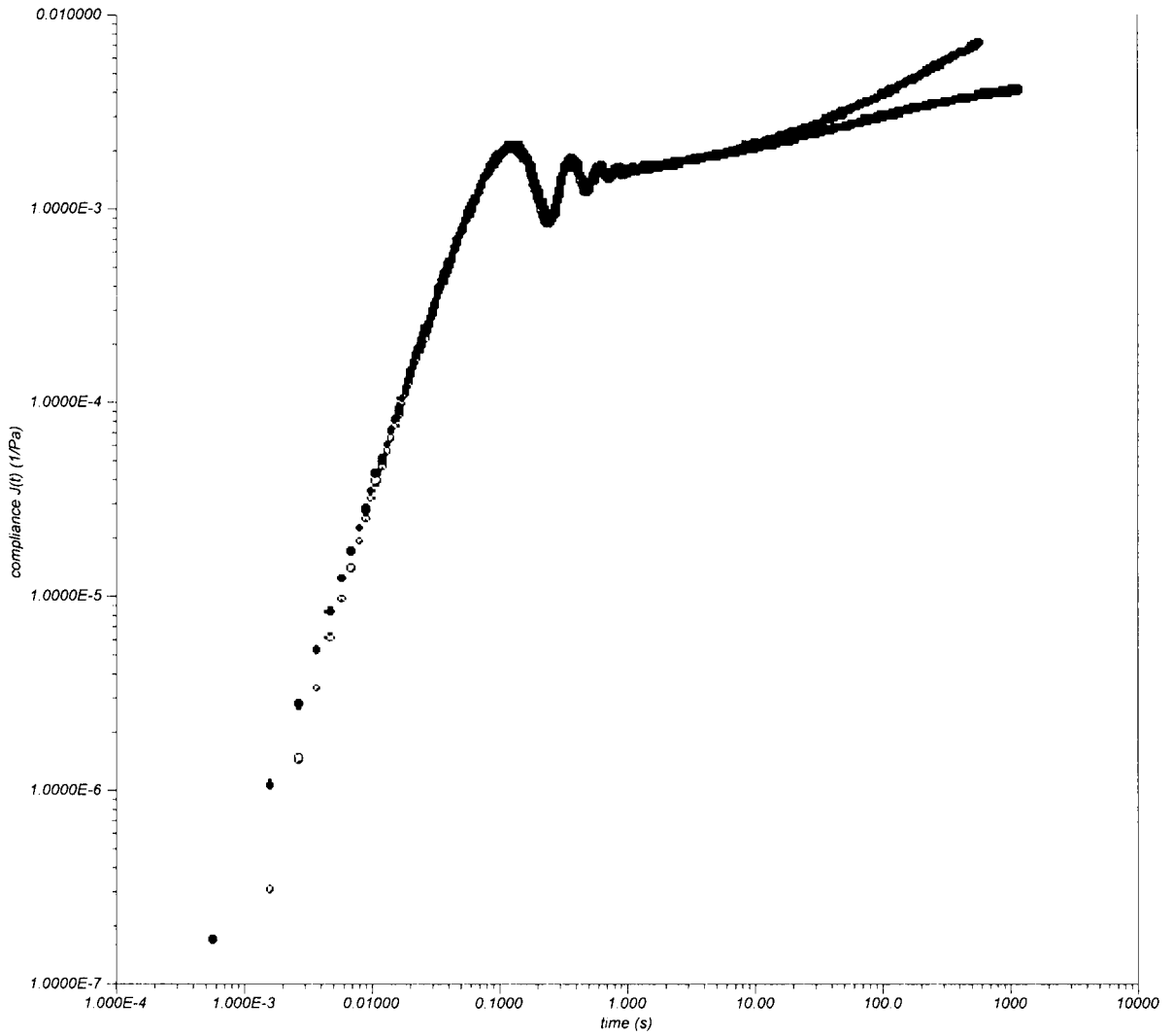
FIGURE 2: Creep and Recovery Compliances at Constant Stress = 10Pa for Example 4
