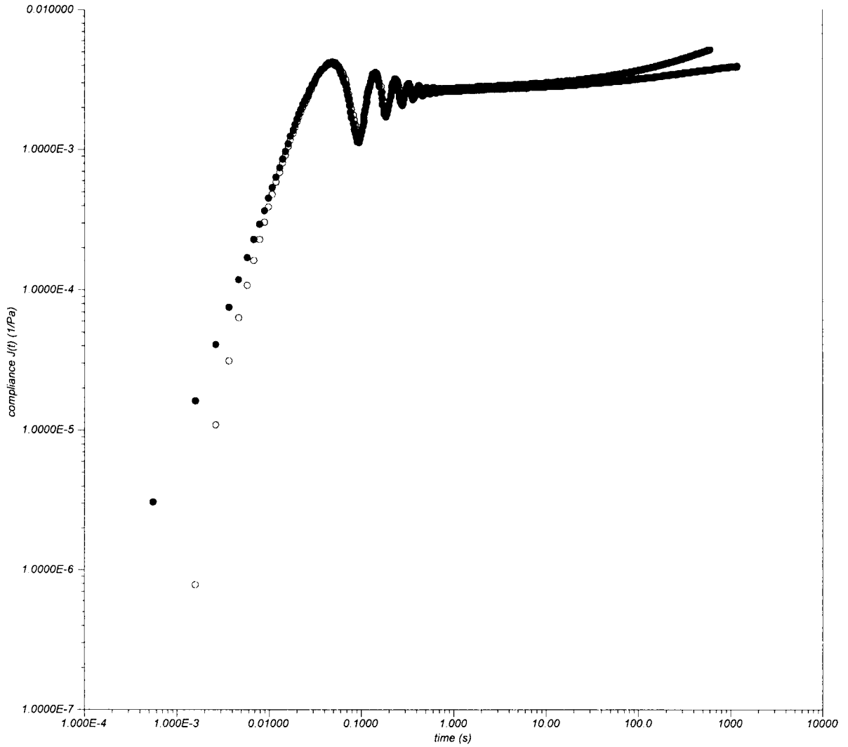
FIGURE 1: Creep and Recovery Compliances at Constant Stress = 10Pa for Example 1
