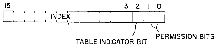
SEGMENT SELECTOR FORMAT IN PROTECTED MODE
