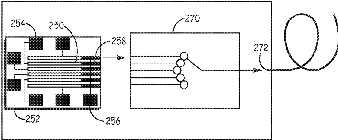
FIG. 6 (Prior Art)
