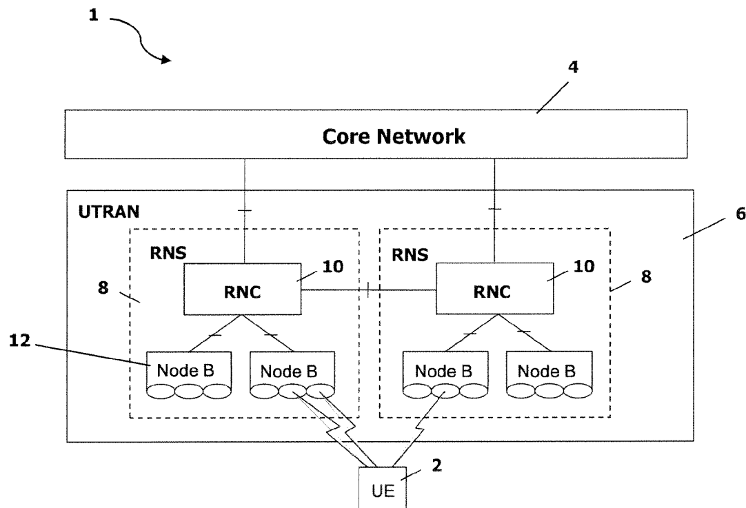
FIG. 1 RELATED ART
