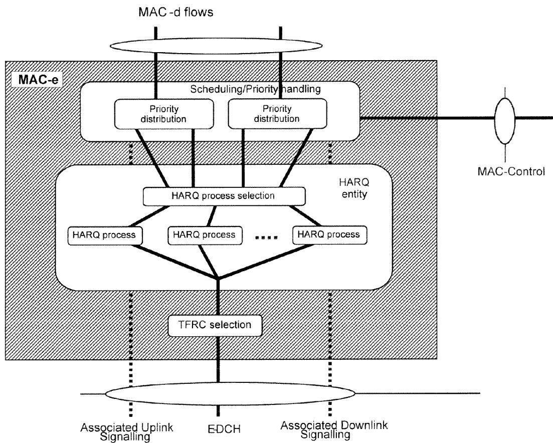
FIG. 6 RELATED ART
