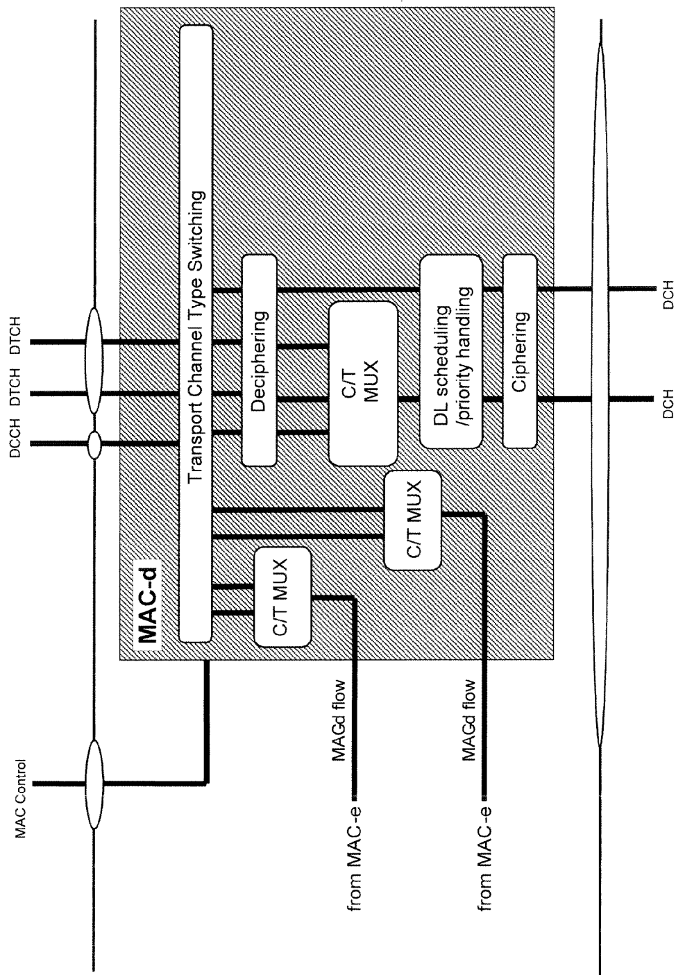
FIG. 9 RELATED ART
