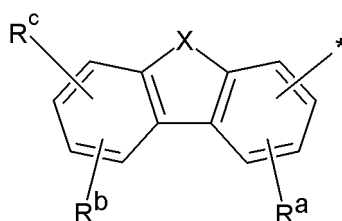
[Chemical Formula 2]
