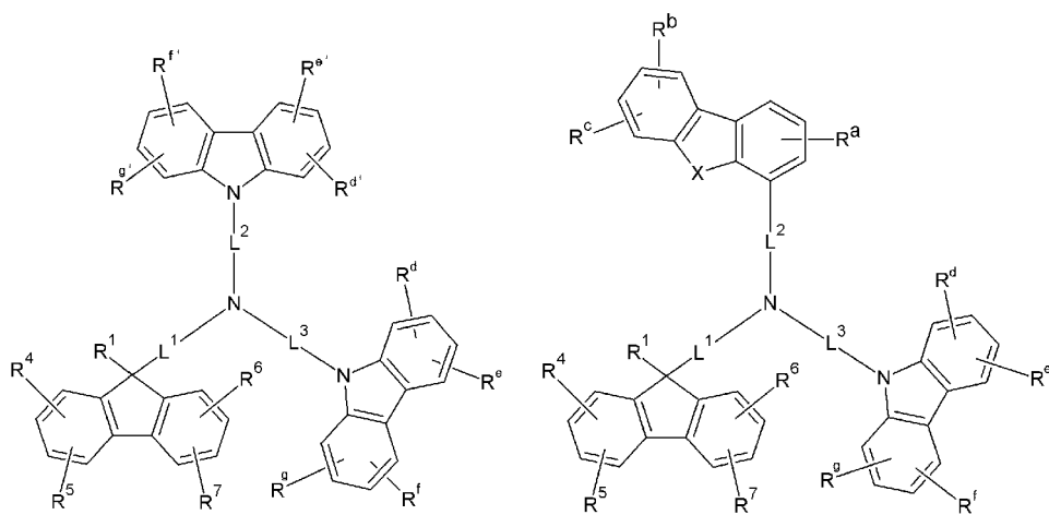
[Chemical Formula 12]
