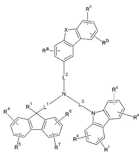
[Chemical Formula 12]
