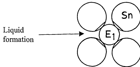
Stage I: solid state interdiffusion
