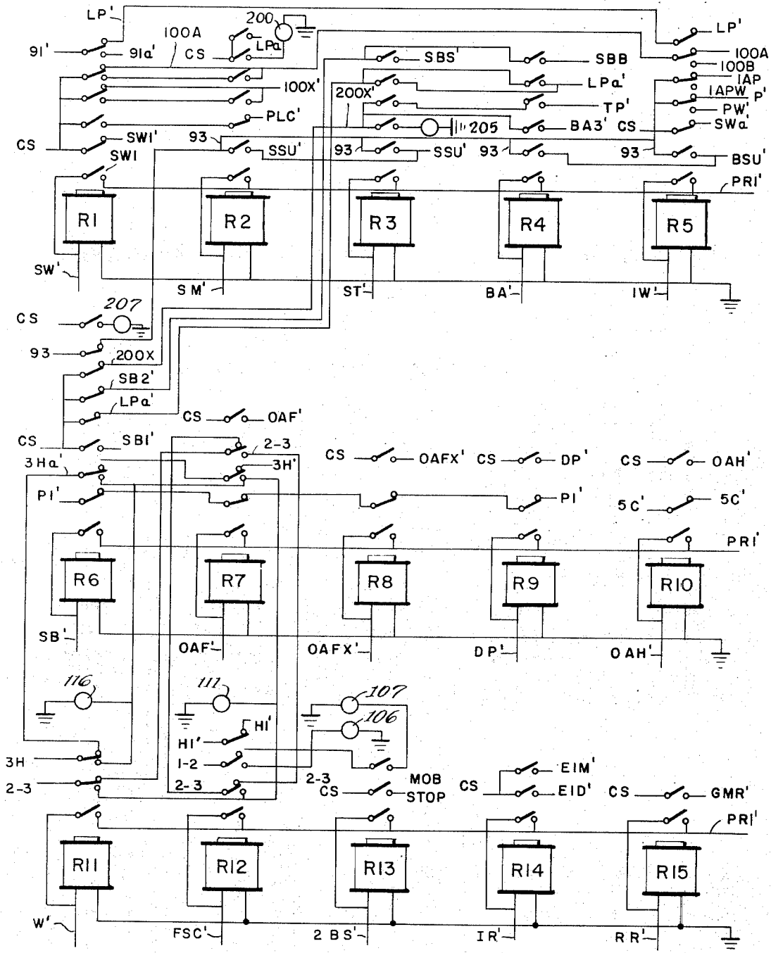
Fig. 7 PLAY CONTROL RELAYS-PCR
