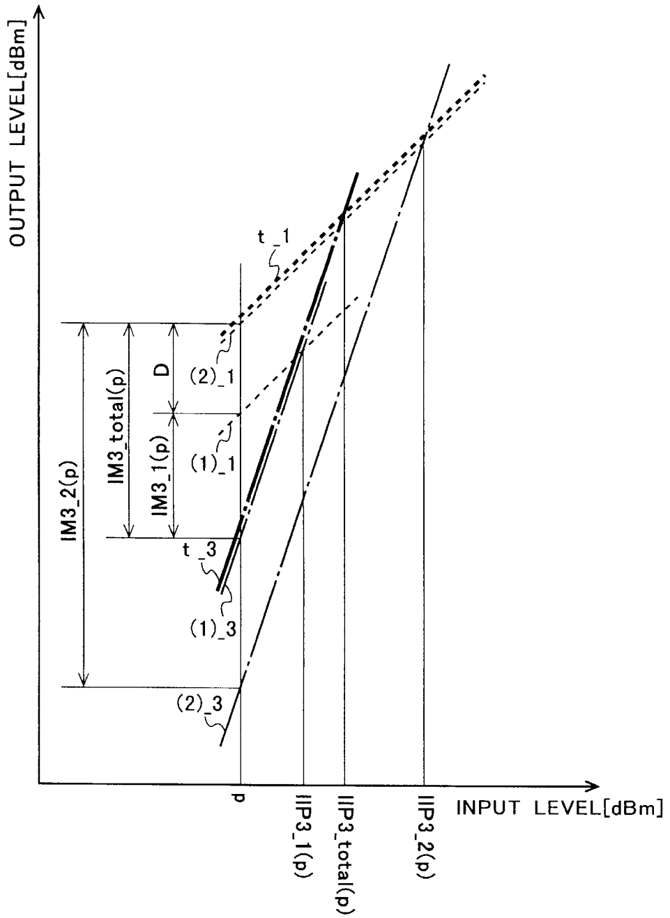
PRIOR ART Fig. 22
