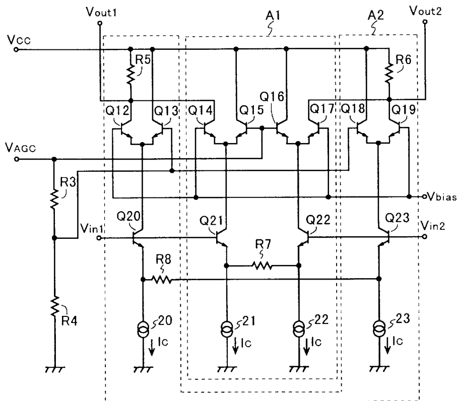
PRIOR ART Fig. 19
