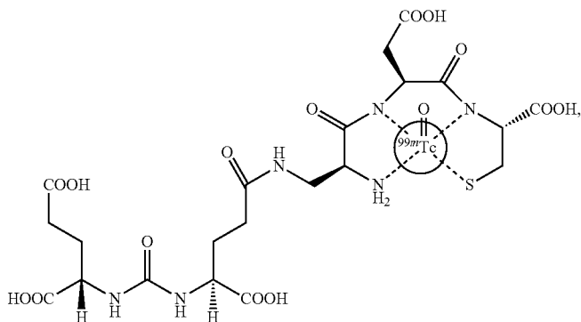
SK60- ^{99m}\text{Tc} (0-atom linker, 1.0 mg)
