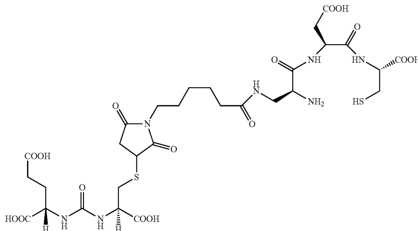
(9-atom linker)
