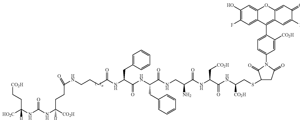
SK49 (25 Atom Linker-Oregon Green 488, C 71 H 76 F 2 N 10 O 24 , Mol. Wt.: 1523.48)
