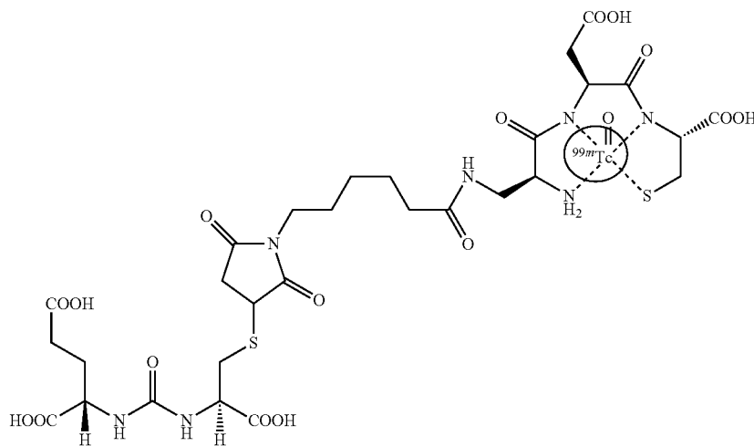
(9-atom linker)
