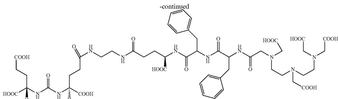
DTPA conjugate capable of chelating for example In, Ga, Ir, Yr, and the like
