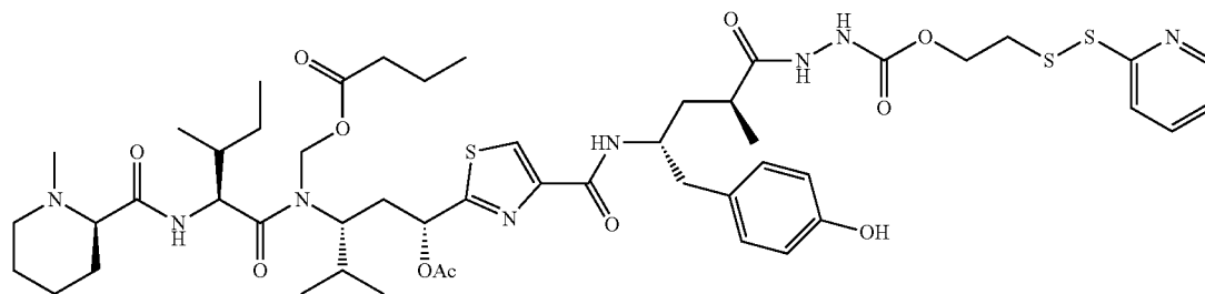
EC0312 C_{50}H_{72}N_8O_{11}S_3 Mol. Wt.: 1057.35
