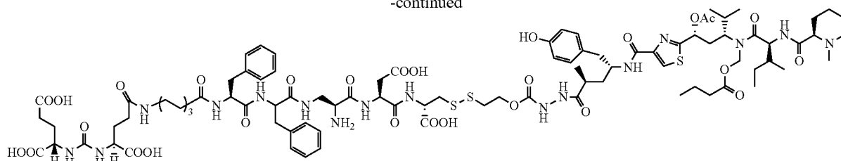
PC01SK77 C_{93}H_{133}N_{16}O_{28}S_3 Mol. Wt.: 2006.32
