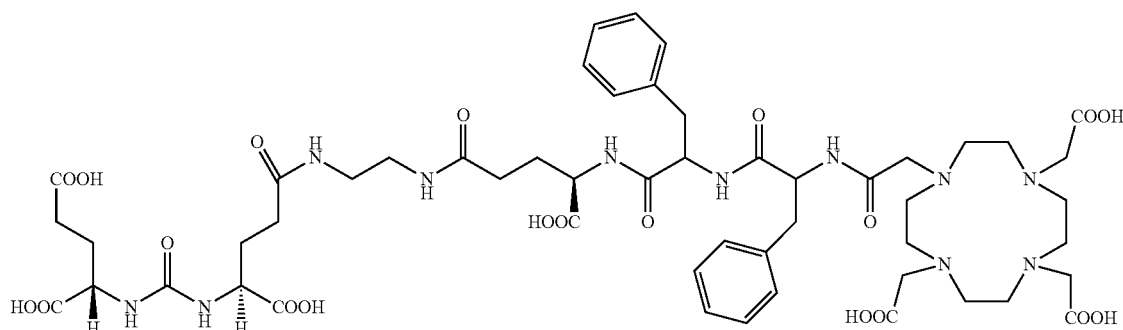
DOTA conjugate capable of chelating for example ^{64}\text{Cu} , ^{65}\text{Cu} , and the like
