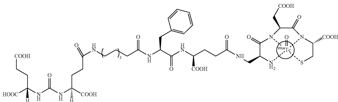
SK38- ^{99m}\text{Tc} (16-atom linker, 1.4 mg)
