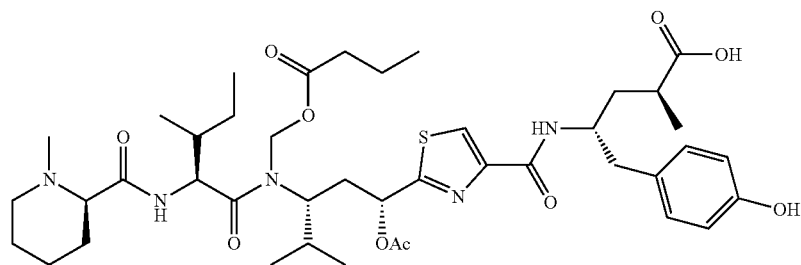
Tubulysin B C_{42}H_{63}N_5O_{10}S Mol. Wt.: 830.44
