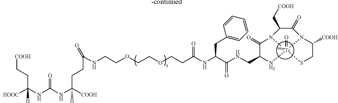
SK57- 99m Tc (24-atom linker, 1.8 mg)
