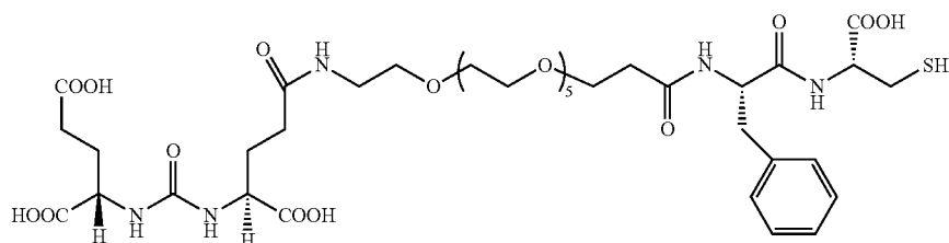
PC01SK54 C_{38}H_{59}N_5O_{18}S Mol. Wt.: 905.96
