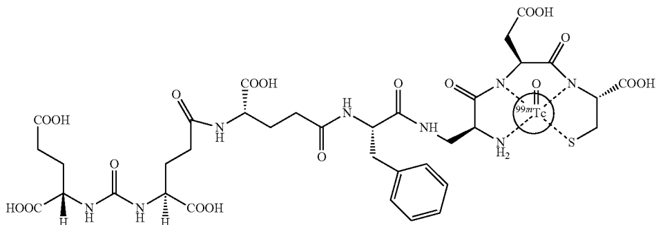
SK62- ^{99m}\text{Tc} (7-atom linker, 1.0 mg)
