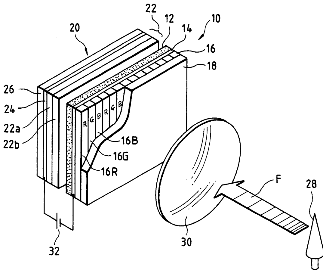
FIG. 8 PRIOR ART
