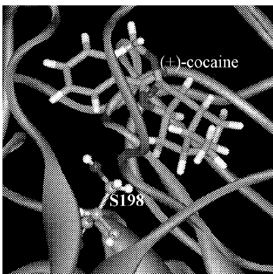
(C) BChE-(+)-cocaine non-prereactive complex
