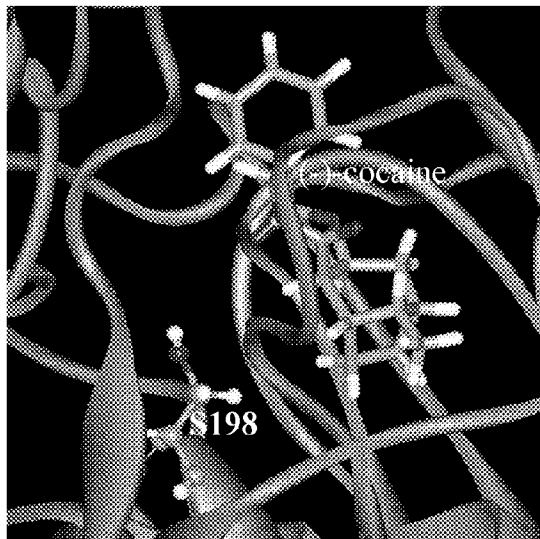
(A) BChE-(-)-cocaine non-prereactive complex
