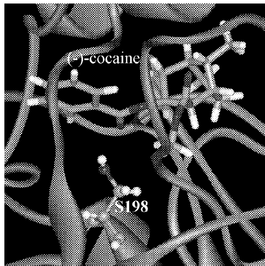
(B) BChE-(-)-cocaine prereactive complex
