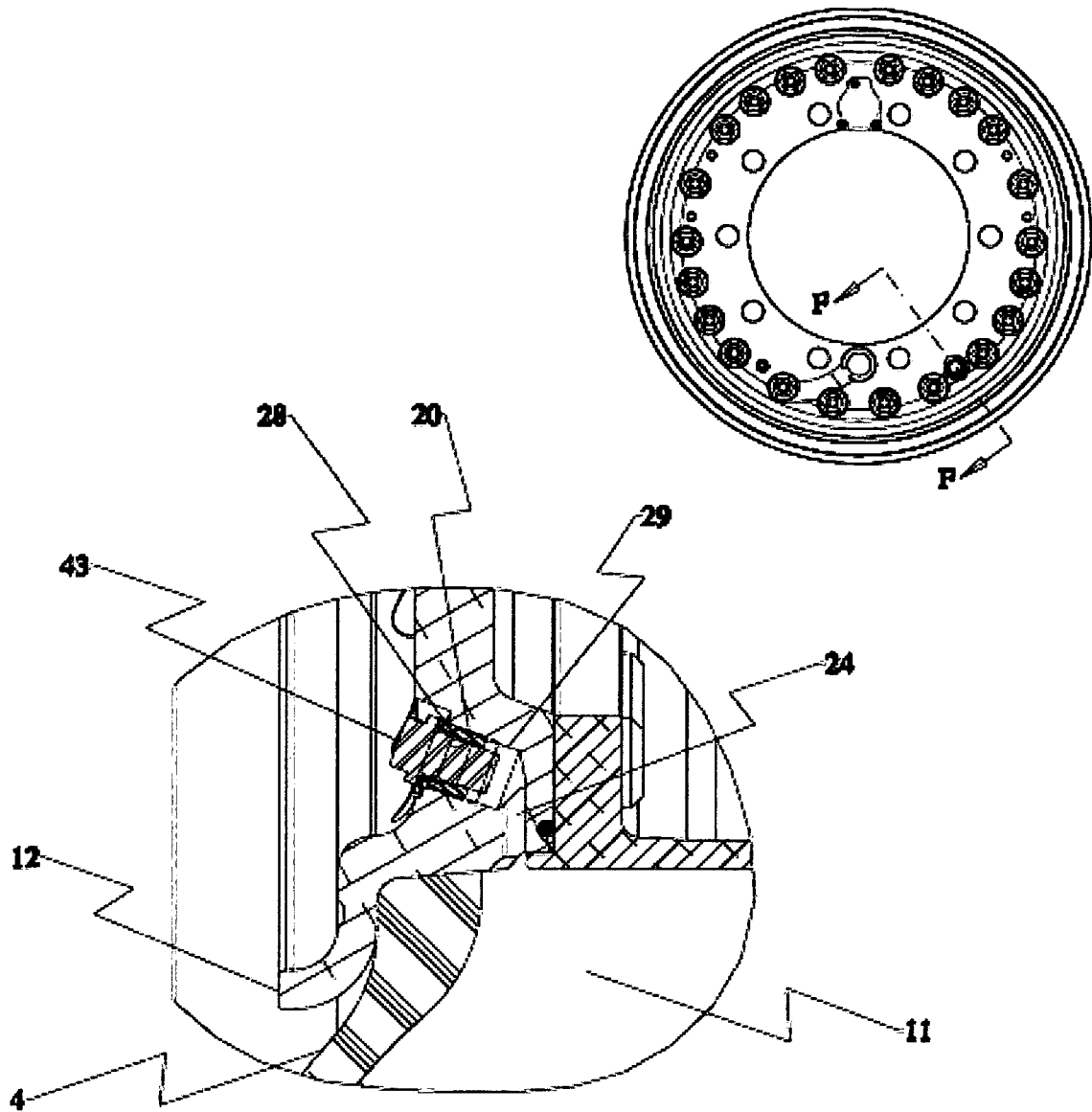
FIG. 7 (SECTION F-F)
