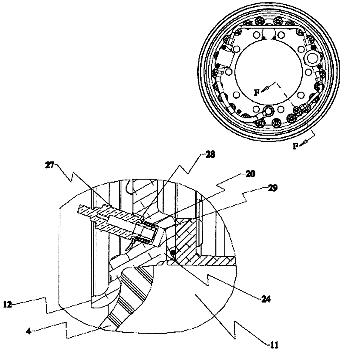
FIG. 4 (SECTION F-F)
