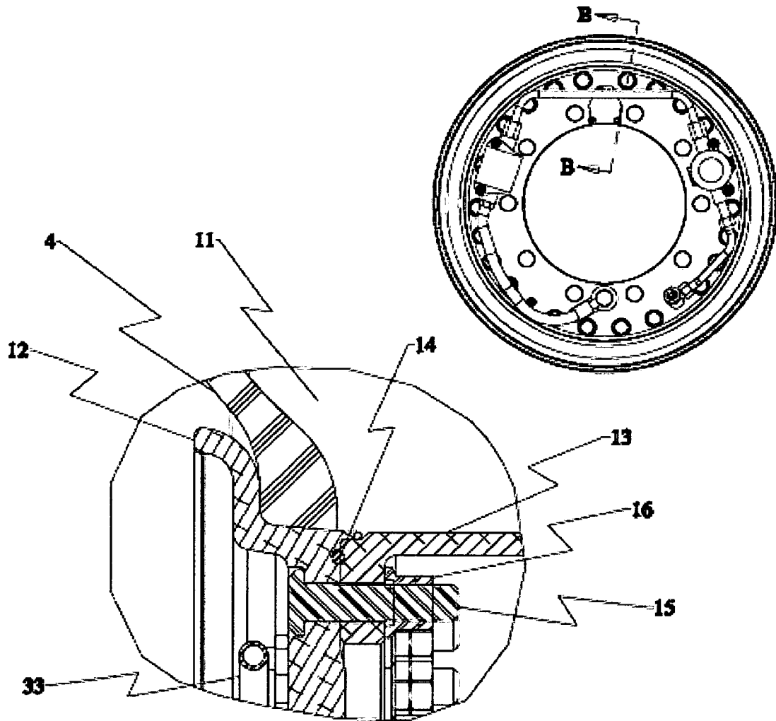
FIG. 9 (SECTION B-B)
