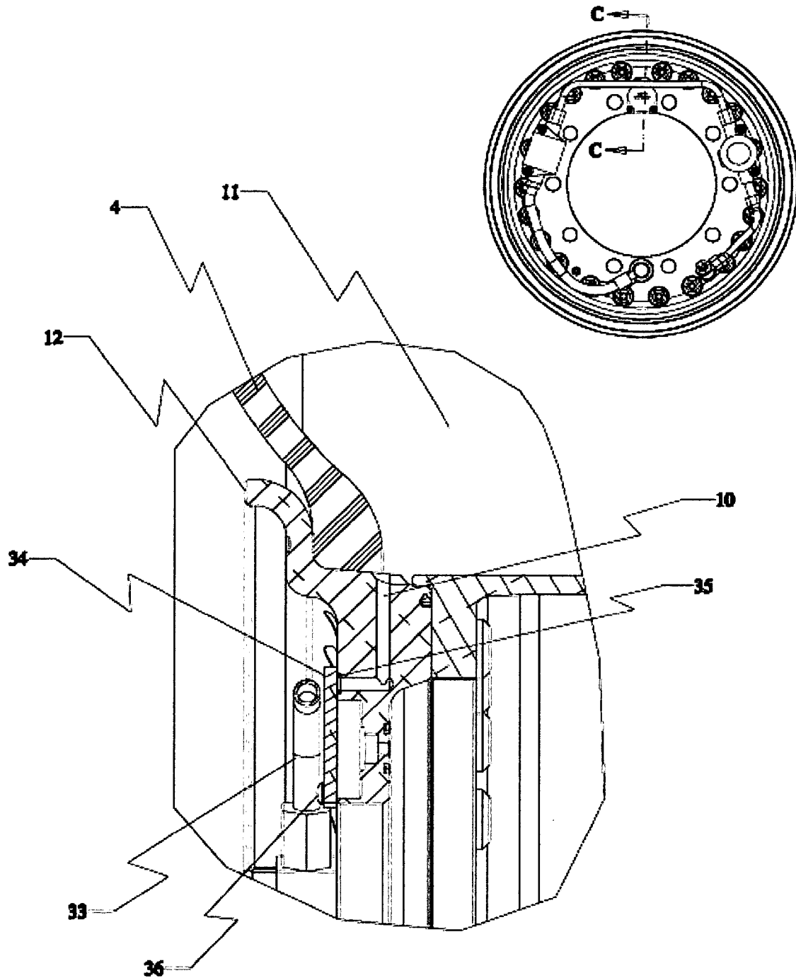
FIG. 3 (SECTION C-C)
