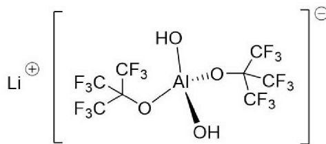
\text{Li[Al(OH)}_2\text{(OC(CF}_3)_3)_2] Compound X4
