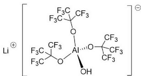
\text{Li[Al(OC(CF}_3)_3)_3\text{(OH)]} Compound X3
