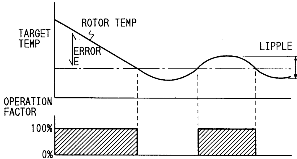
FIG. 9 PRIOR ART
