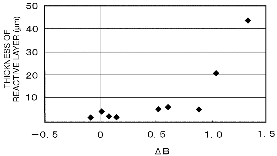
RELATIONSHIP BETWEEN \Delta B AND THICKNESS OF REACTIVE LAYER
