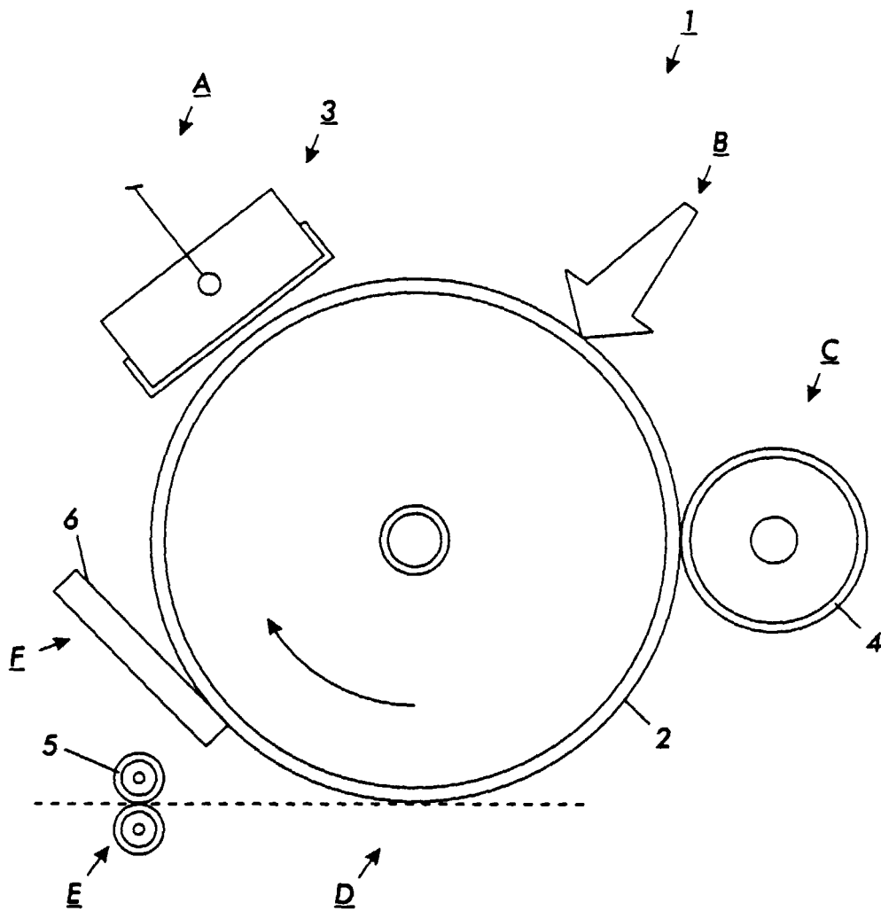
FIG. 2 PRIOR ART
