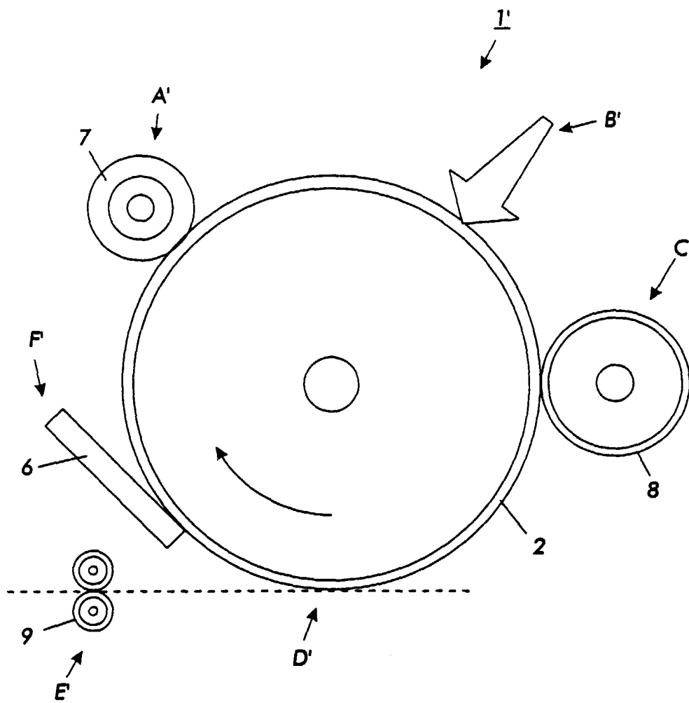
FIG. 3 PRIOR ART
