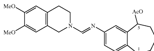
Acetic acid 7-[(3,4-dihydro-1H-isoquinolin-2-ylmethylene)-amino]-1,2,3,4-tetrahydronaphthalen-1-yl ester
