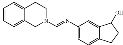
6-[(3,4-dihydro-1H-isoquinolin-2-ylmethylene)-amino]-indan-1-ol
