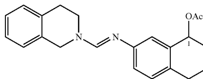
Acetic acid 7-[(3,4-dihydro-1H-isoquinolin-2-ylmethylene)-amino]-1,2,3,4-tetrahydronaphthalen-1-yl ester
