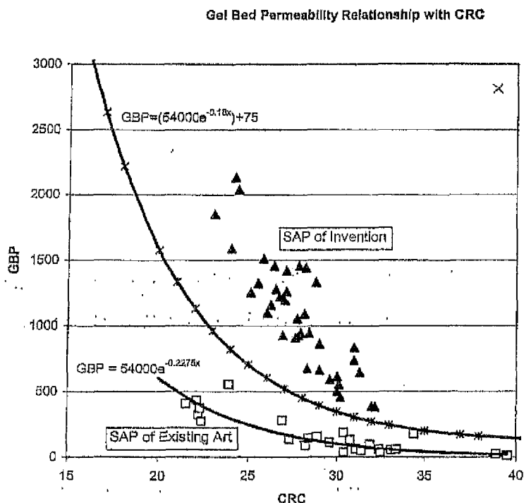
Graph 1. Relationship of Gel Bed Permeability I and Centrifuge Retention Capacity.
