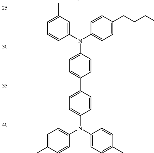
N-(4-Butyl-phenyl)-N-m-tolyl-N',N'-di-p-tolyl-biphenyl-4,4'-diamine
