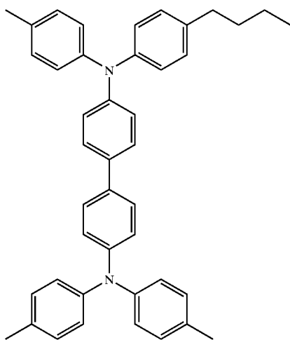
N-(4-Butyl-phenyl)-N,N',N'-tri-p-tolyl-biphenyl-4,4'-diamine
