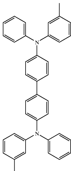
N,N'-Diphenyl-N,N'-di-m-tolyl-biphenyl-4,4'-diamine
