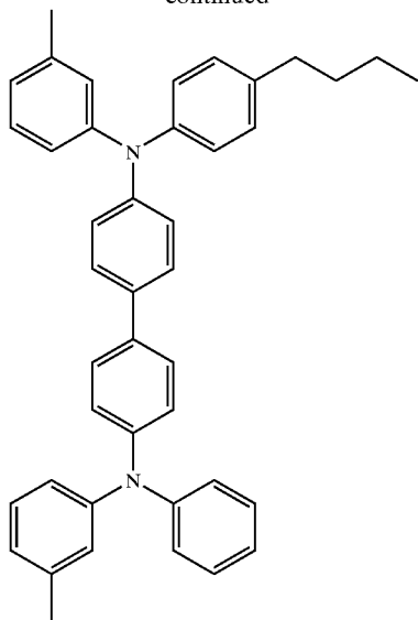
N-(4-Butyl-phenyl)-N'-phenyl- N,N'-di-m-tolyl-biphenyl-4,4'- diamine
