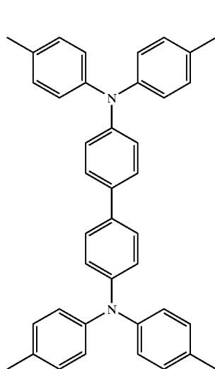
N,N,N',N'-Tetra-p-tolyl-biphenyl-4,4'-diamine
