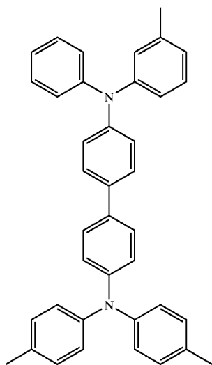
N-Phenyl-N-m-tolyl-N',N'-di-p-tolyl-biphenyl-4,4'-diamine
