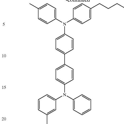
N-(4-Butyl-phenyl)-N'-phenyl-N'-m-tolyl-N-p-tolyl-biphenyl-4,4'-diamine
