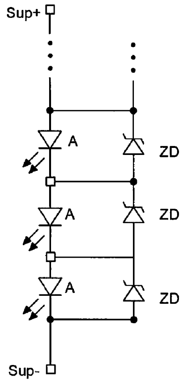
FIG. 1 (Prior Art)
