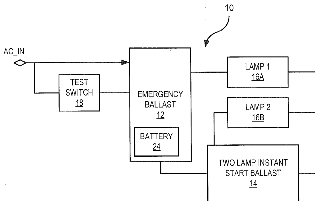
FIGURE 1 (PRIOR ART)
