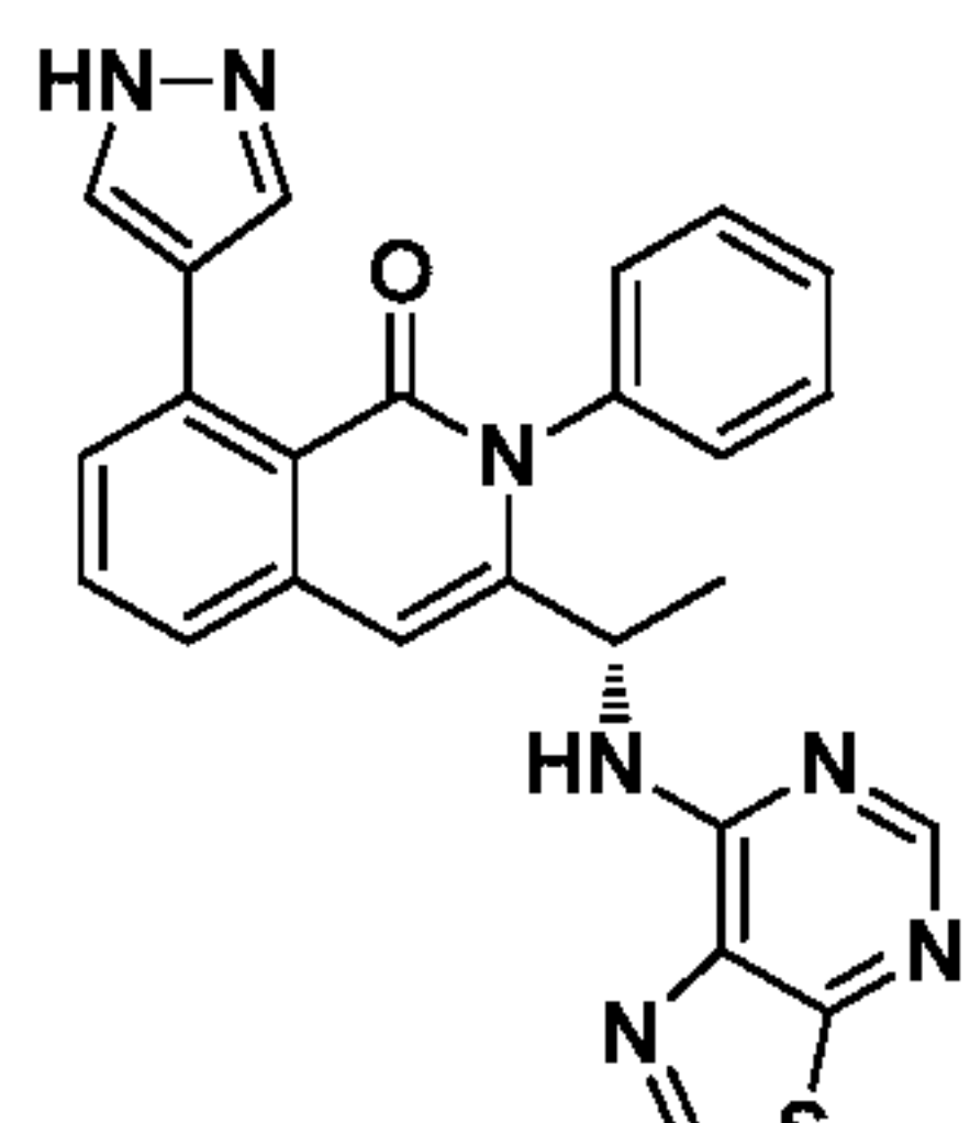
Compound 26,
