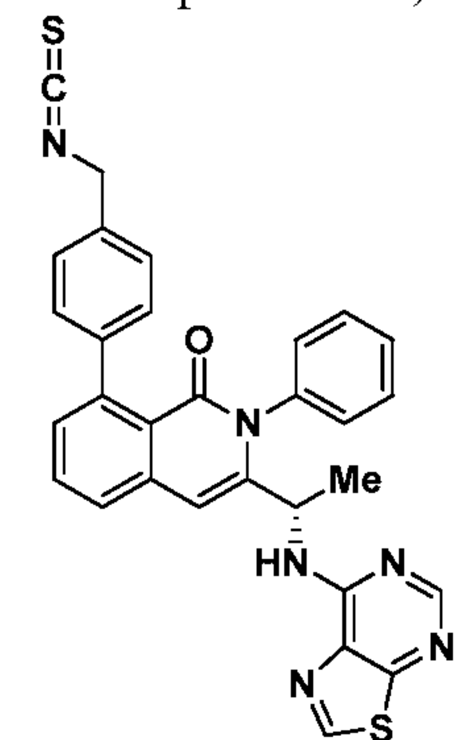
Compound 121,
