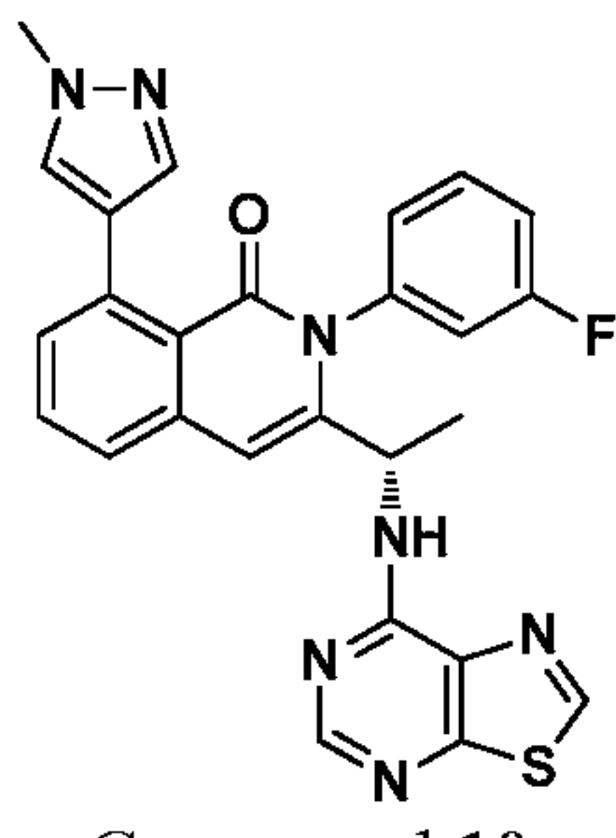
Compound 10,
