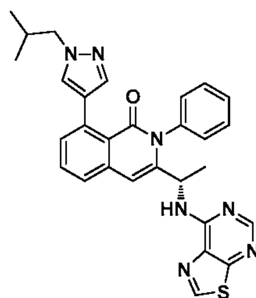
Compound 24,
