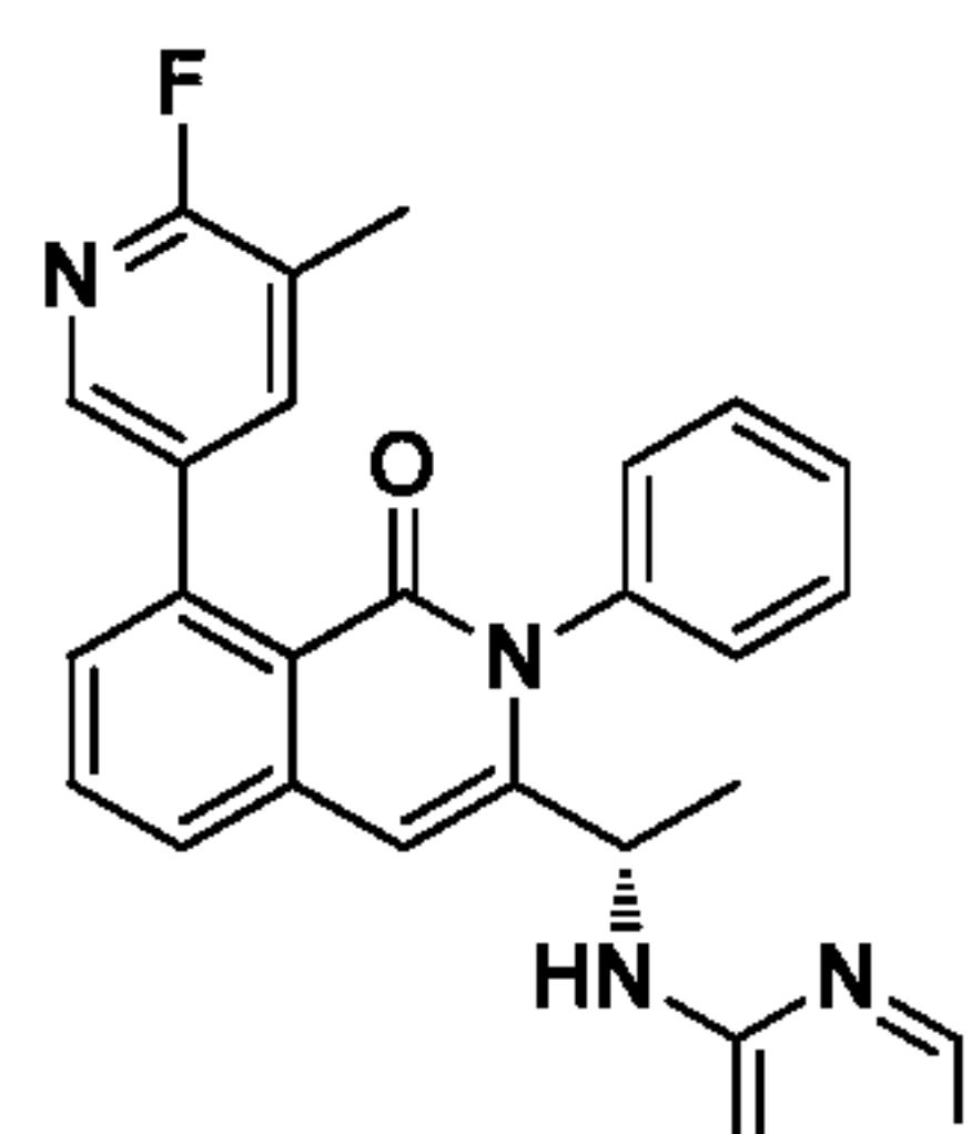
Compound 25,
