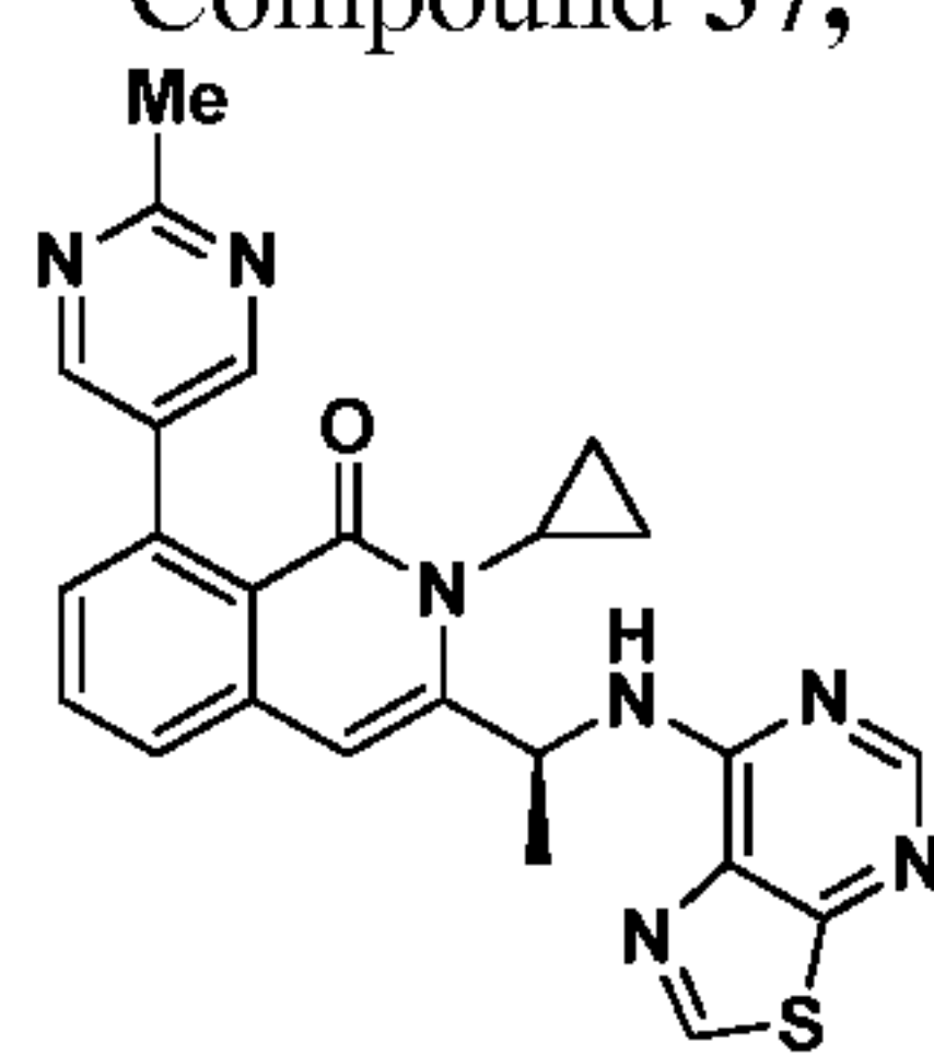
Compound 62,
