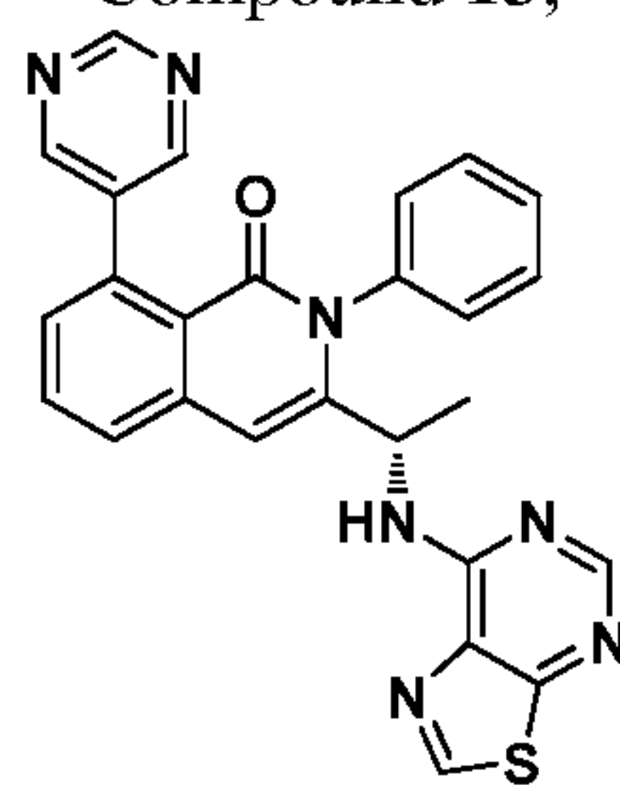
Compound 19,
