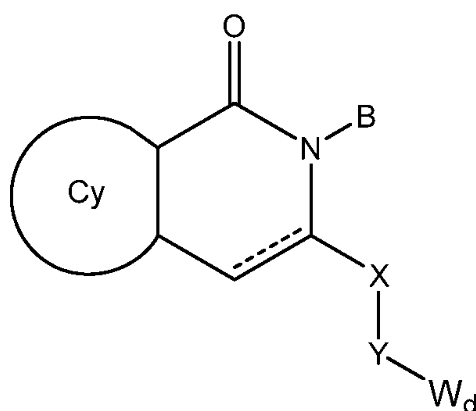
Formula (XIII)
