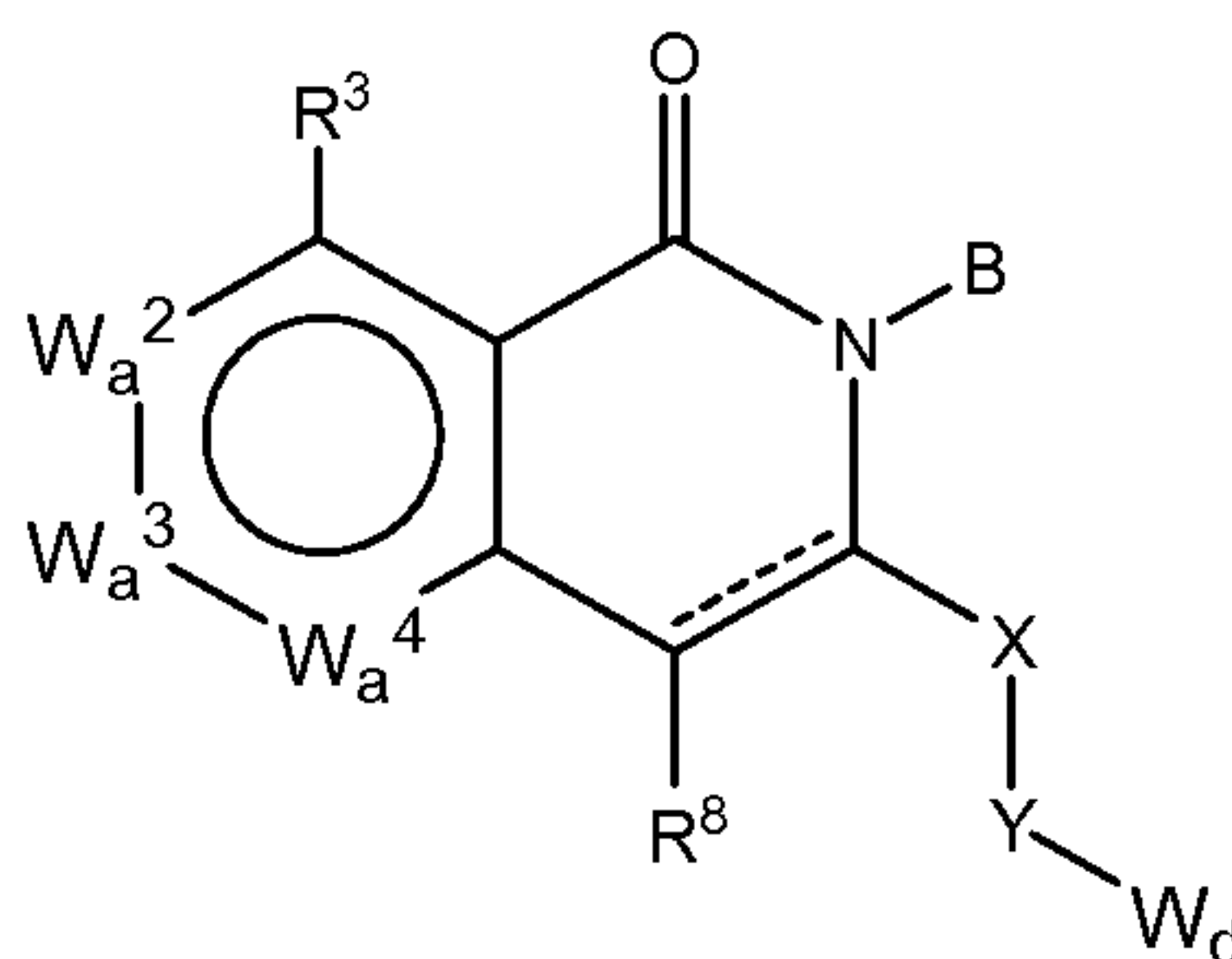
Formula (XV)
