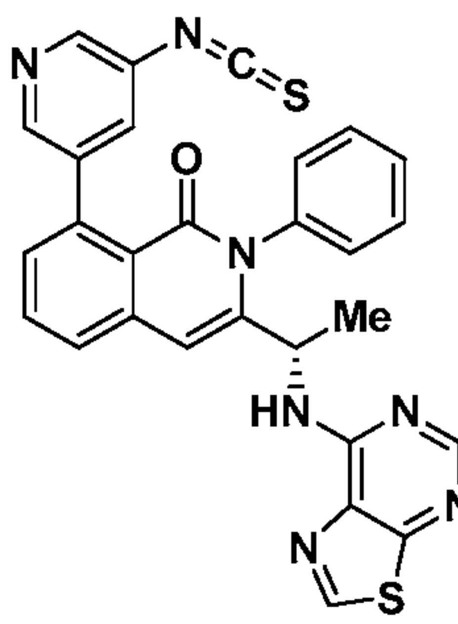
Compound 122,
