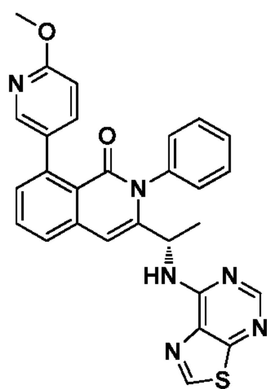
Compound 18,
