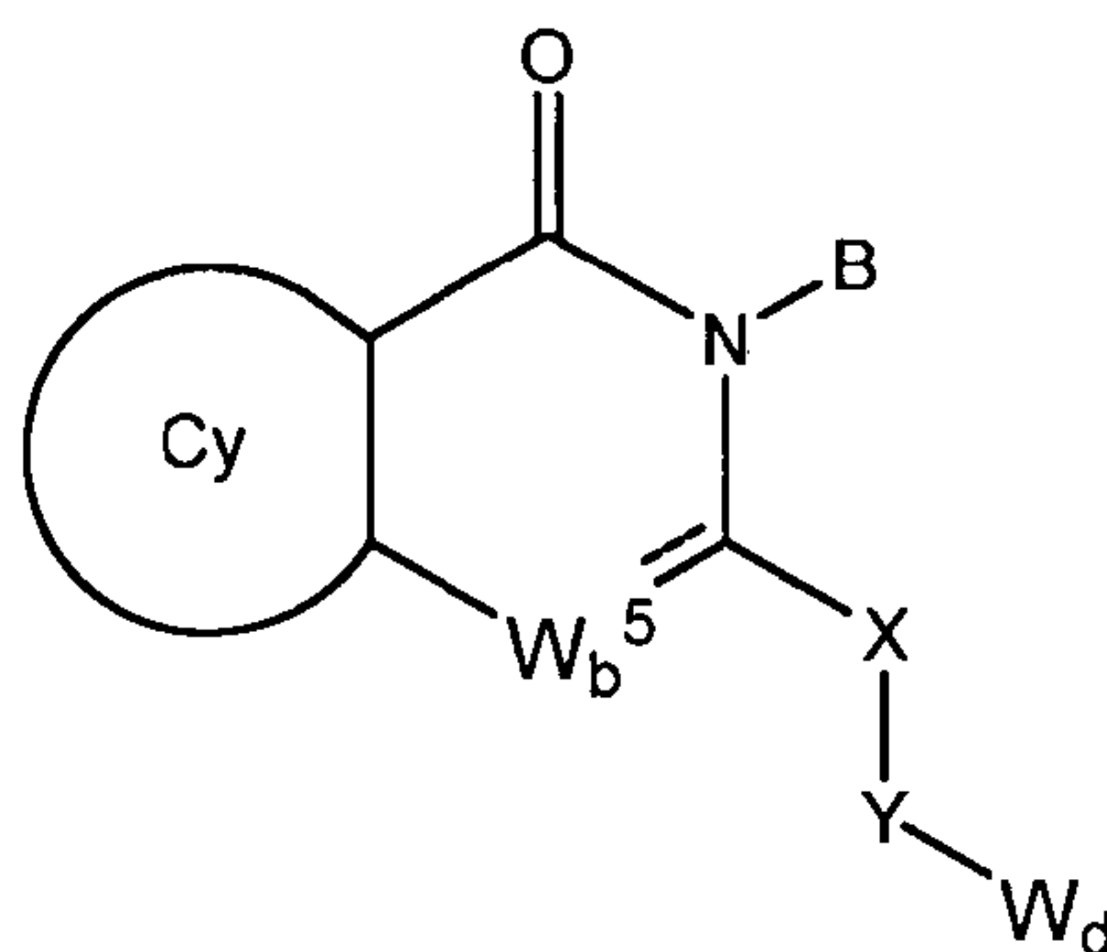
Formula (I)
