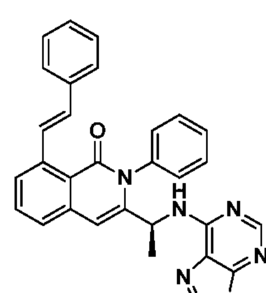
Compound 49,
