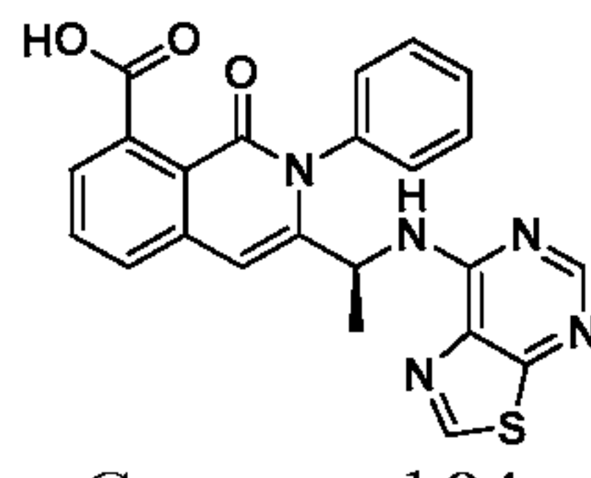
Compound 84,
