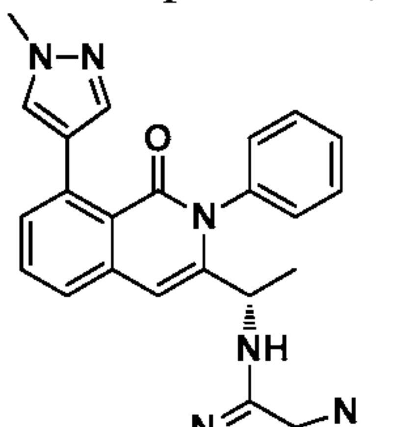
Compound 73,
