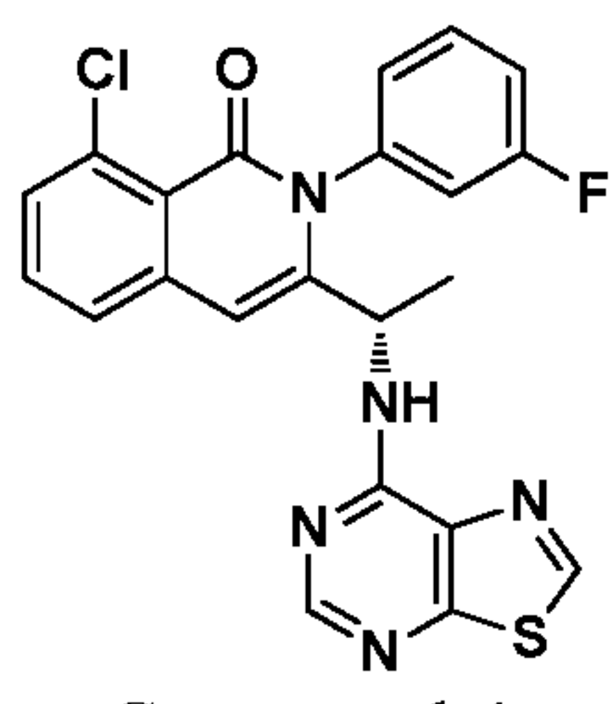
Compound 4,
