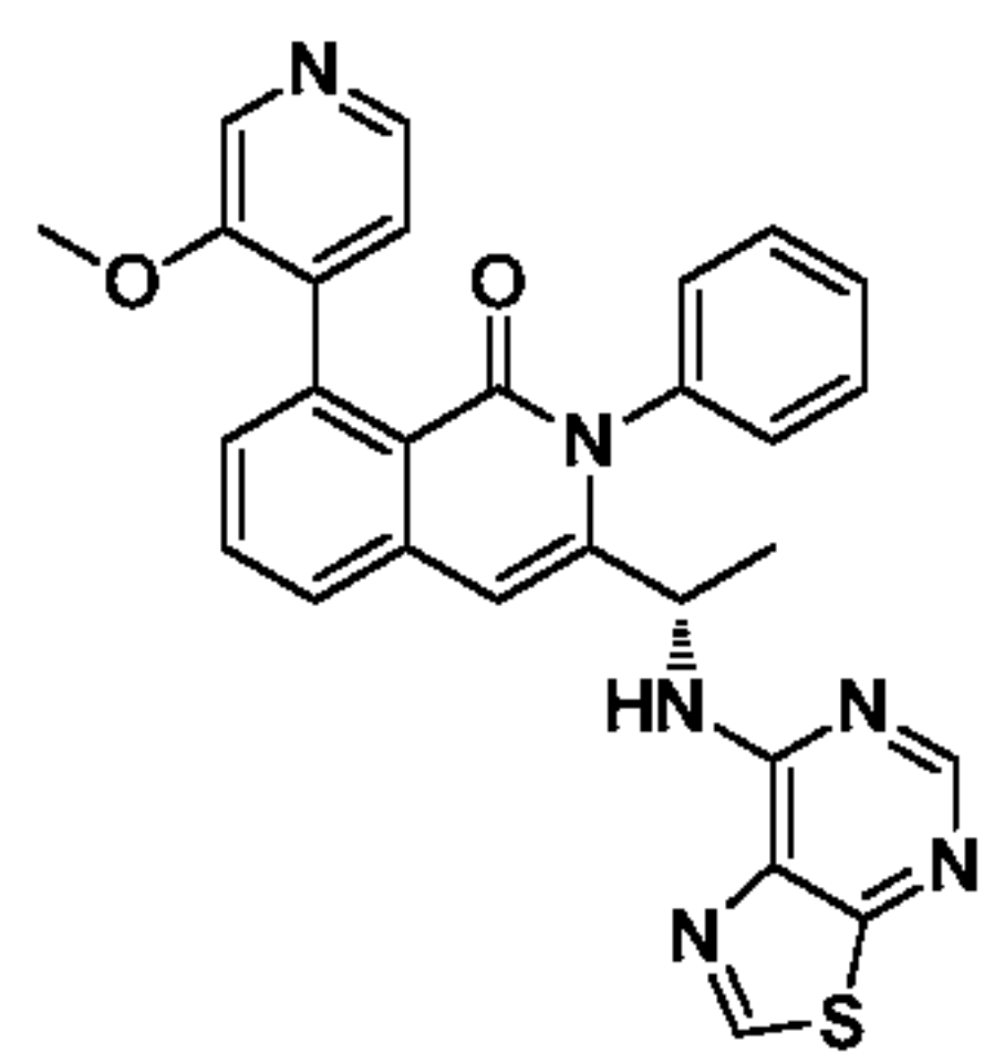
Compound 36,
