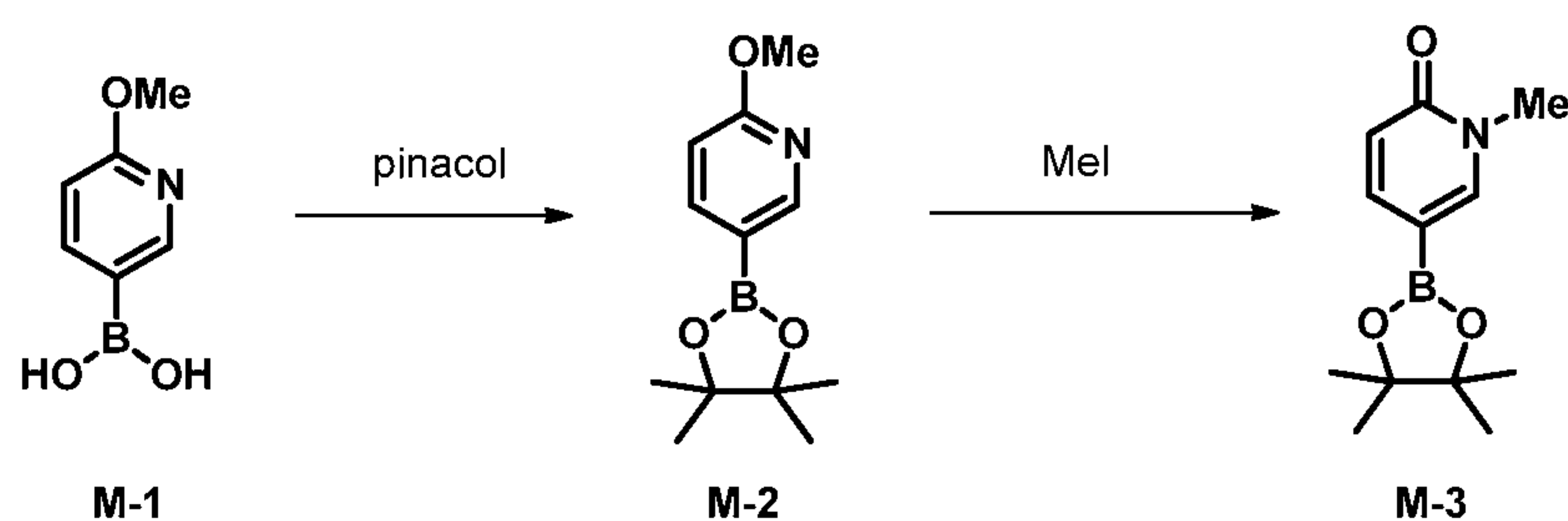
Method M:
