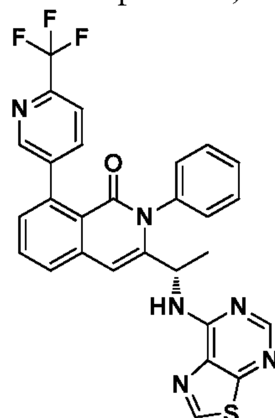
Compound 13,
