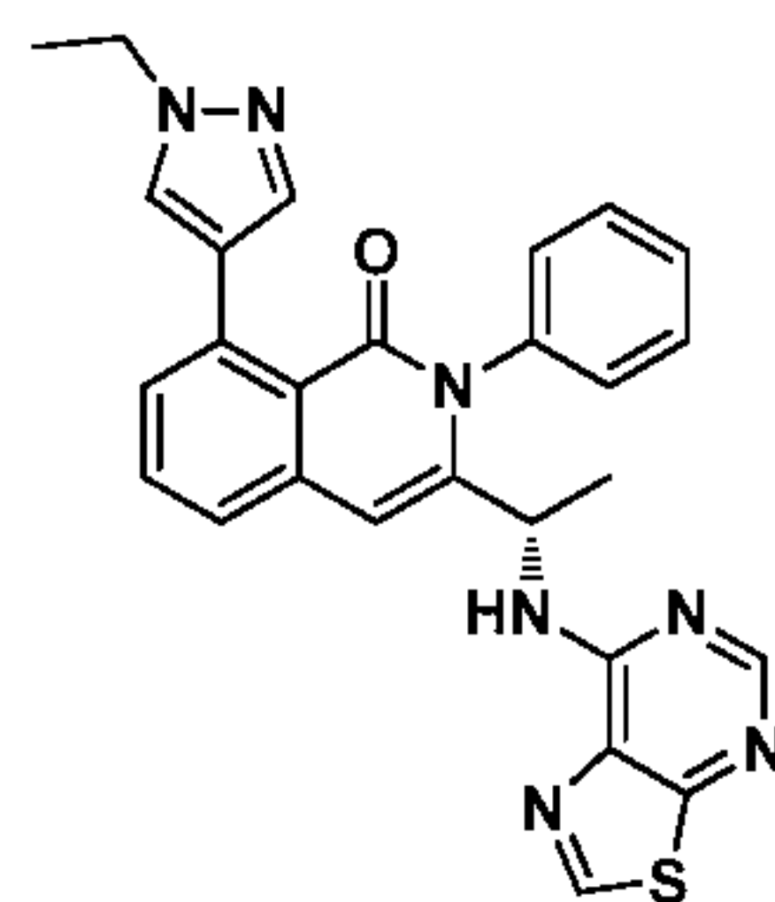
Compound 25,
