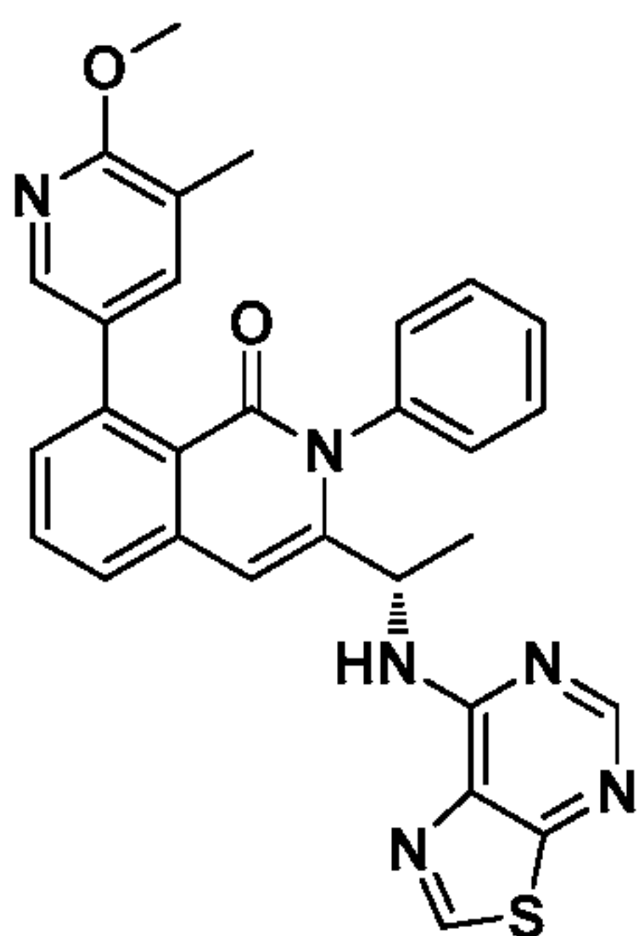
Compound 56,
