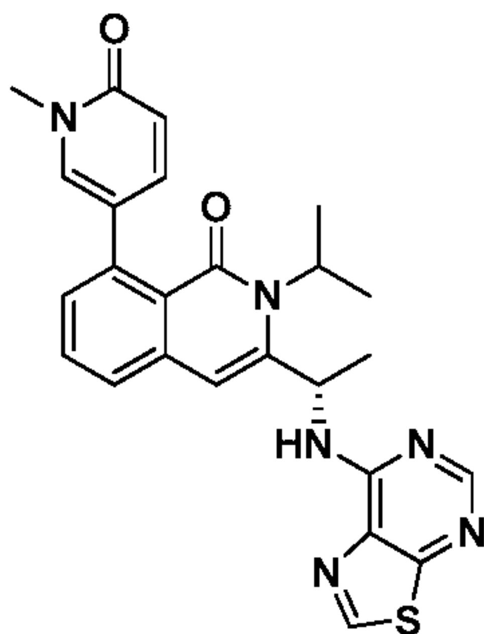
Compound 103,
