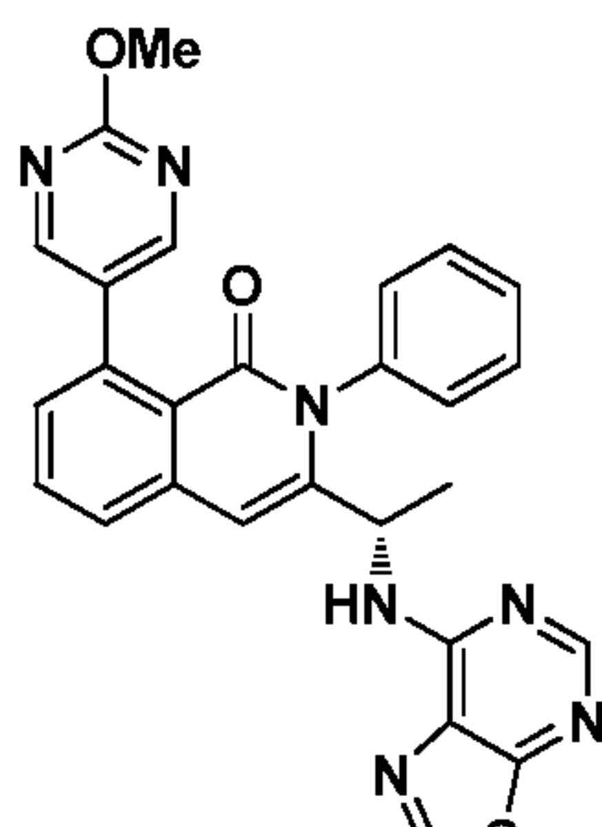
Compound 38,
