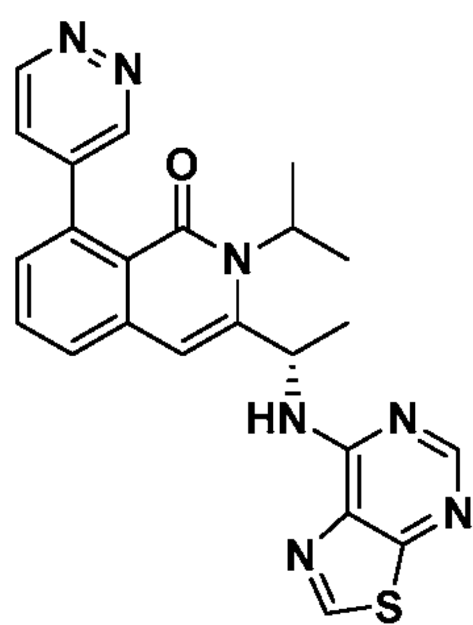
Compound 108,
