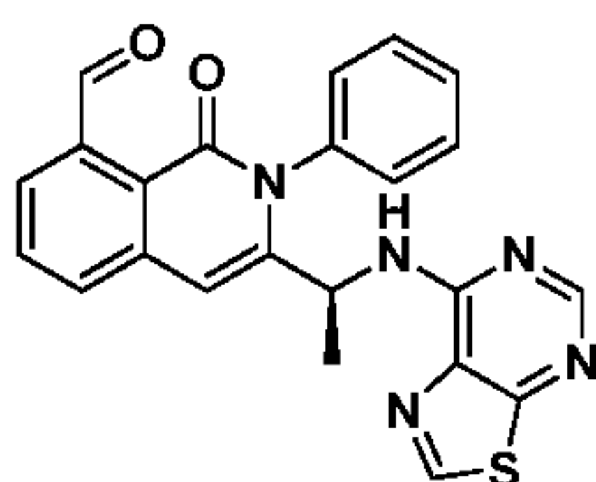
Compound 83,
