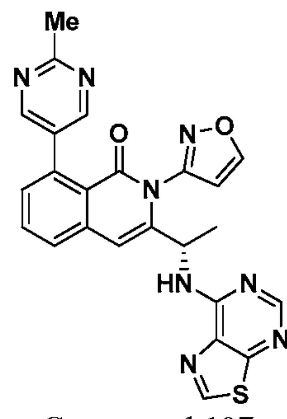
Compound 107,
