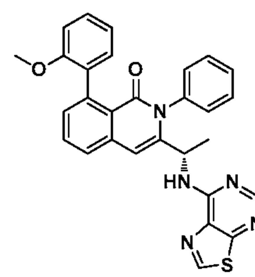
Compound 35,
