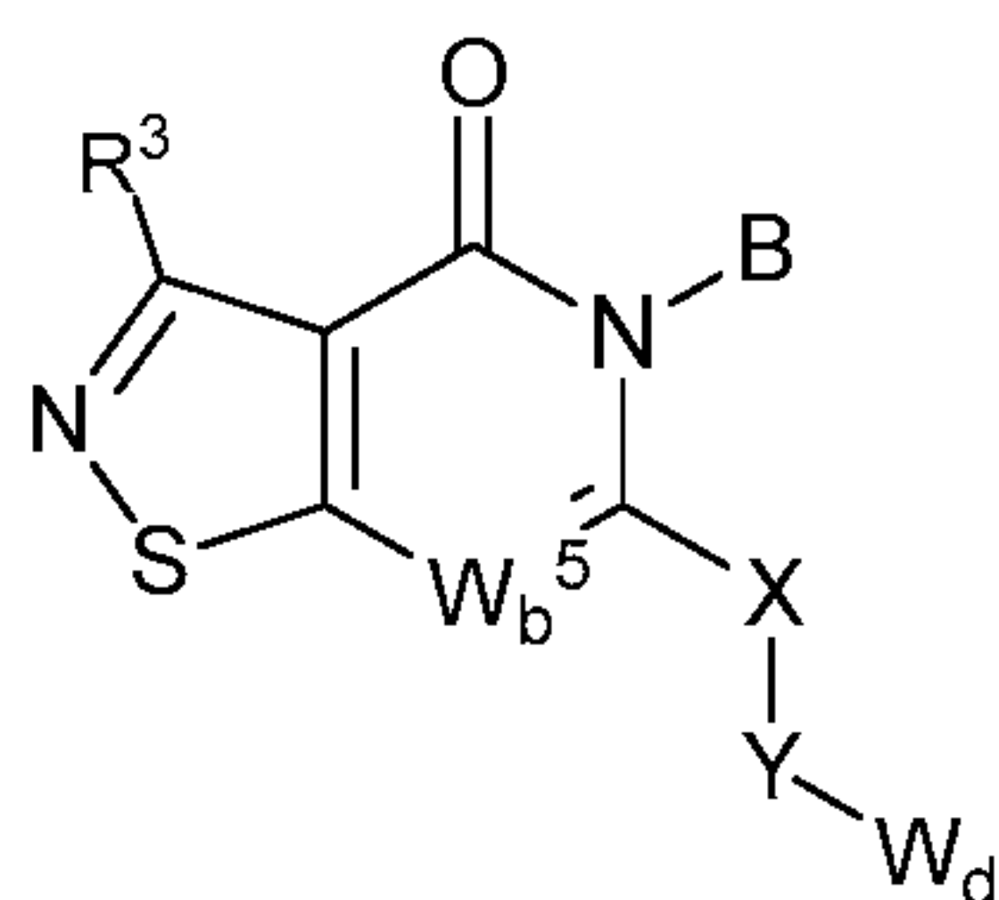
Formula (IVa)
