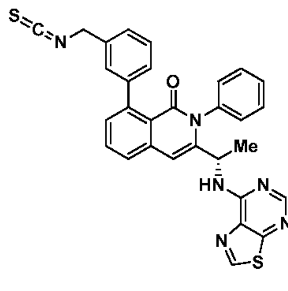
Compound 120,
