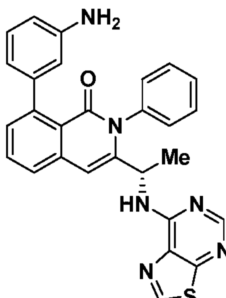
Compound 111,
