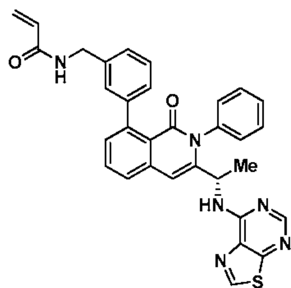
Compound 123 , or
