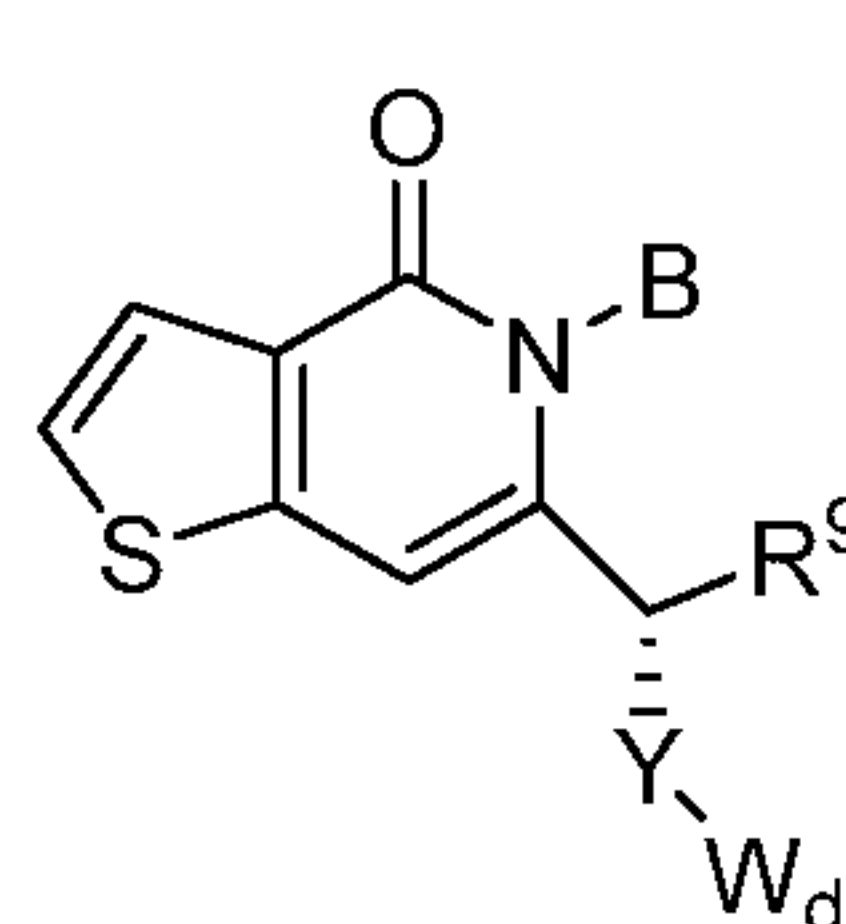
Formula (IXb).
