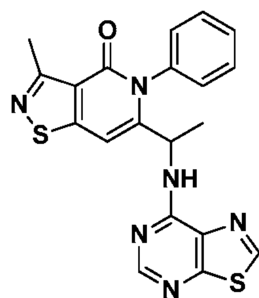
Compound 12,
