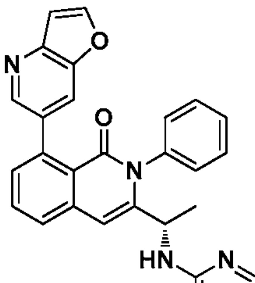
Compound 50,
