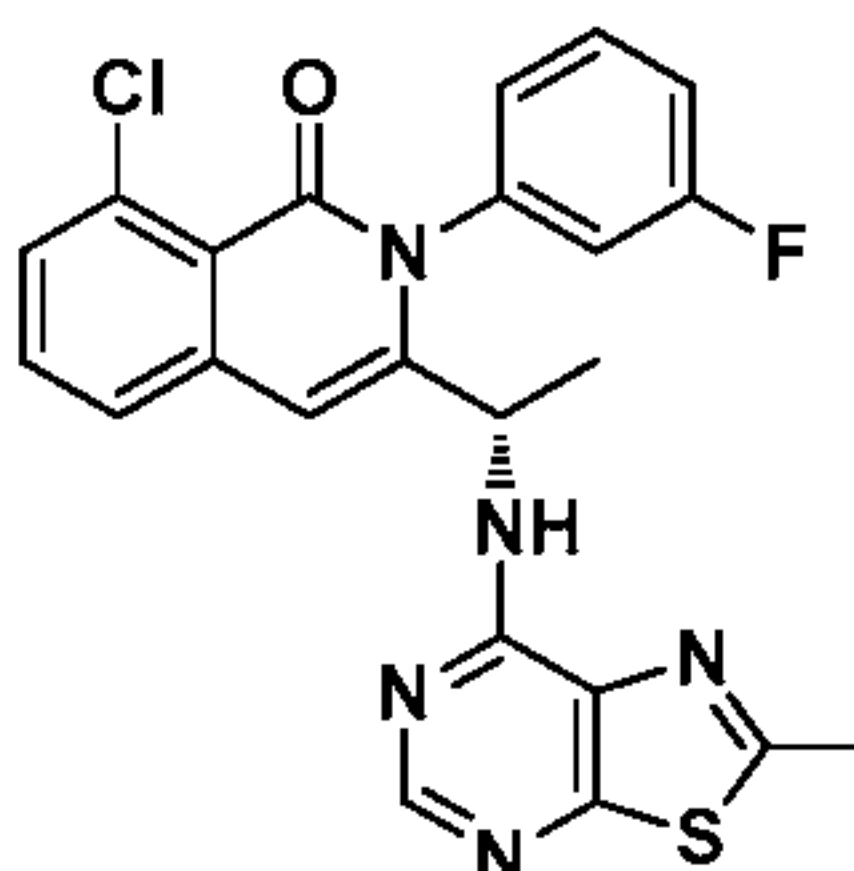
Compound 78,
