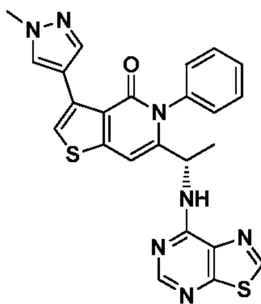
Compound 16, or
