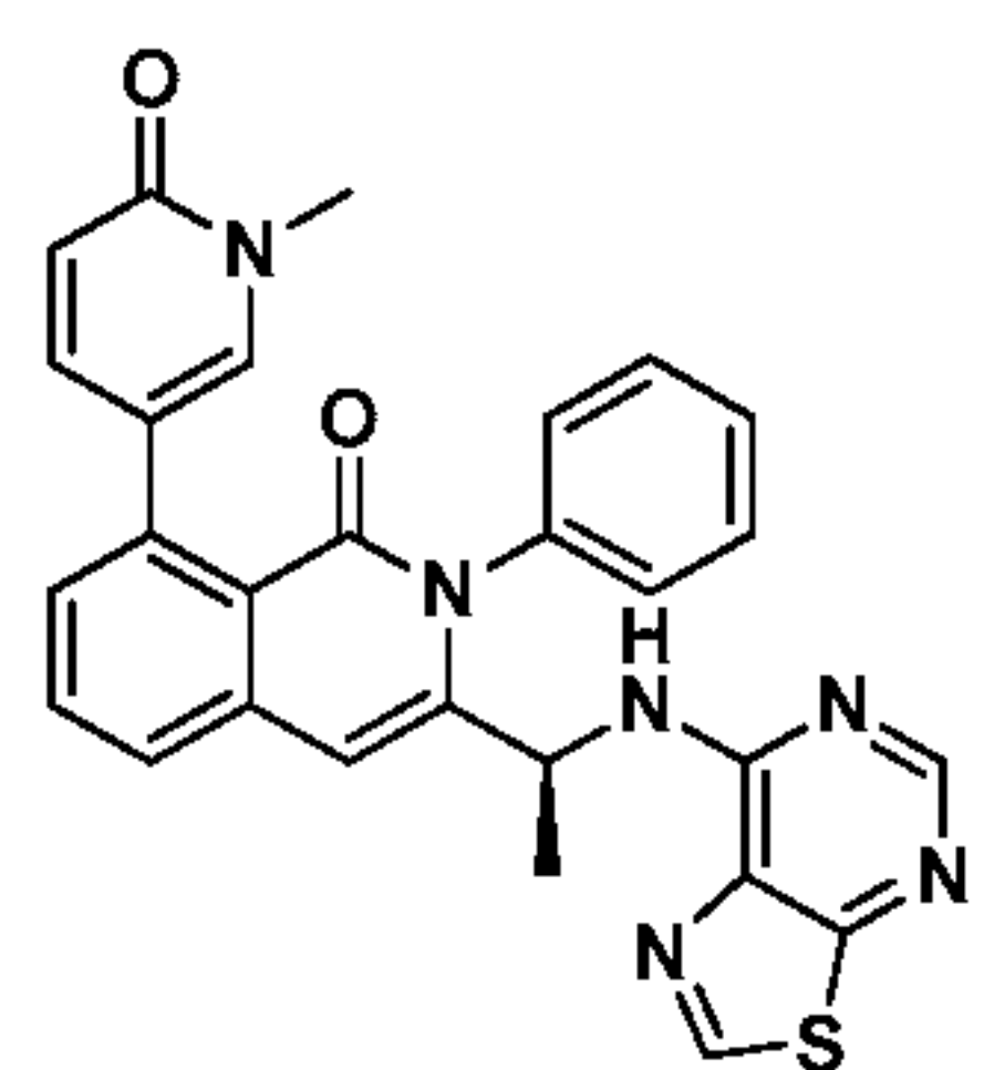
Compound 51,
