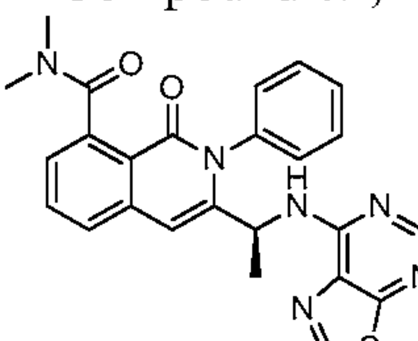
Compound 85,
