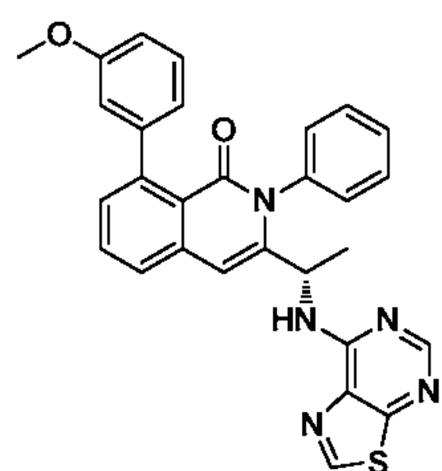
Compound 31,
