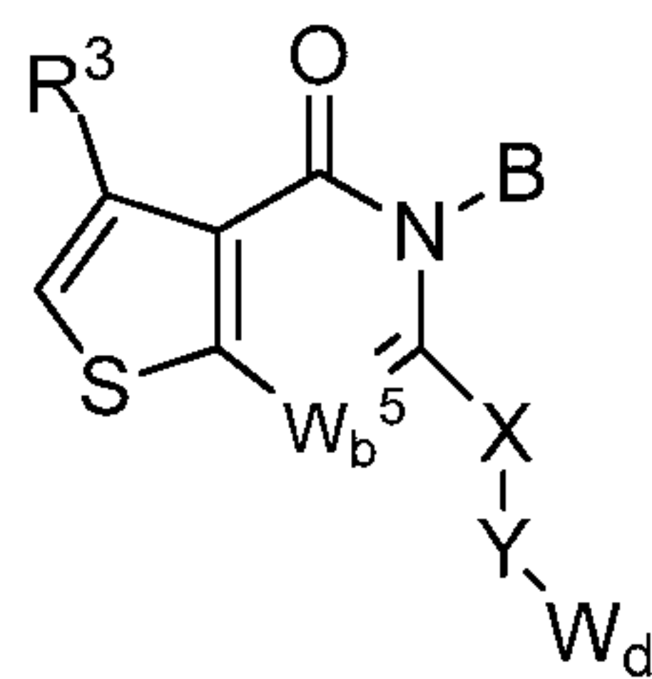
Formula (VIa)
