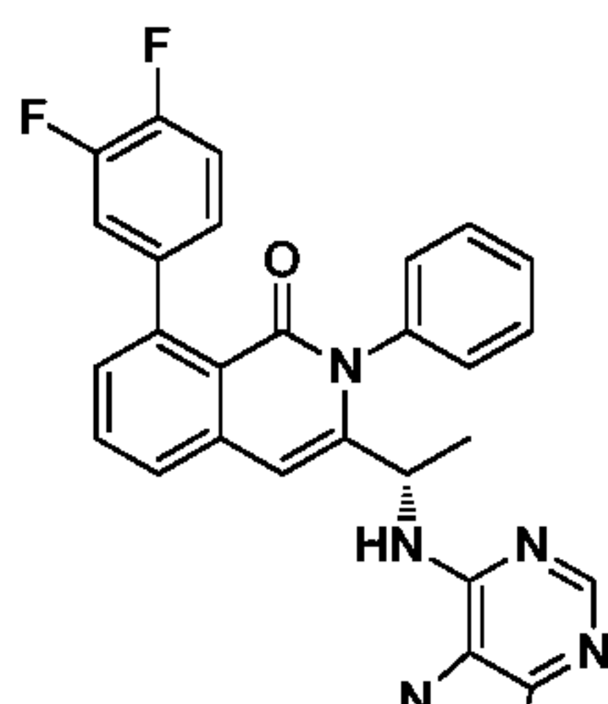
Compound 22,
