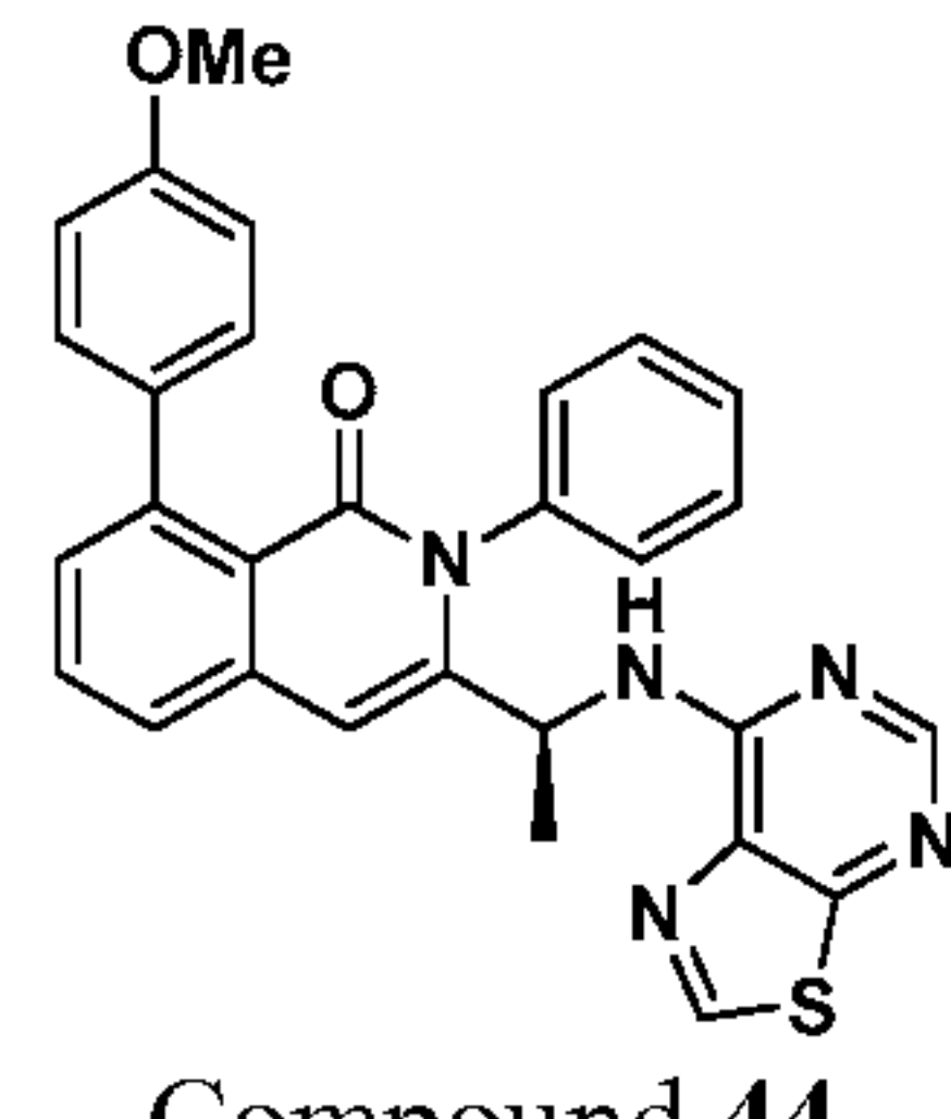
Compound 44,
