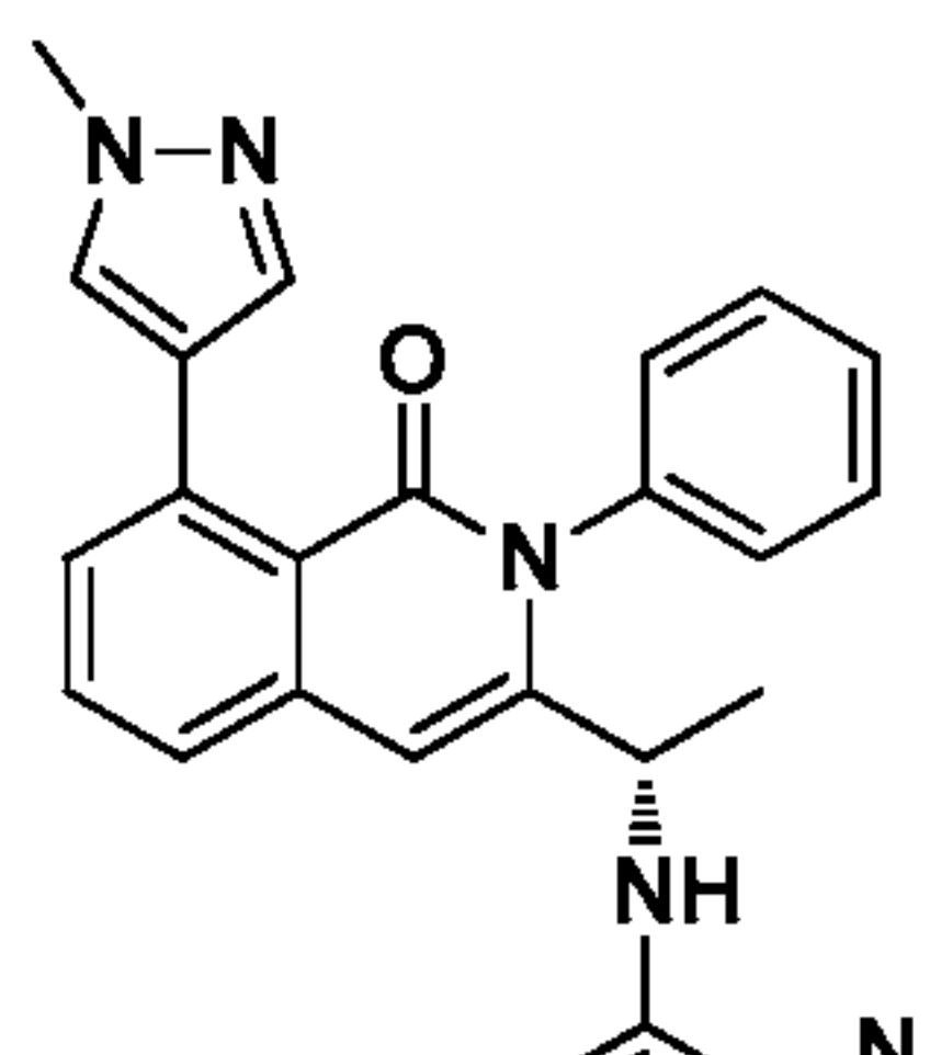
Compound 68,
