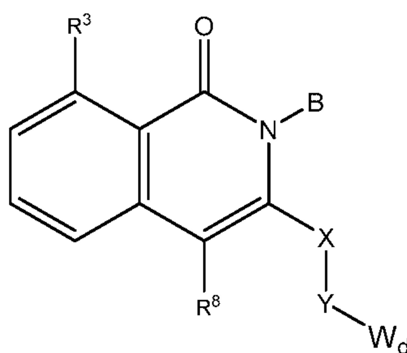
Formula (IIb).
