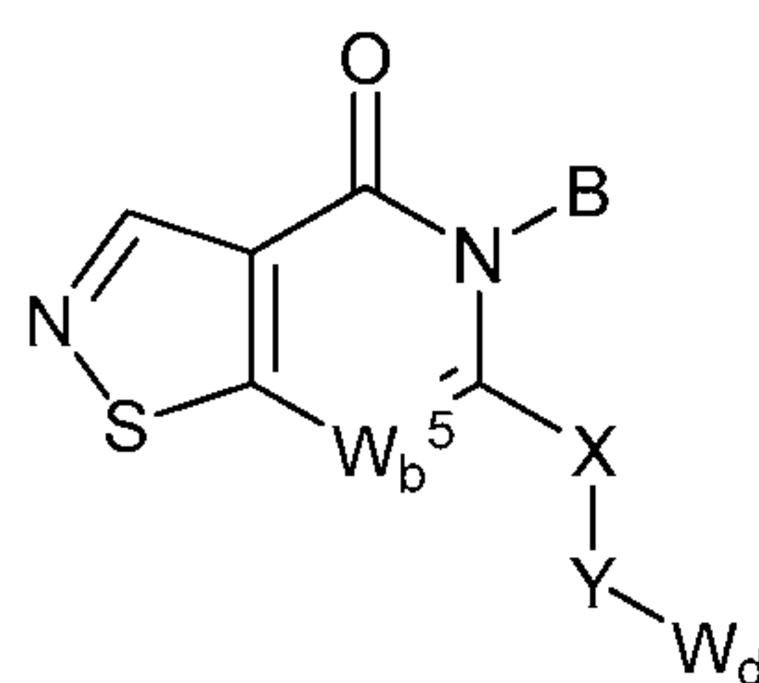
Formula (IVb).
