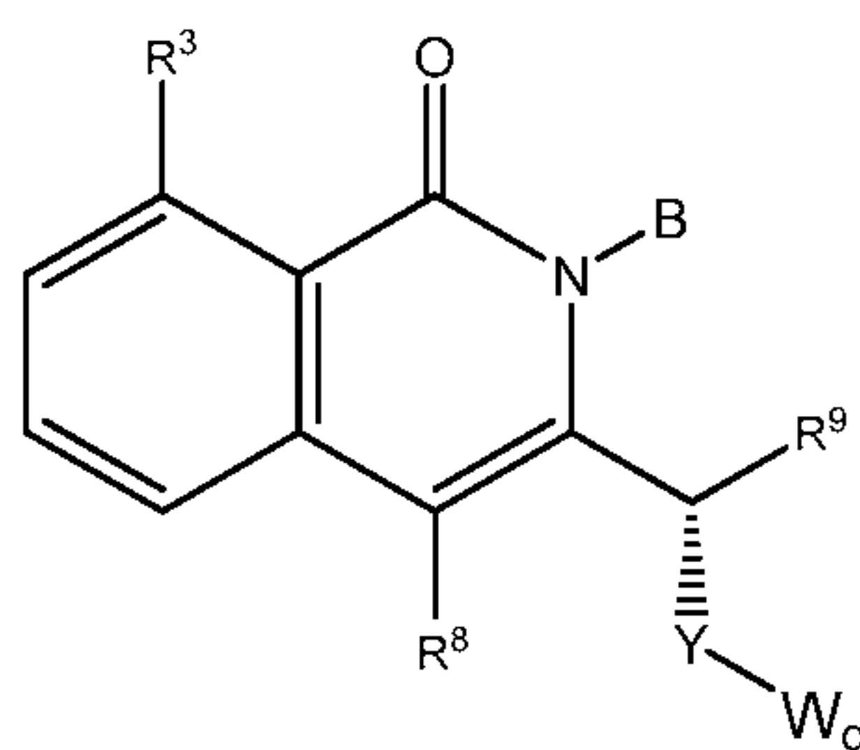
Formula (IIIb).
