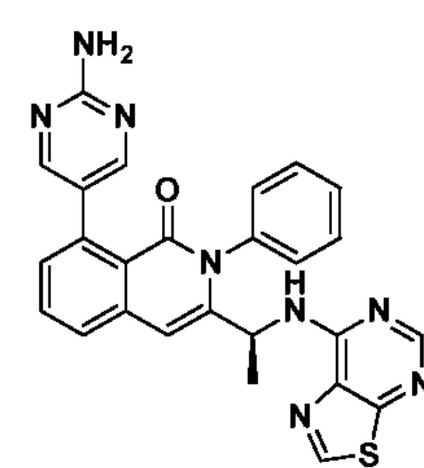
Compound 50,
