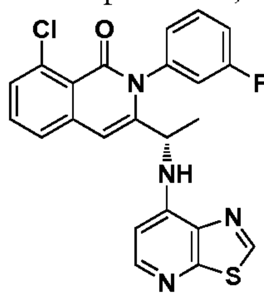
Compound 90,
