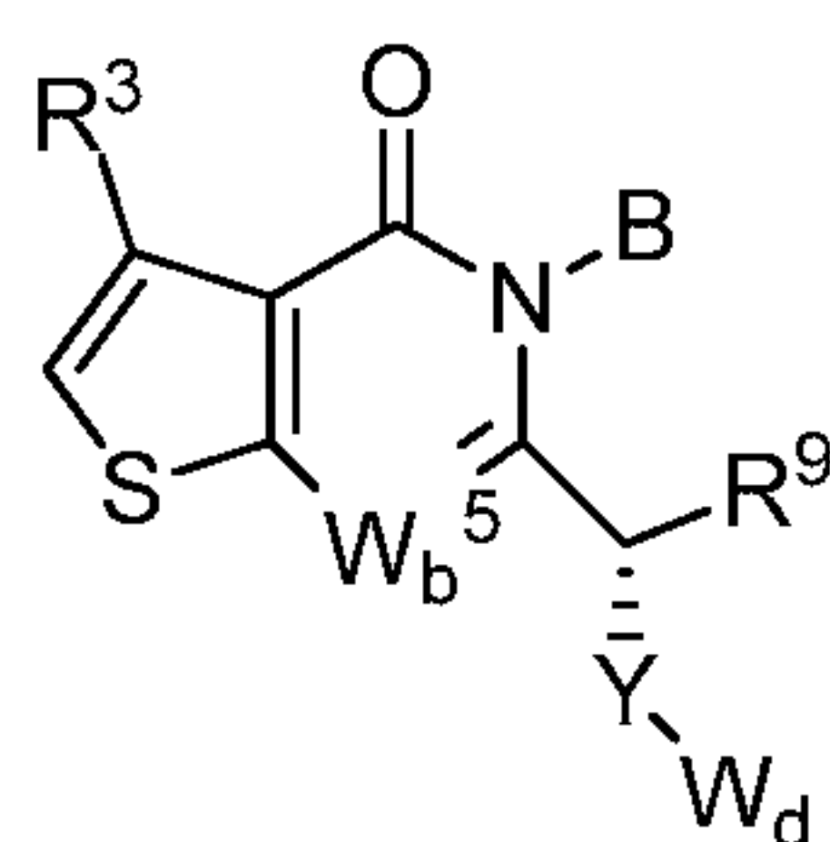
Formula (VIIa)
