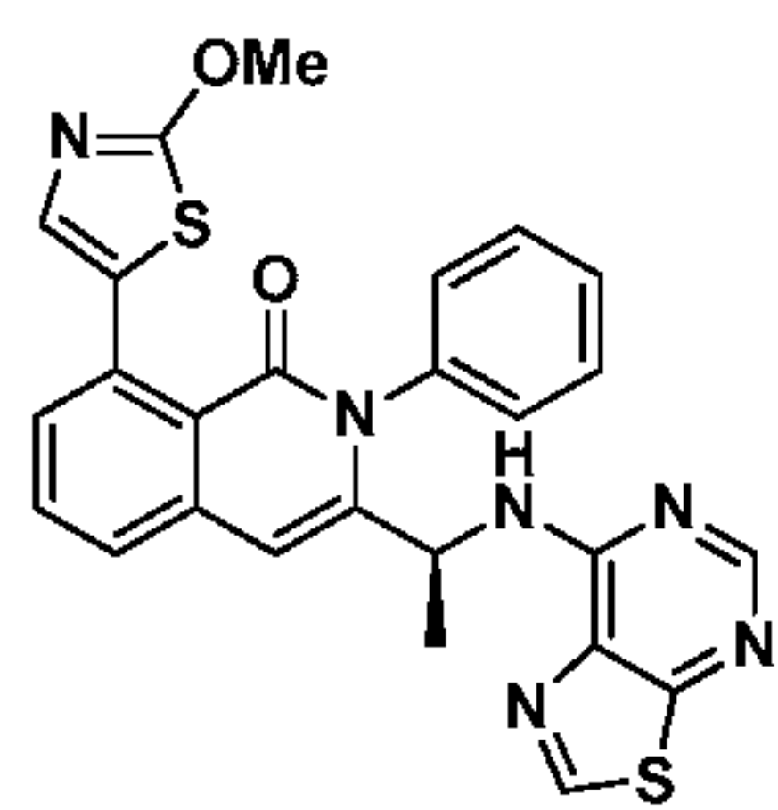
Compound 93,
