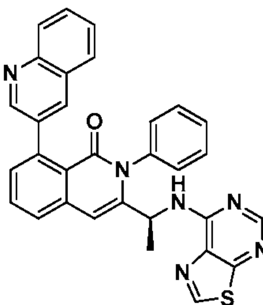
Compound 41,
