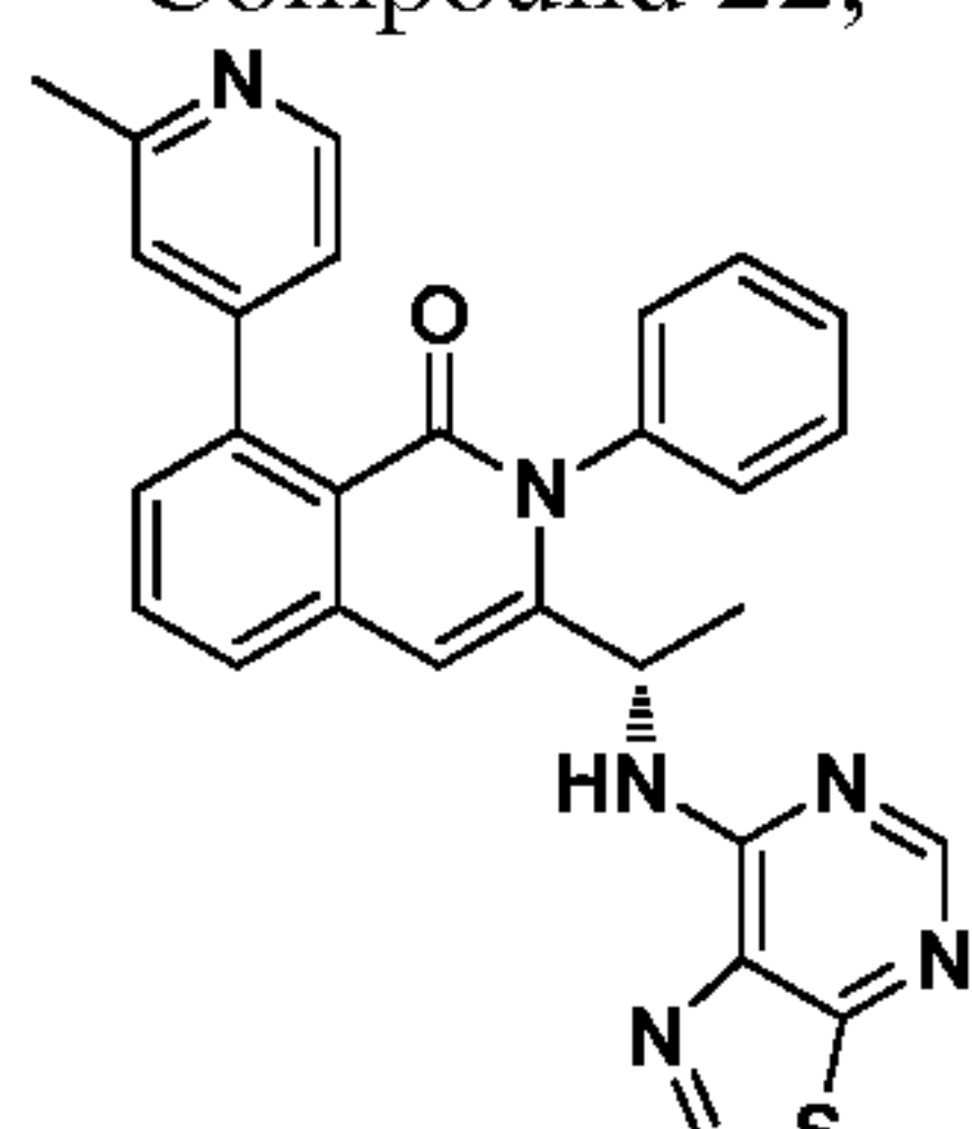
Compound 27,
