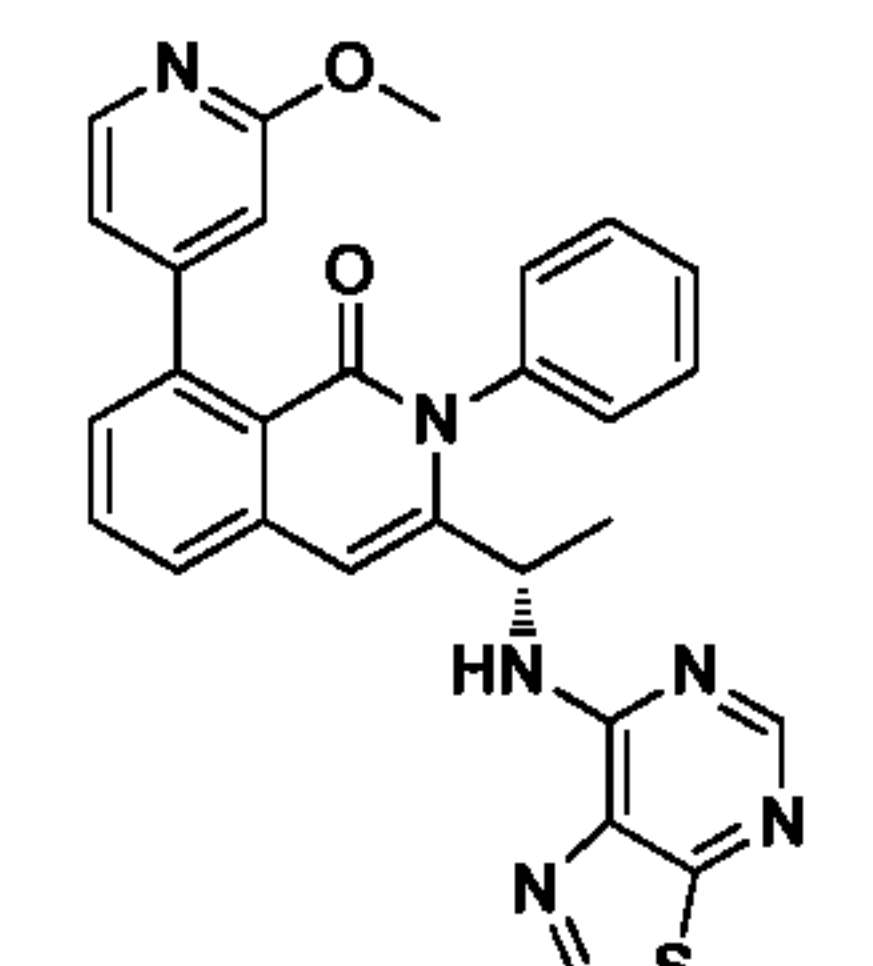
Compound 52,
