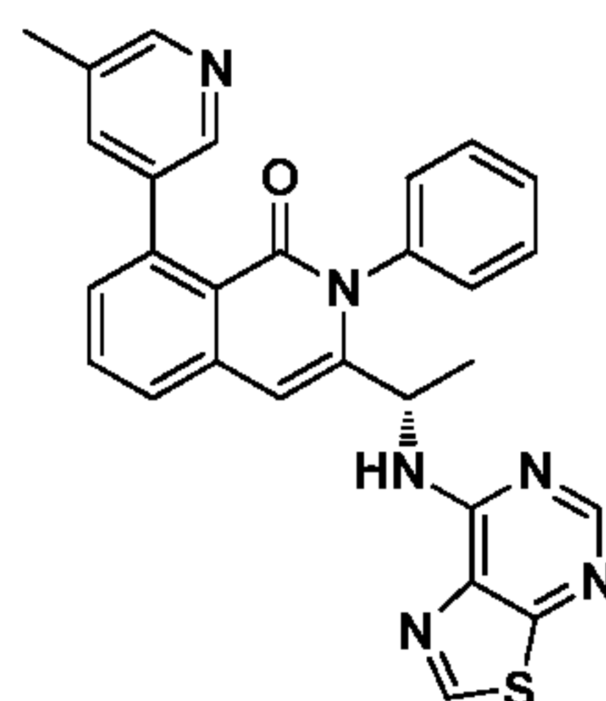
Compound 20,
