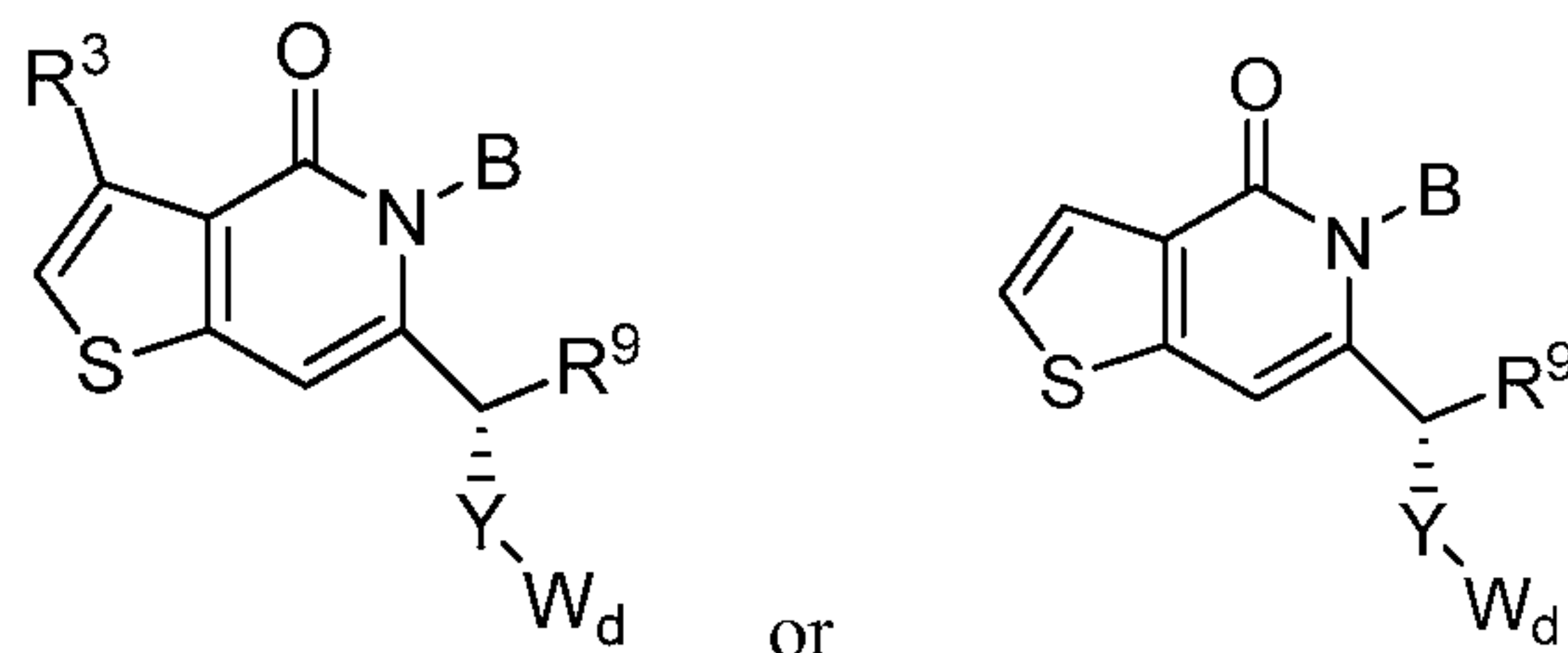
Formula (IXa)
