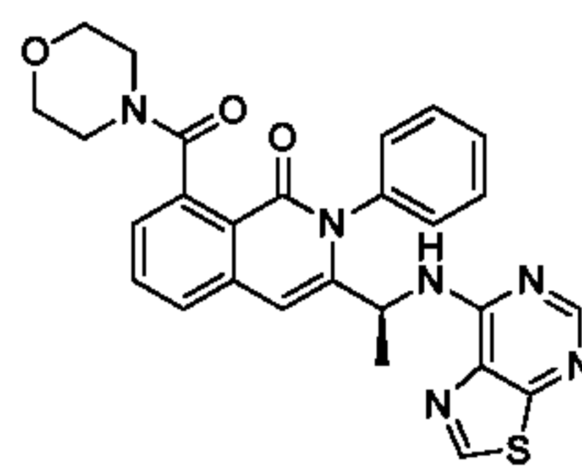
Compound 86,
