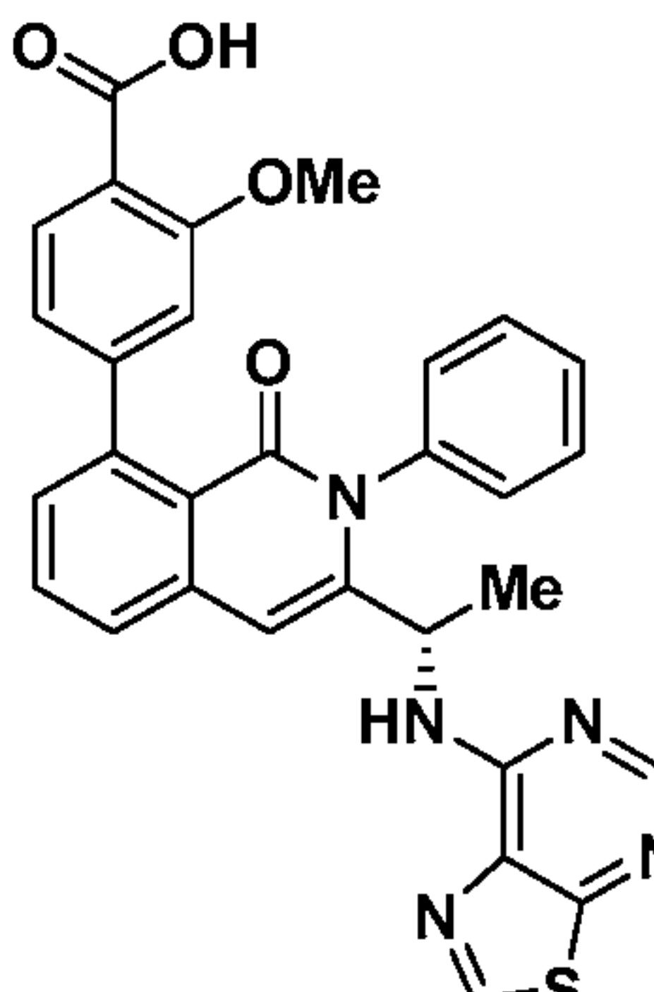
Compound 112,
