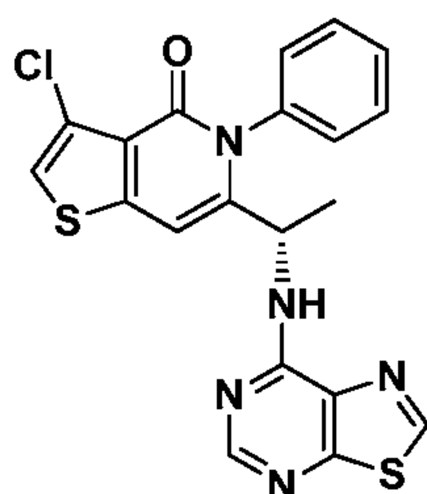
Compound 15,
