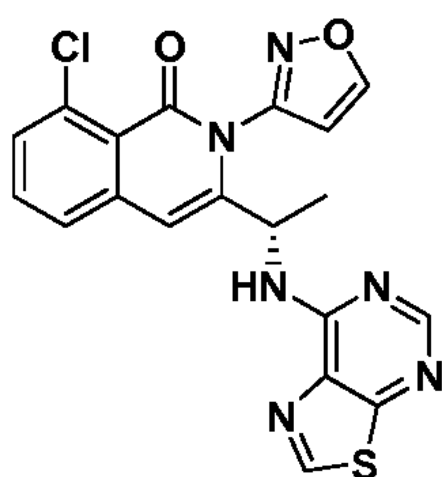
Compound 105 ,
