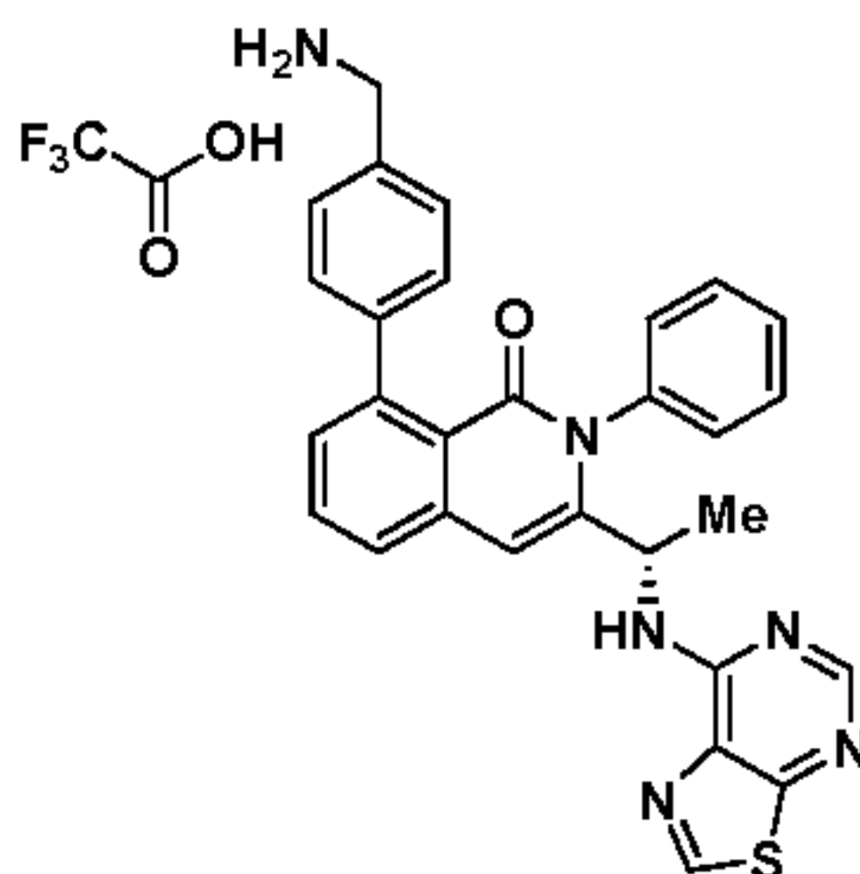
Compound 119,
