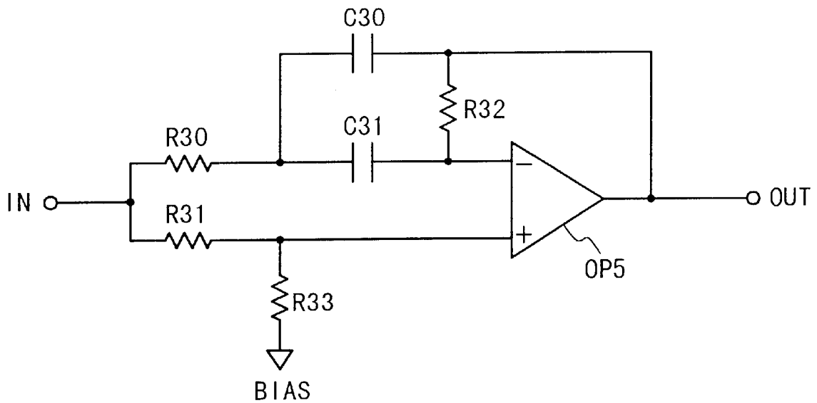
CIRCUIT ARRANGMENT OF DELAY DEVICE 12a, OR 12b
