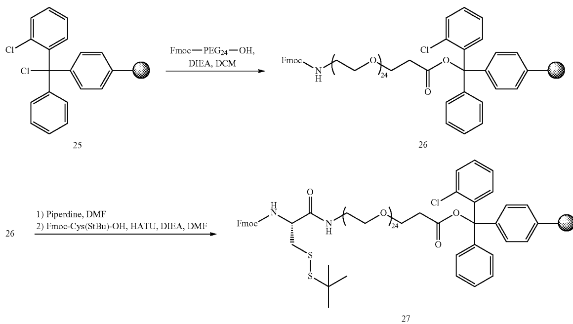
Scheme 13: Synthesis of mPEG 24 -Cys(StBu)-Lys(MDpr)-Cys(SBu)-PEG 24 -OH (Scaffold A)
