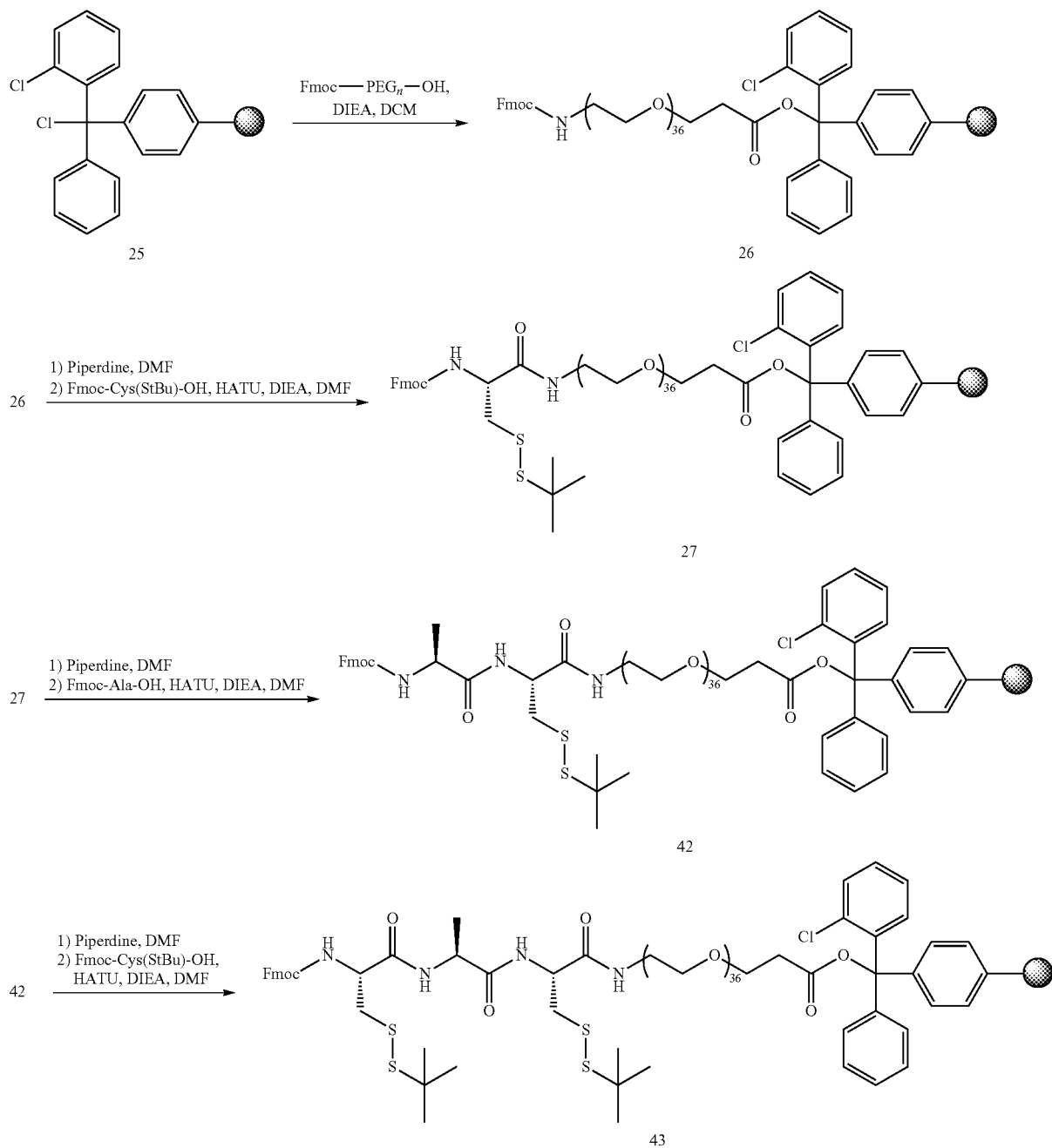
Scheme 12. Synthesis of MDpr-Cys(StBu)-Ala-Cys(StBu)-PEG 36 -OH (Scaffold B)
