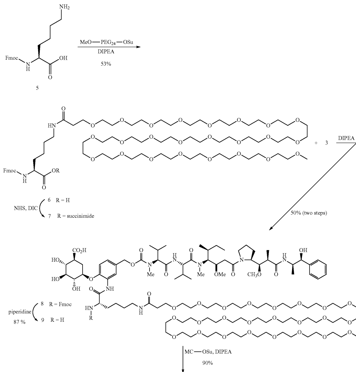
Scheme 2.
