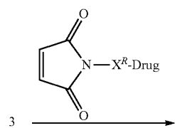
Scheme 16: Conjugation of Maleimide Containing Drug Linkers to Branched Drug Carrier:
