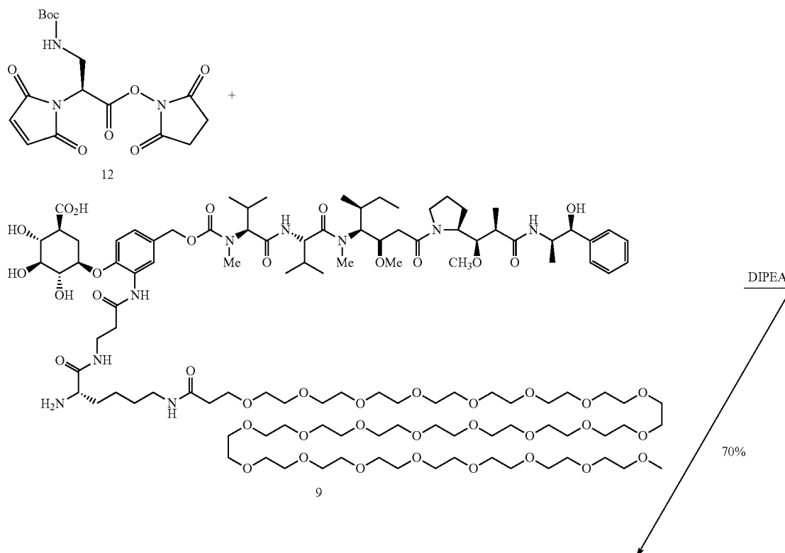
Scheme 4.
