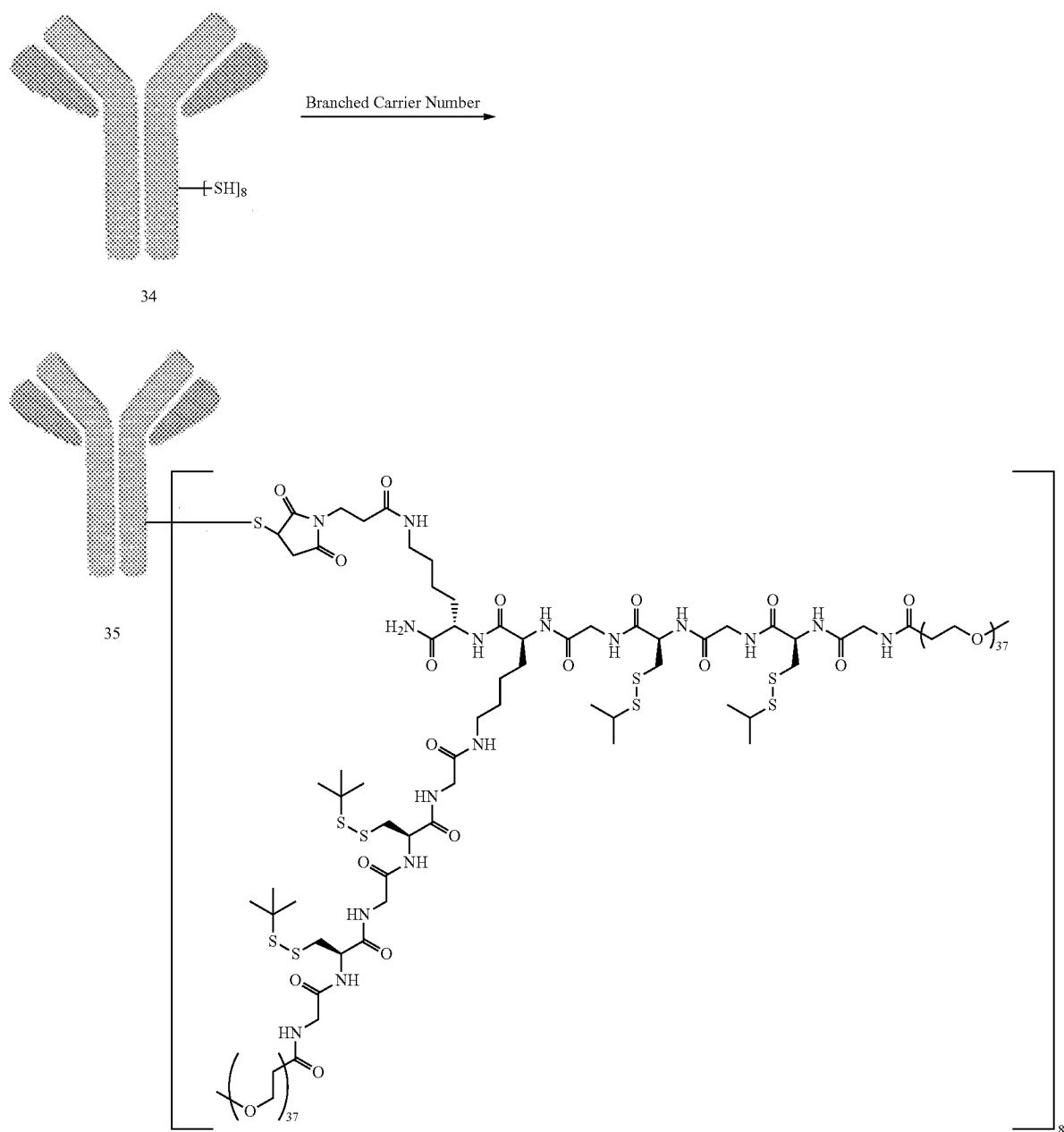
Scheme 15: Conjugation of Maleimide Containing PEGylated Branched Drug Carrier Scaffold and Removal of t-Butylthiol Protecting Groups
