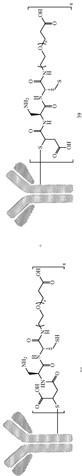
Scheme 11: Drug Conjugation of PEGylated Scaffolds
