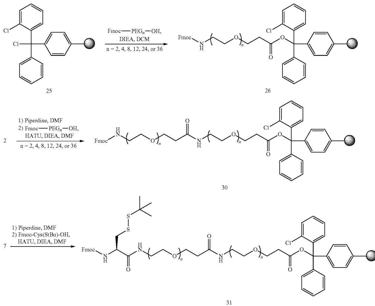
Scheme 8: Synthesis of MDpr-Cys(StBu)-PEG 48-72 -OH
