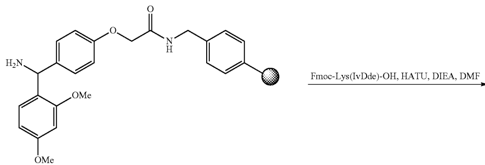
Scheme 14: Branched PEGylated Drug-Carrier Scaffold (Scaffold C)
