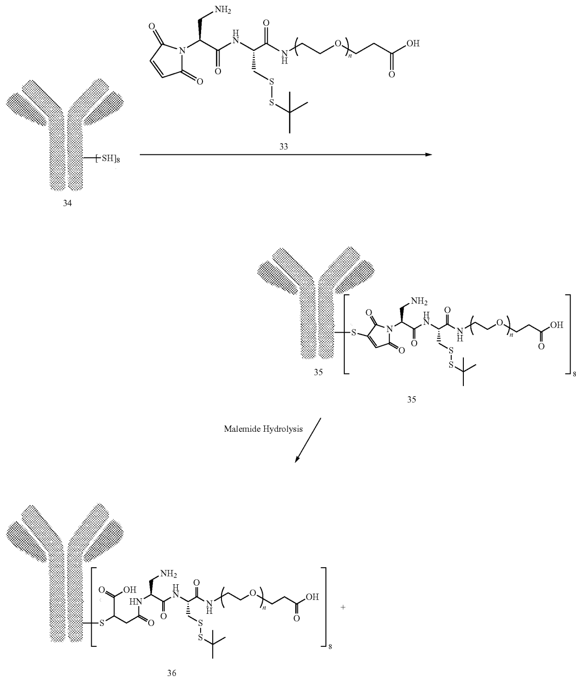
Scheme 9: Conjugation of PEGylated Scaffold to Fully Reduced Antibody Interchain Disulfides
