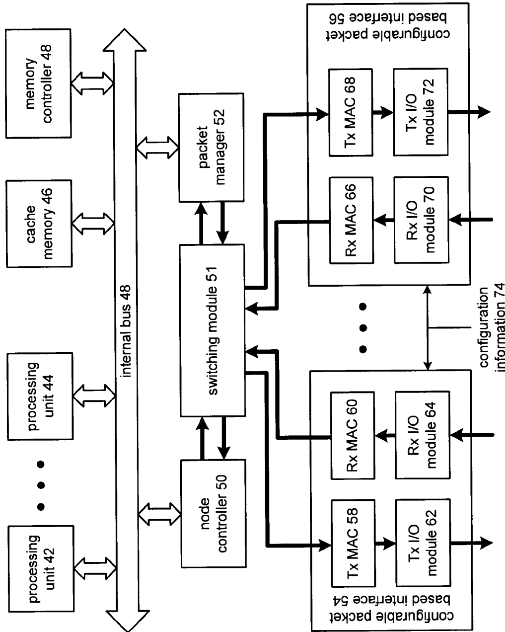
FIG. 4 multiple processor device 40
