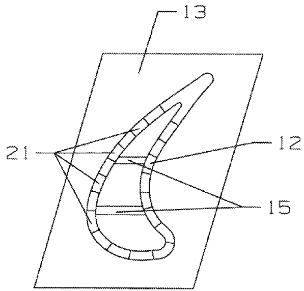
View A-A Fig 2
