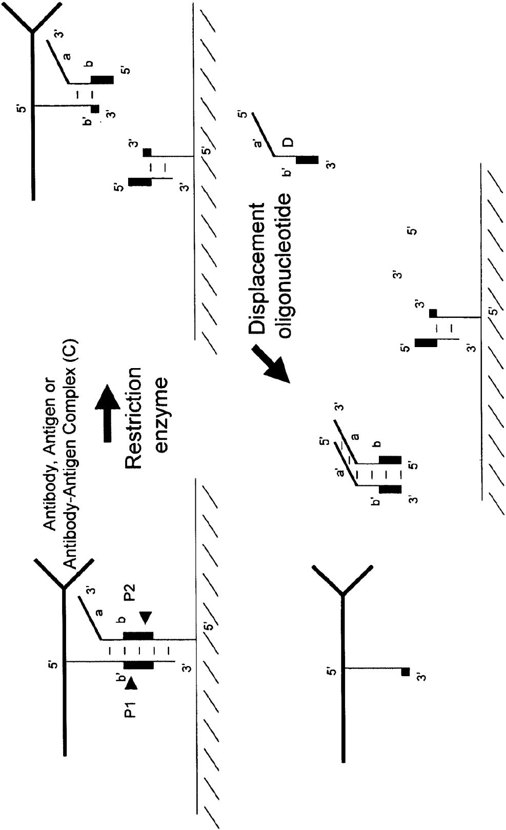
FIGURE 6B Restriction endonuclease-mediated release
