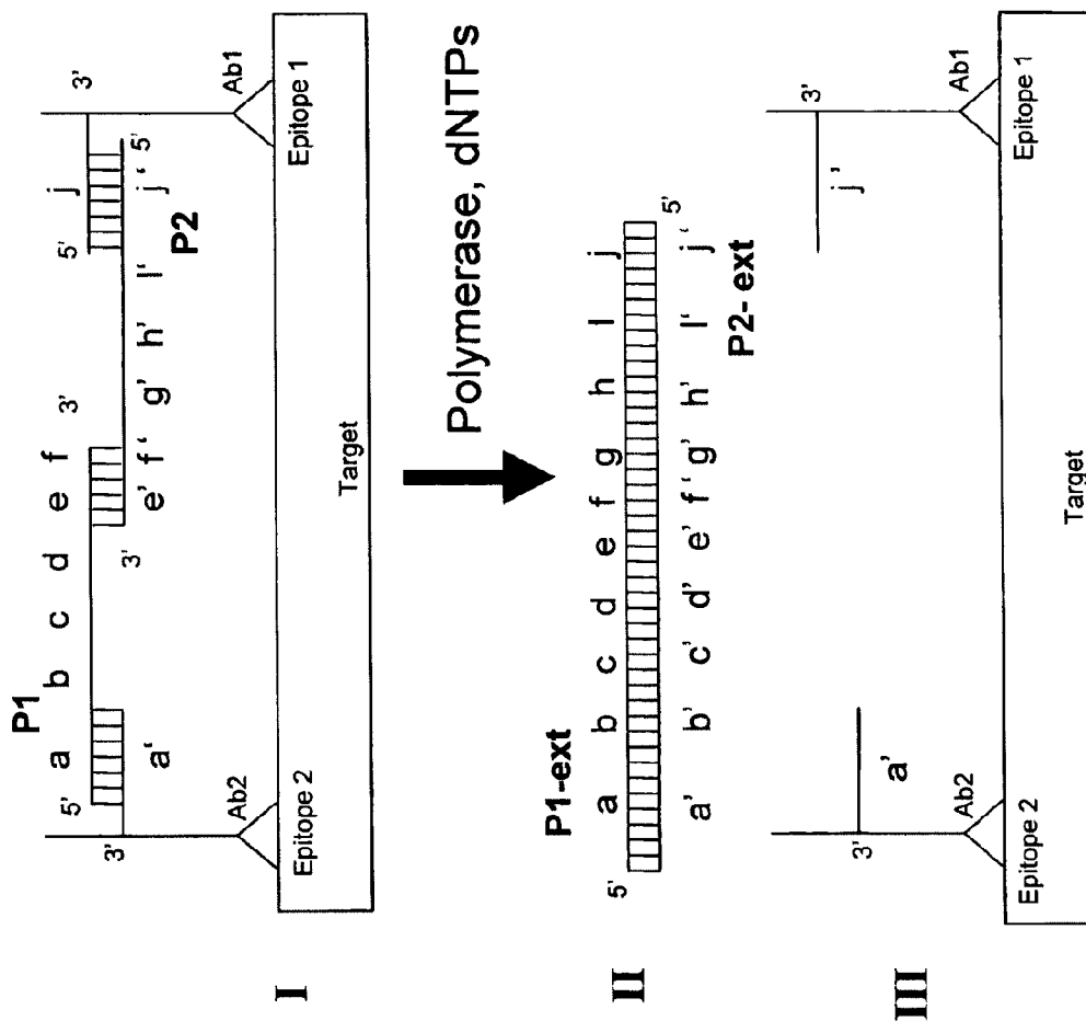
FIGURE 3F Extension / displacement of splint probes
