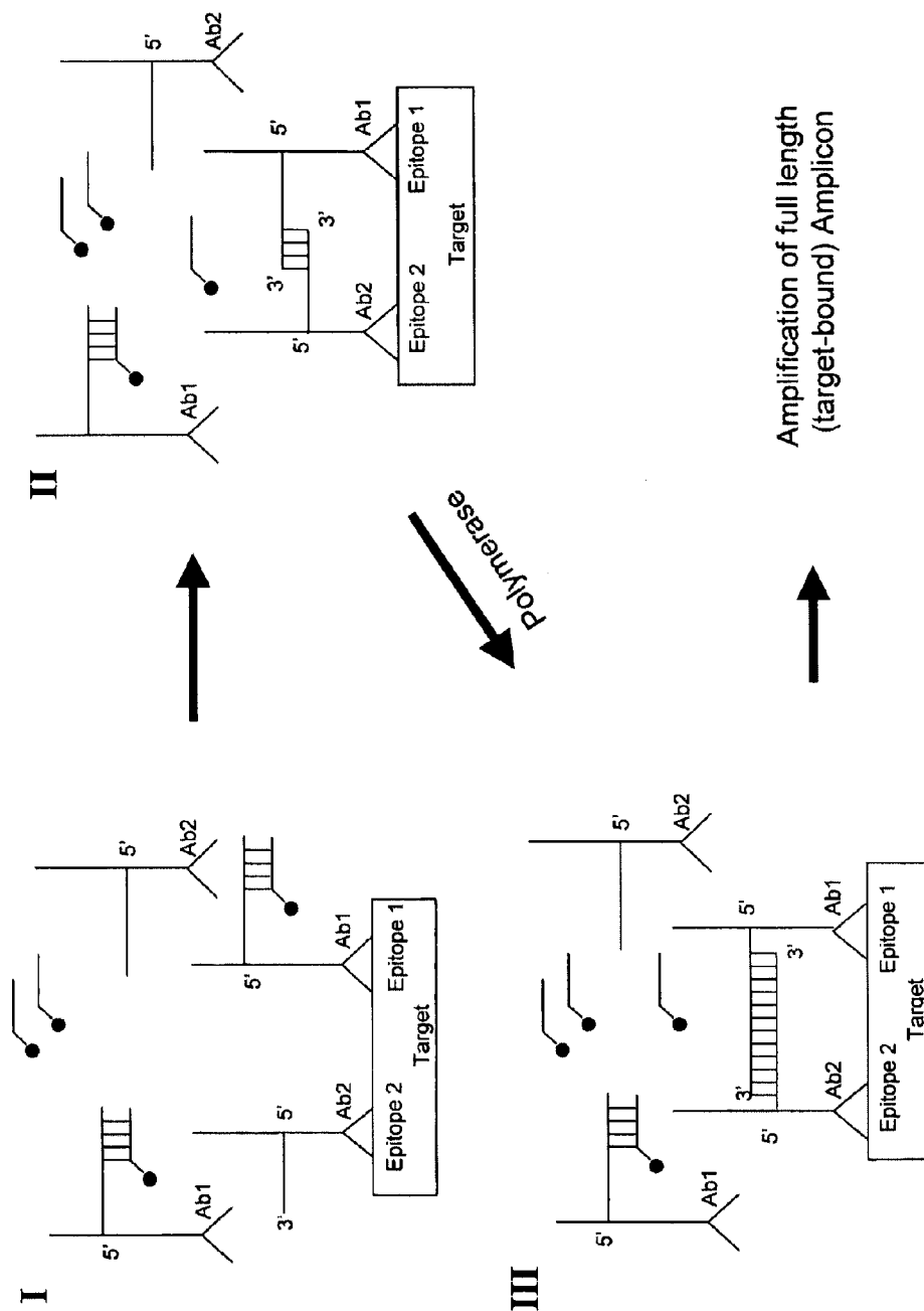
FIGURE 4F Competitive blocker oligonucleotide in binary immuno-SDA
