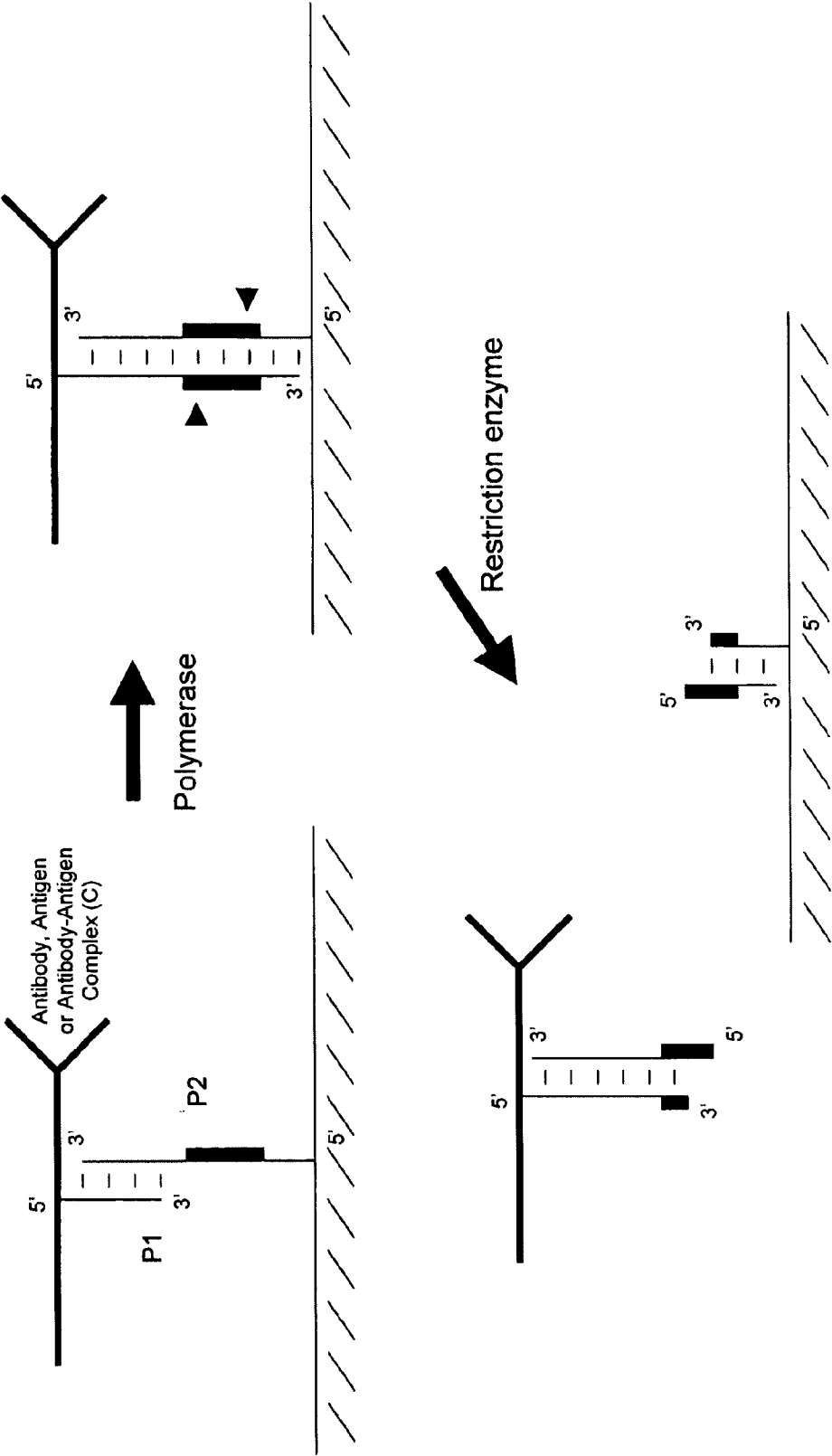
FIGURE 6D Polymerase and restriction endonuclease-mediated release
