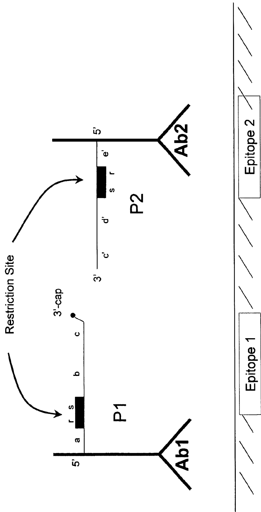
FIGURE 14A Immuno-SDA using capped oligonucleotide probes: Mixing of antigens and oligonucleotide-conjugated antibodies
