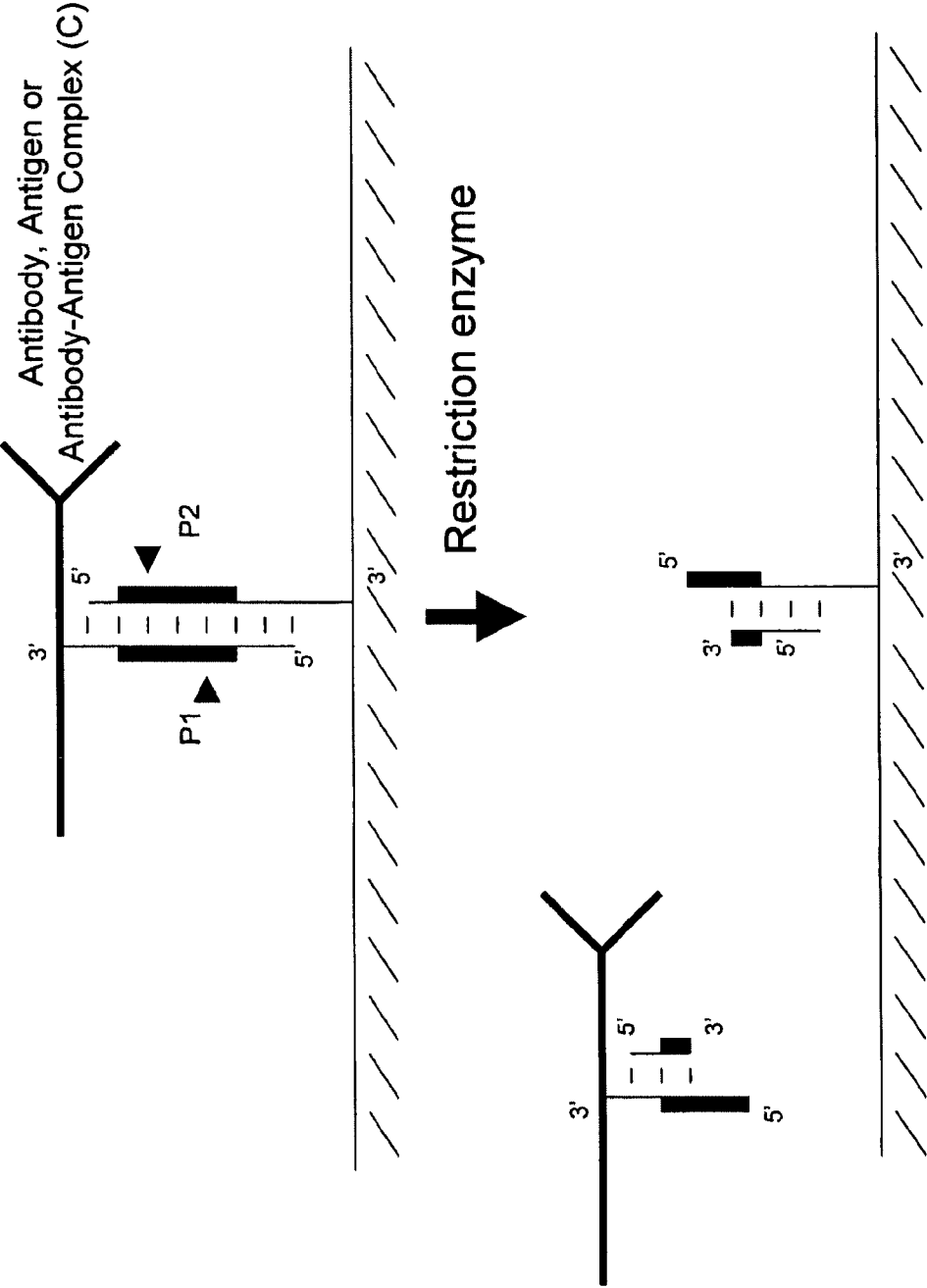
FIGURE 6C Restriction endonuclease-mediated release
