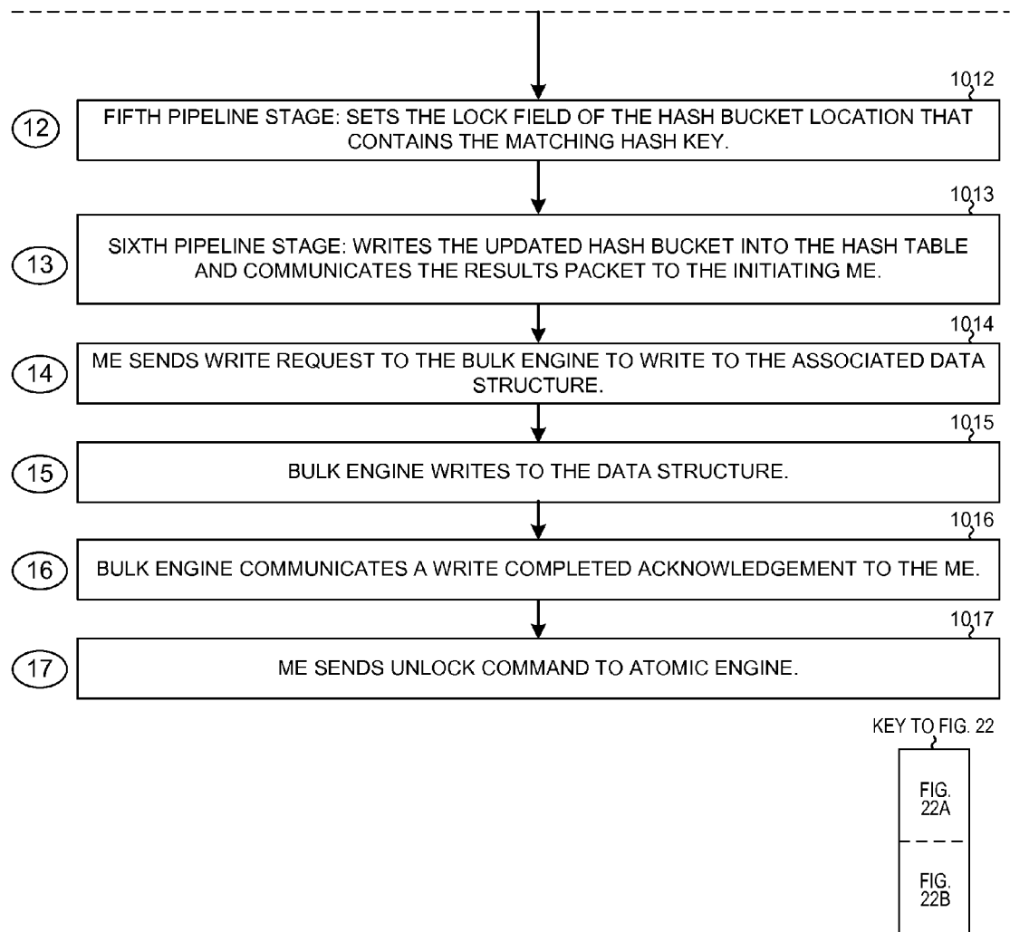
TRANSACTIONAL MEMORY FLOWCHART FIG. 22B
