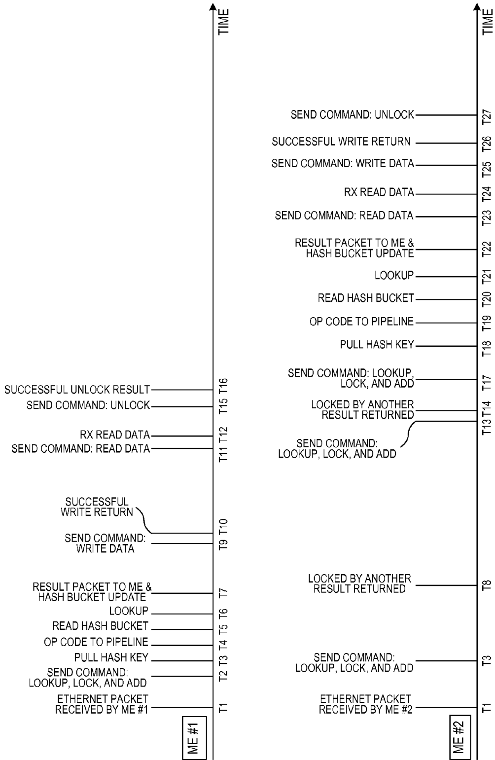
LOOKUP, LOCK, AND ADD TIMING DIAGRAM
