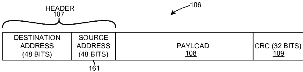
ETHERNET PACKET FIG. 15
