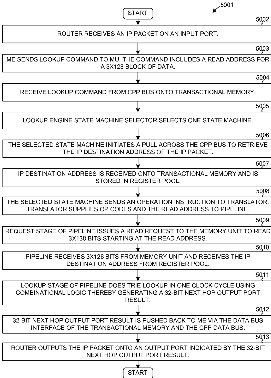
FLOWCHART OF A TRIE MULTI-BIT LOOKUP OPERATION
