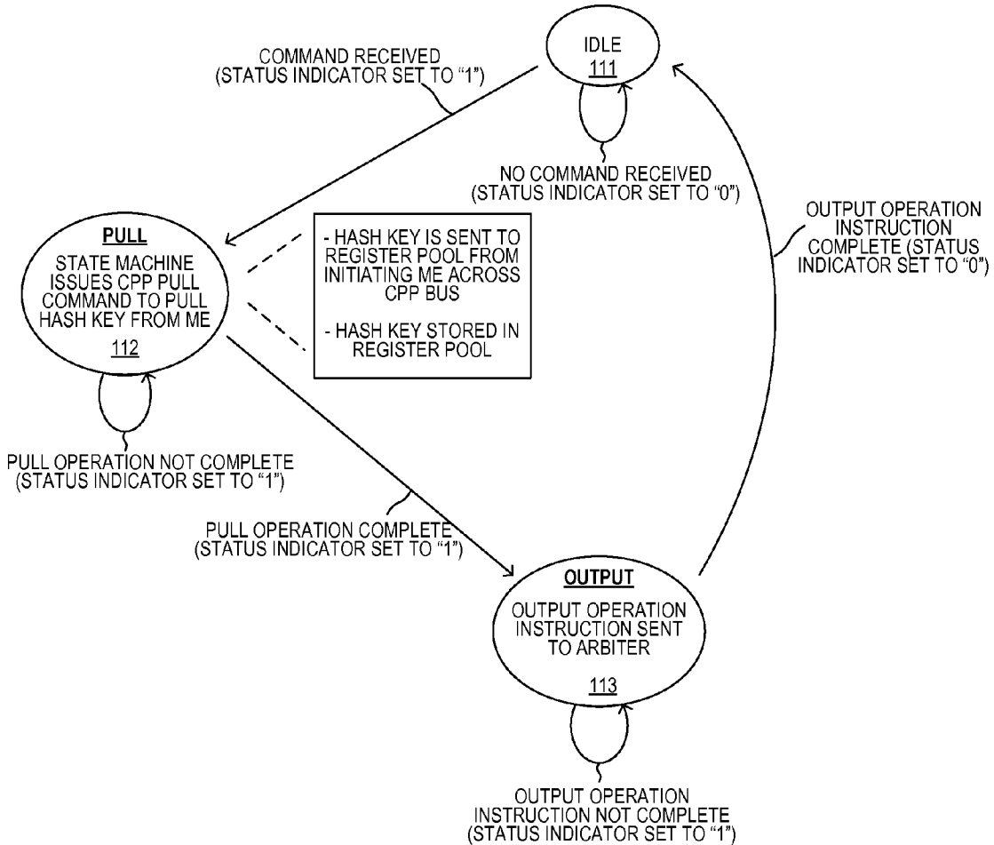
STATE MACHINE STATE DIAGRAM FIG. 16
