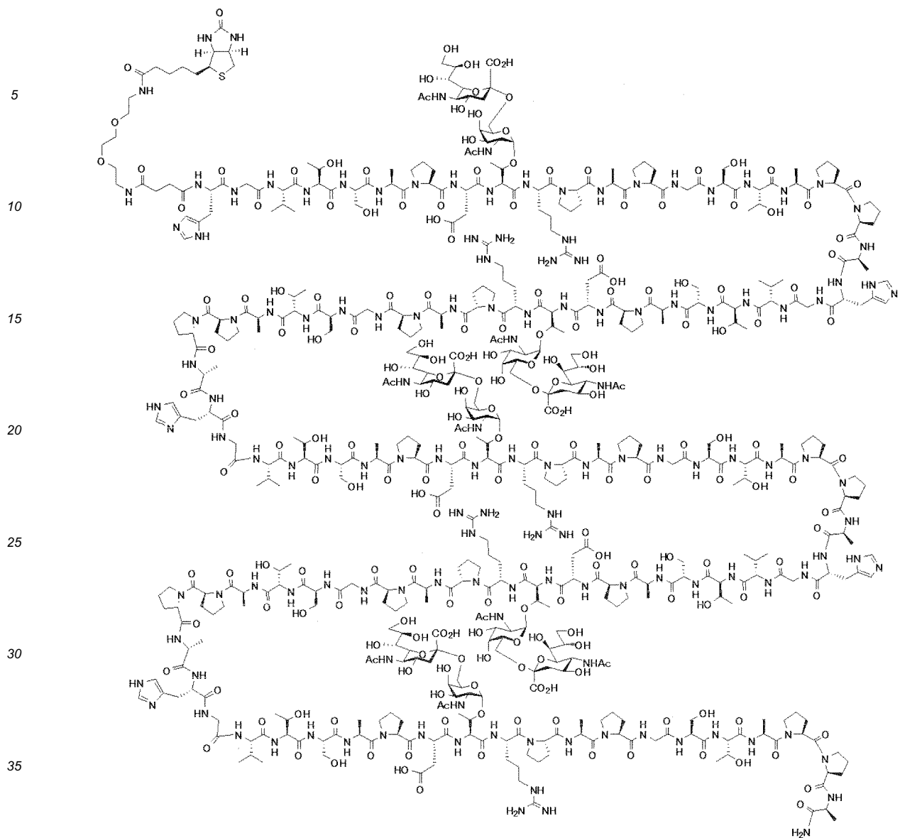
40 Compound 19
