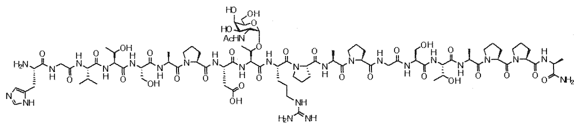
Compound 4
