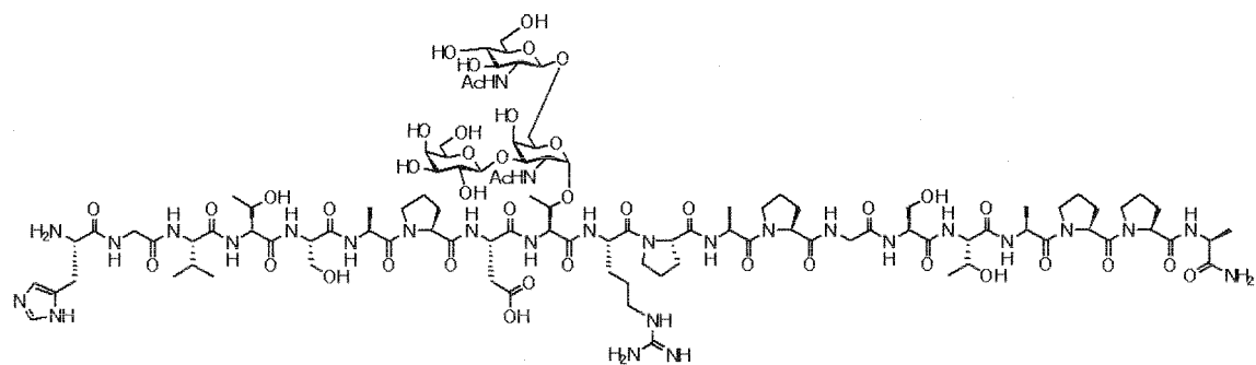
Compound 6
