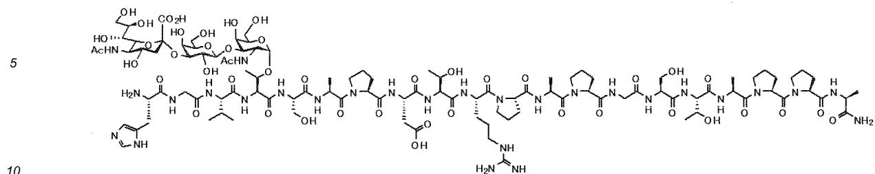
[Chemical Formula 12]
