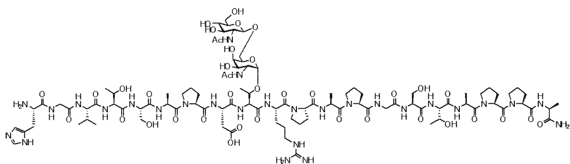
Compound 10
