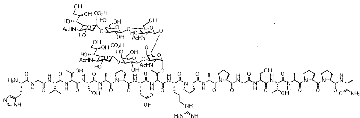
Compound 9
