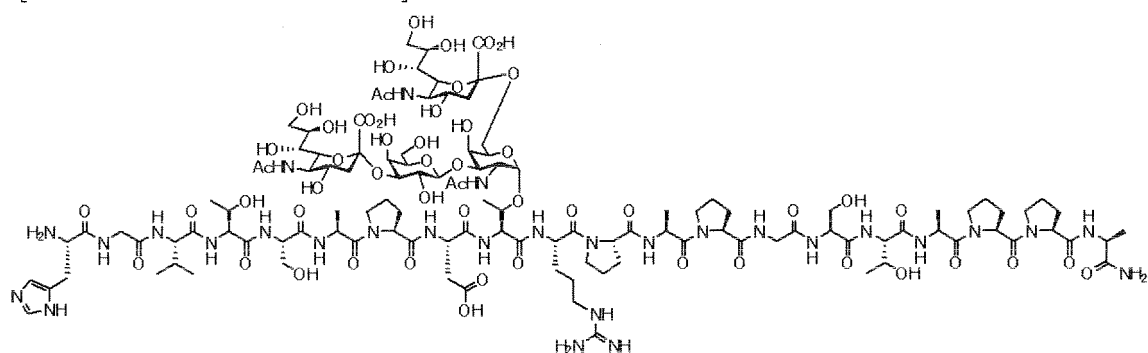
Compound 12
