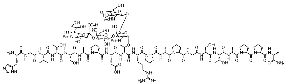
Compound 7
