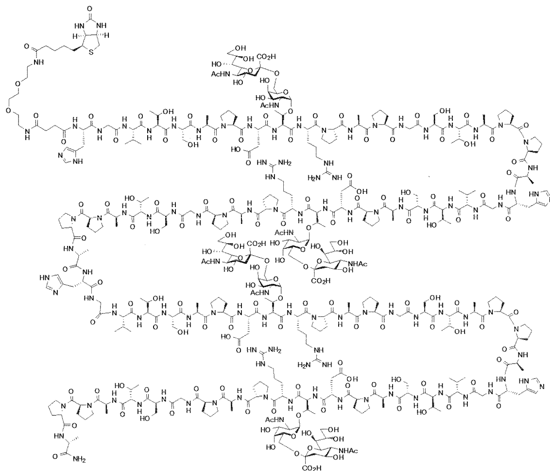
Compound 18
