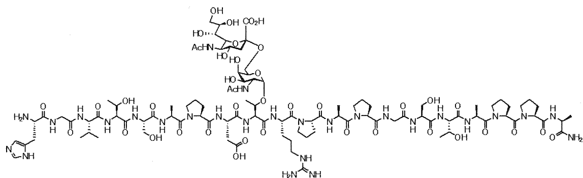
Compound 5
