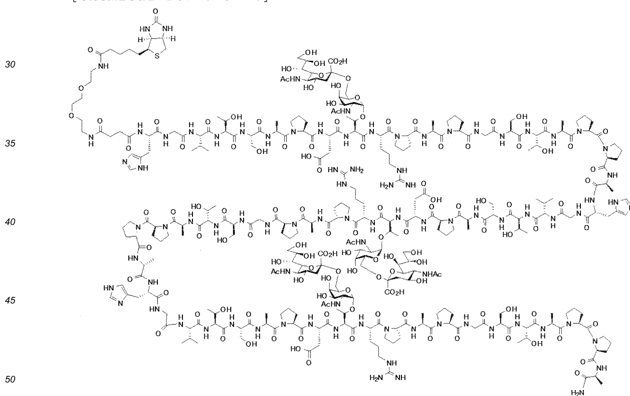
Compound 17
