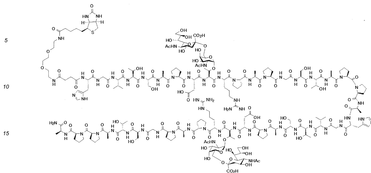
Compound 16
