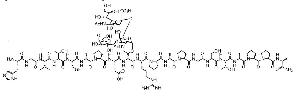
Compound 11
