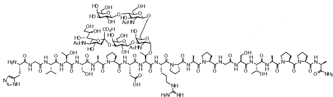
Compound 8
