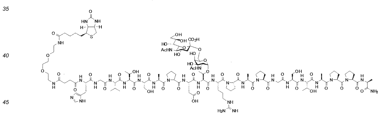
[Chemical Formula 14]
