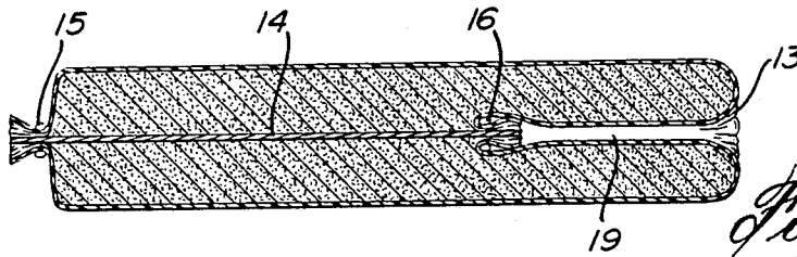
Fig. 1 PRIOR ART
