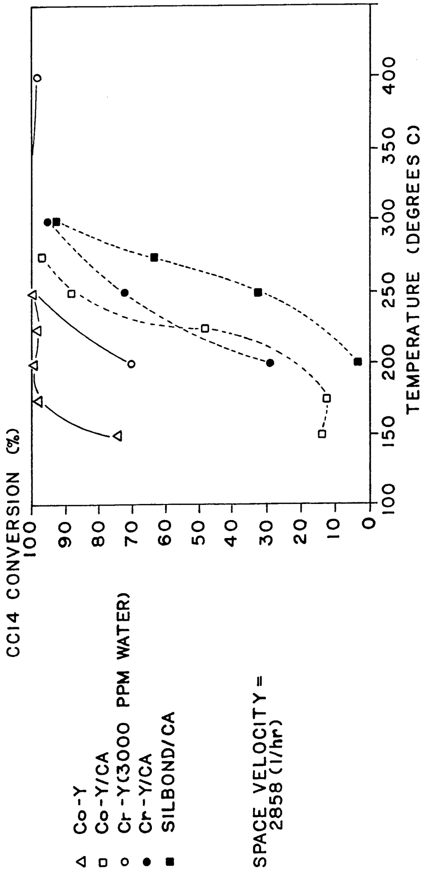
CCl4 CONVERSION VS. TEMPERATURE PLOT WITH VARIOUS CATALYSTS (MONOLITHS)
