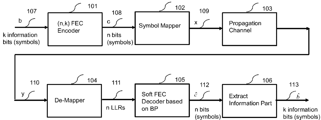
System model for a linear block code encoder, channel and soft decoder based on BP
