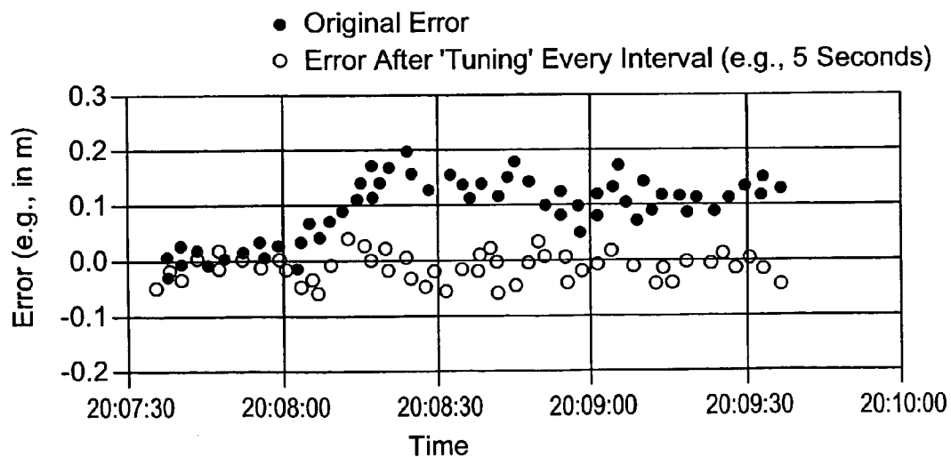
Fig. 13 DGPS by "Tuning" Positioning Error
