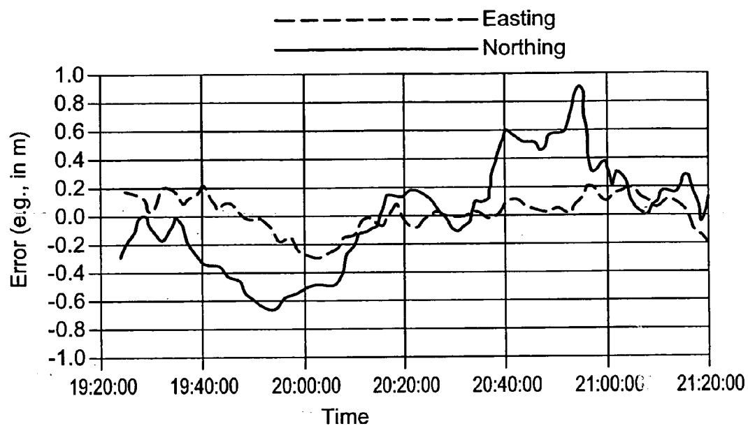
Fig. 12 DGPS Static Positioning Error
