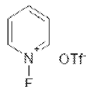
N-Fluoropyridinium triflate
