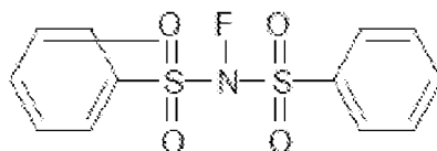
NFSI
