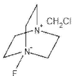
F-TEDA or Selectfluor
