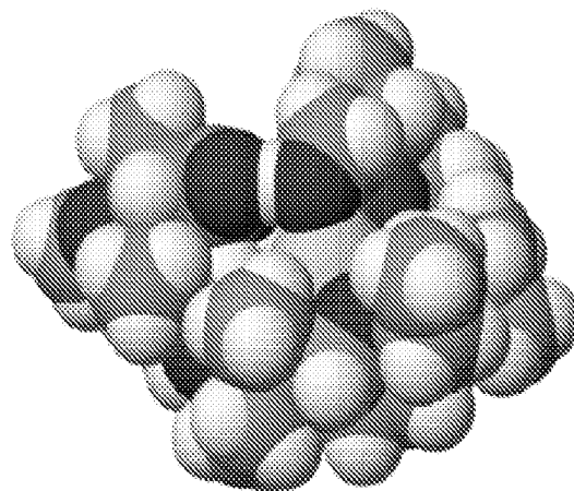
Monensin A – complexed around sodium ion
