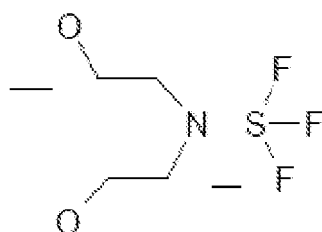
Deoxo-Fluorine
