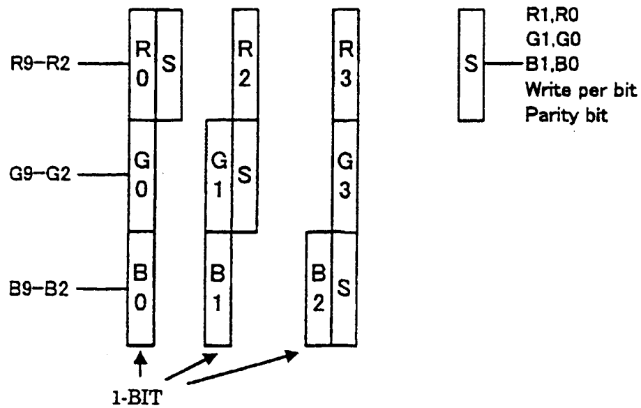
(b) BIT ASSIGN OF 30-BIT COLOR
