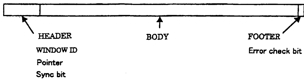
(c) FORMAT OF PACKET VIDEO DATA
