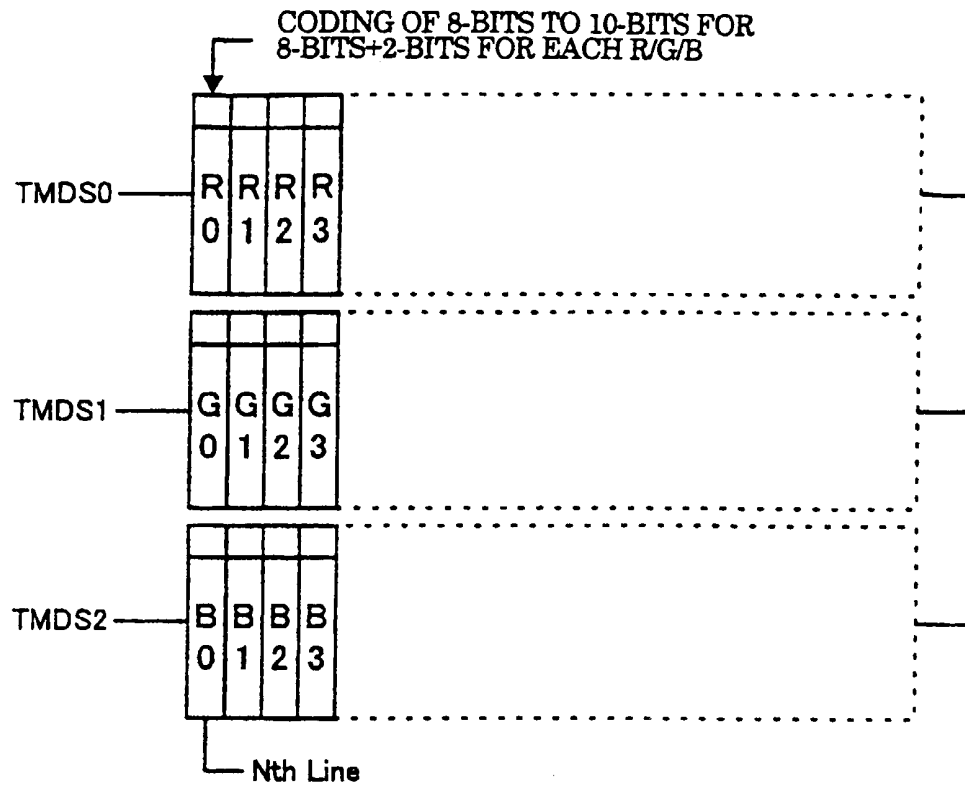
(a) TMDs DATA TRANSFER
