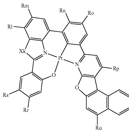
Structure of A_k^a - (Rl)(Rm)(Rn)(Ro)(Rp)(Rr)(Rs)
