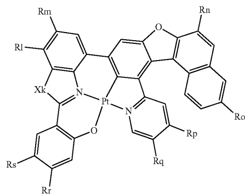
Structure of A_k^{a-} (Rl)(Rm)(Rn)(Ro)(Rp)(Rq)(Rr)(Rs)
