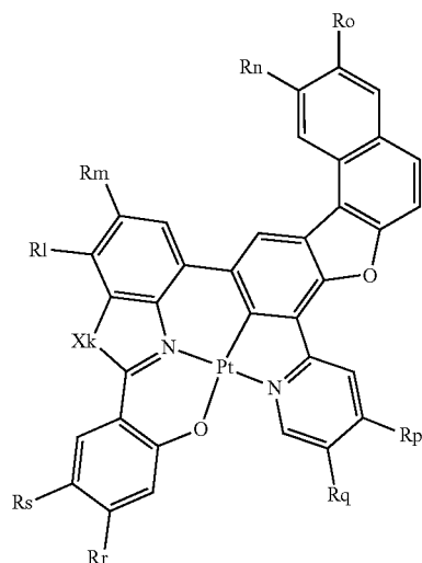
Structure of A_k^{a-} (Rl)(Rm)(Rn)(Ro)(Rp)(Rq)(Rr)(Rs)
