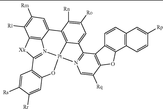
Structure of A_k^{a-} (Rl)(Rm)(Rn)(Ro)(Rp)(Rq)(Rr)(Rs)
