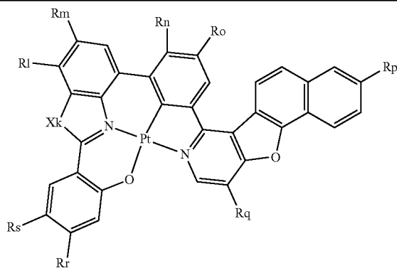
Structure of A_8^{a-} (Rl)(Rm)(Rn)(Ro)(Rp)(Rq)(Rr)(Rs)
