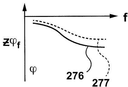
Frequency profile of Z^{\phi_f} during safe state
