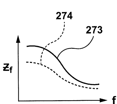
Frequency profile of Z_{mag} during safe state
