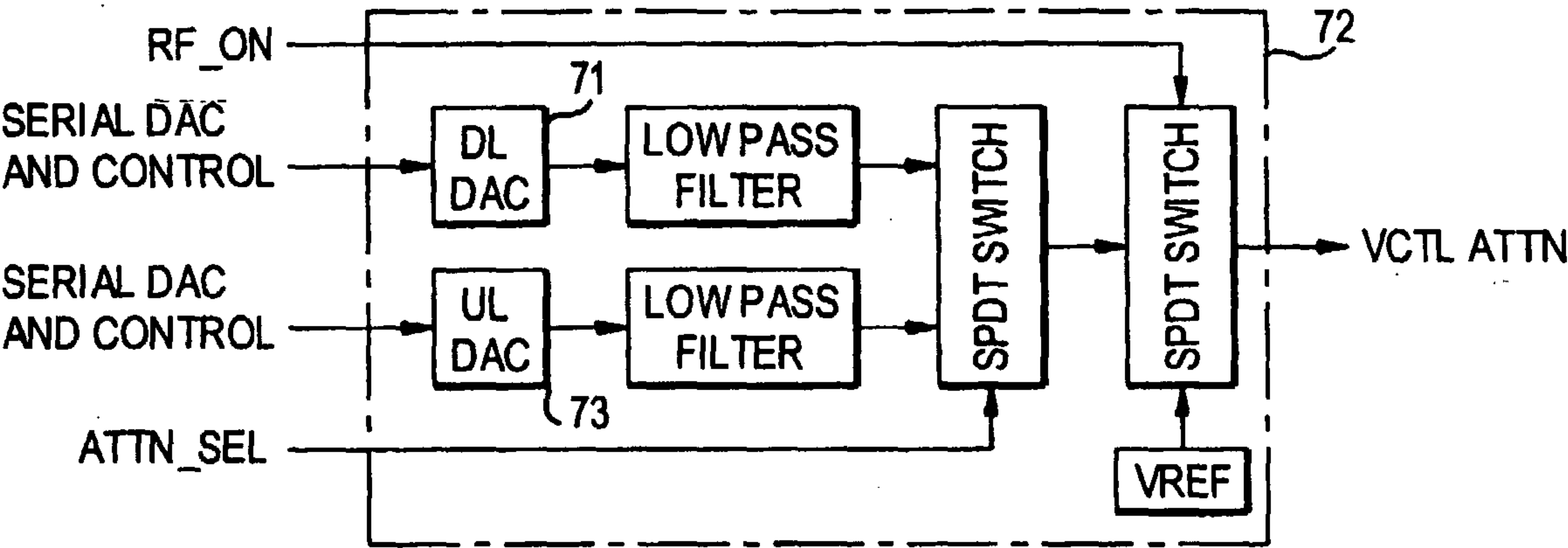
FIG. 9 DOWNLINK / UPLINK DAC'S AND POWER CONTROL BLOCK DIAGRAM
