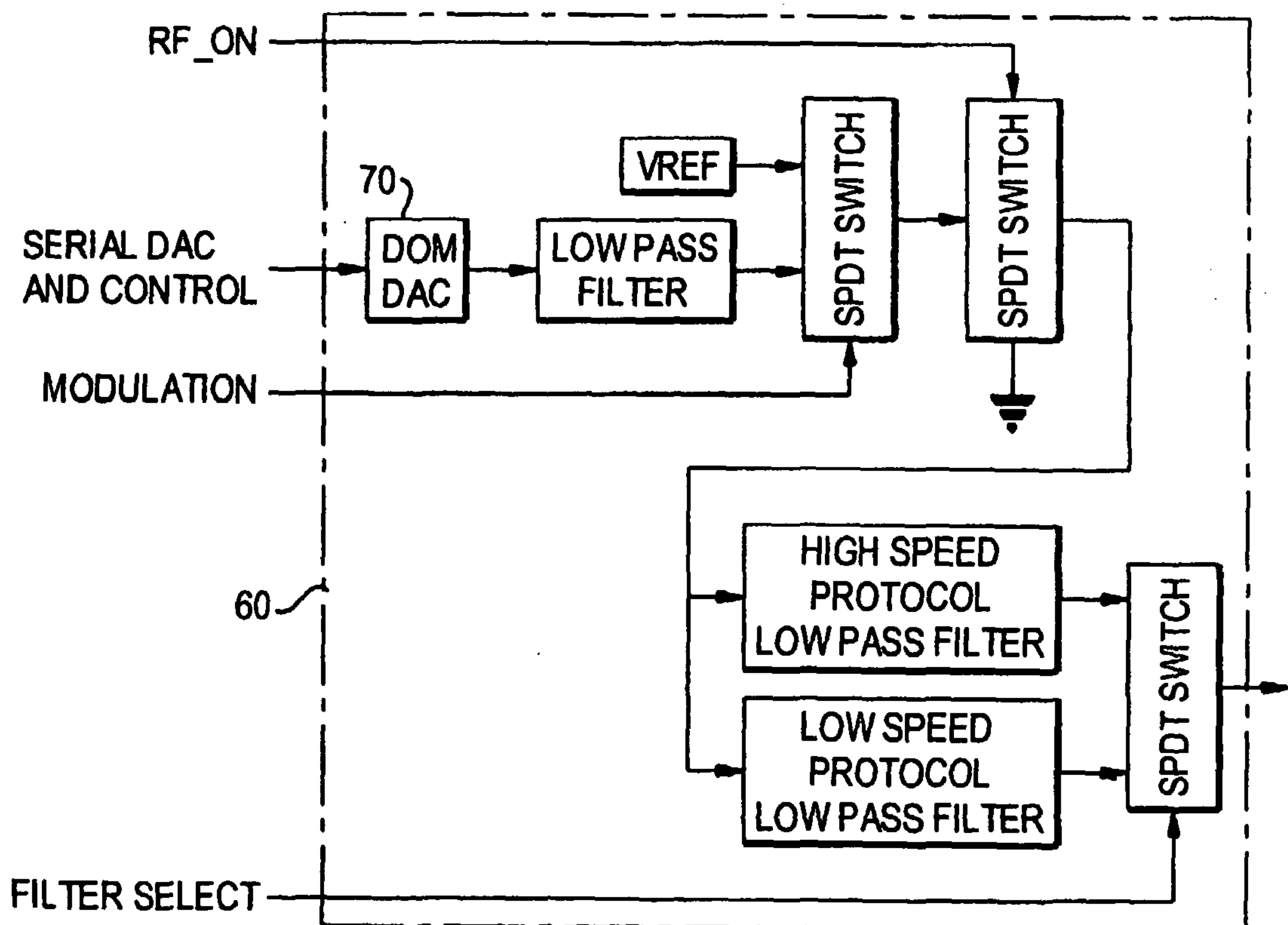
FIG. 7 DOM DAC AND MODULATION CONTROL BLOCK DIAGRAM
