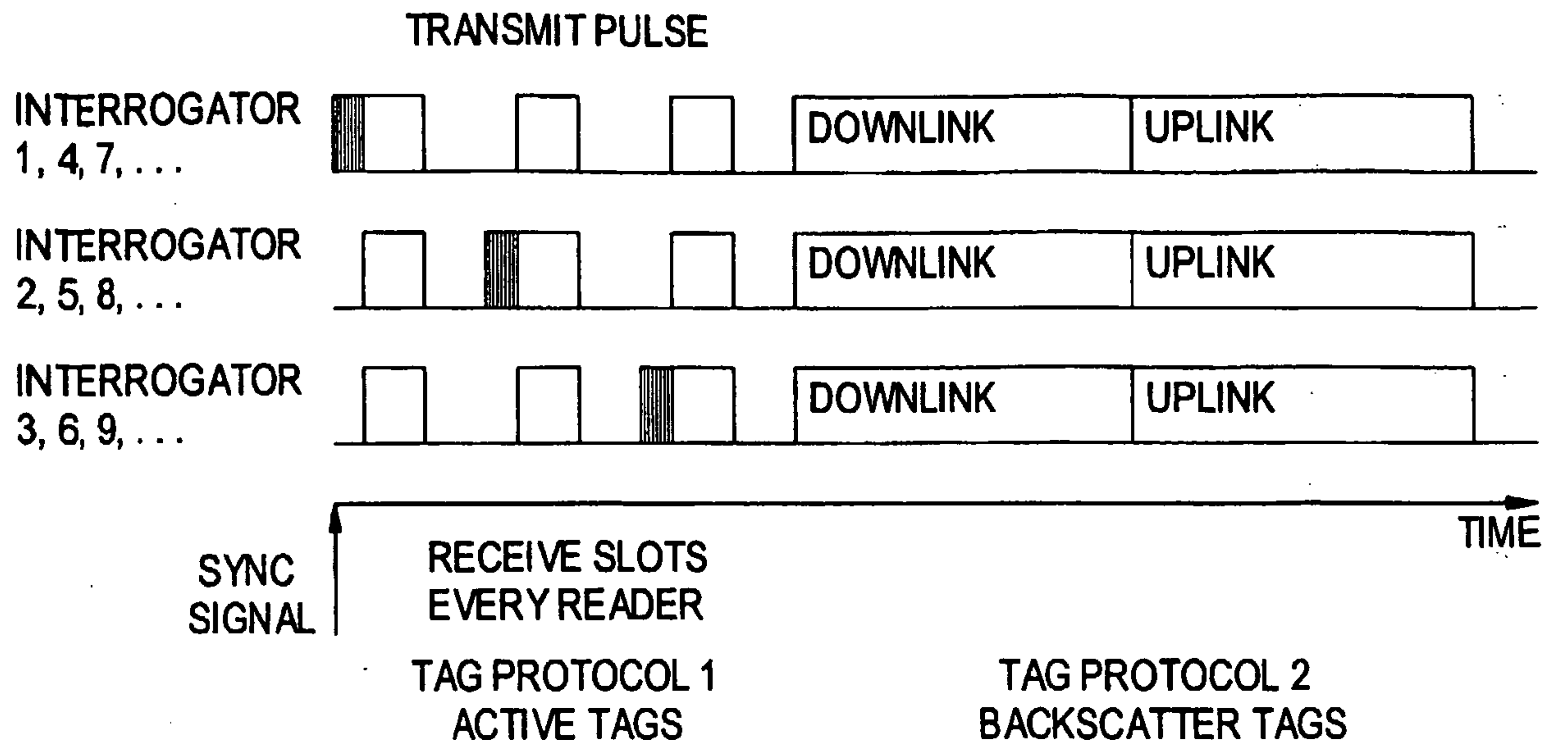
FIG. 3(c) TIME DIVISION MULTIPLEXING AND STEP LOCK COMBINATION FOR ACTIVE AND BACKSCATTER
