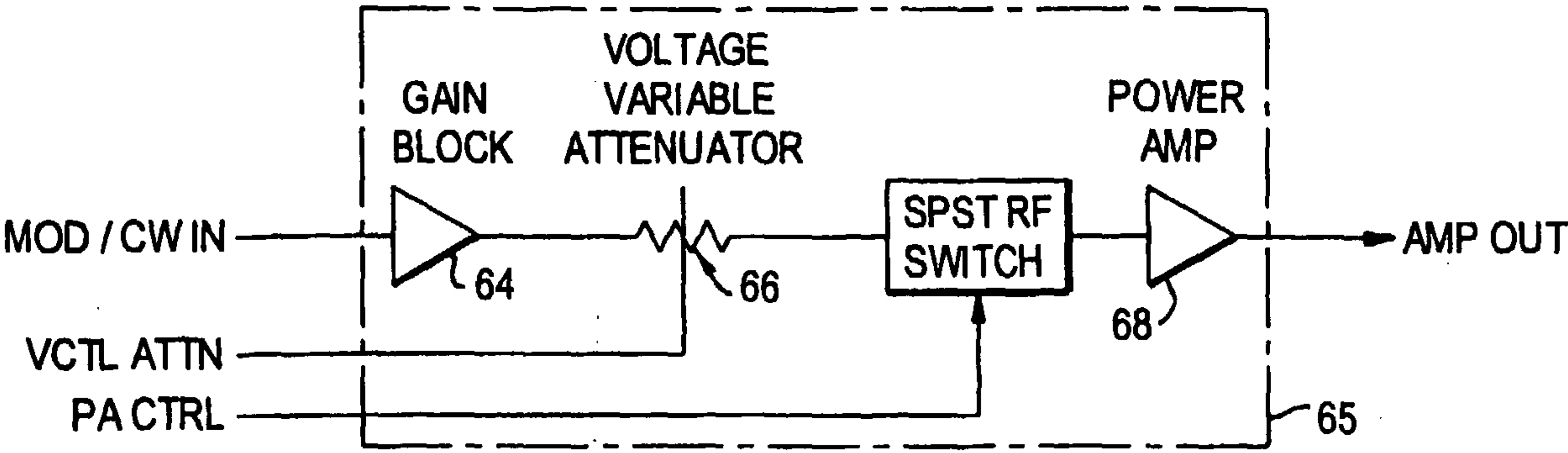
FIG. 8 POWER AMPLIFIER BLOCK DIAGRAM
