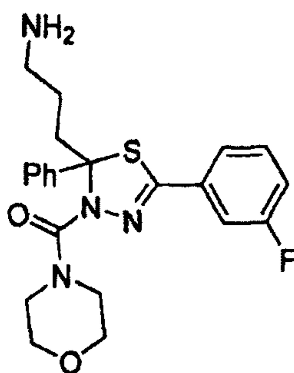
[2-(3-Aminopropyl)-5-(3-fluorophenyl)-2-phenyl-[1,3,4]thiadiazol-3-yl]-morpholin-4-yl-methanone
