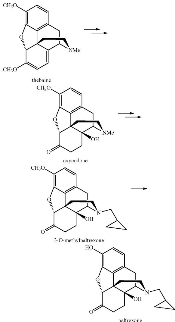
Scheme 3 Thebaine to naltrexone
