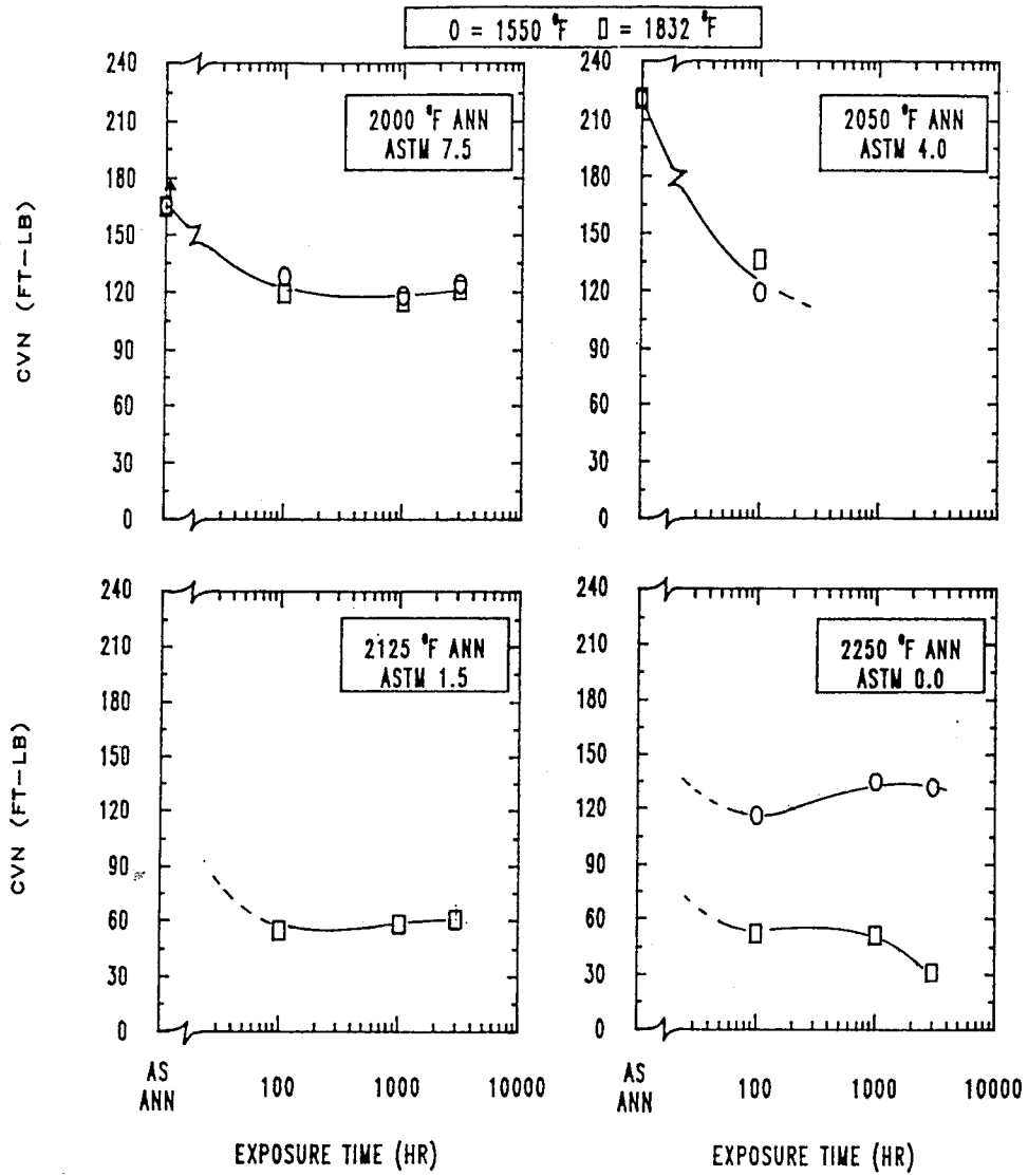
FIGURE 1 EFFECT OF EXPOSURE TIME ON IMPACT ENERGY
