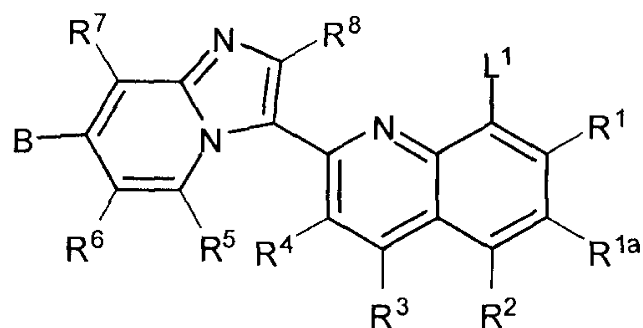
II
