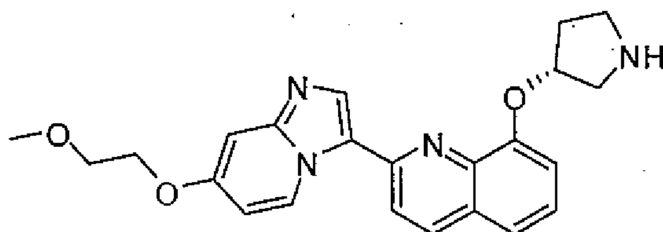
(R)-2-(7-(2-methoxyethoxy)imidazo[1,2-a]pyridin-3-yl)-8-(pyrrolidin-3-yloxy)quinoline
