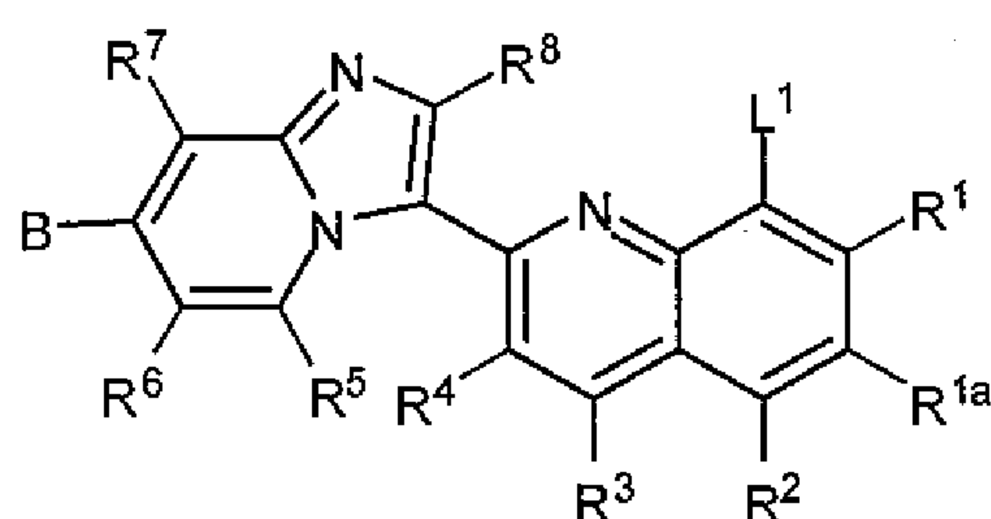
II
