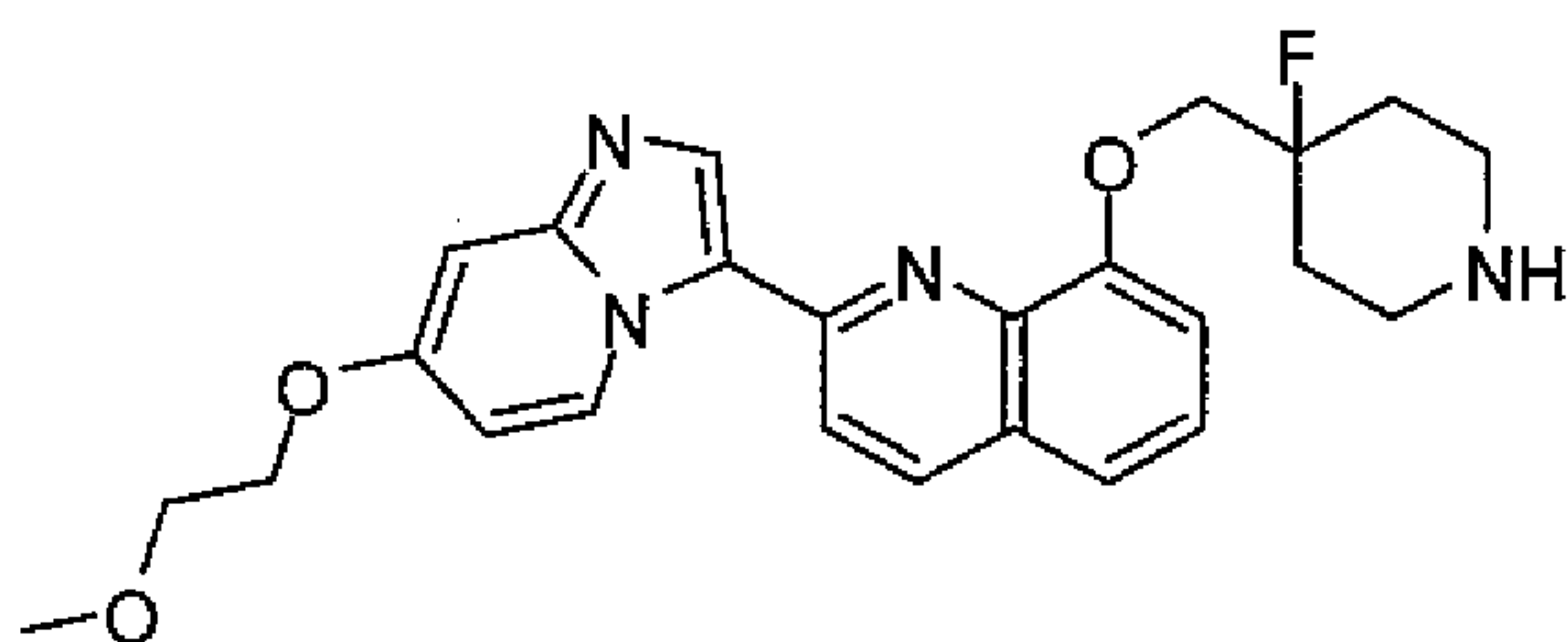
8-(((4-fluoropiperidin-4-yl)methoxy)-2-(7-(2-methoxyethoxy)imidazo[1,2-a]pyridin-3-yl)quinoline
