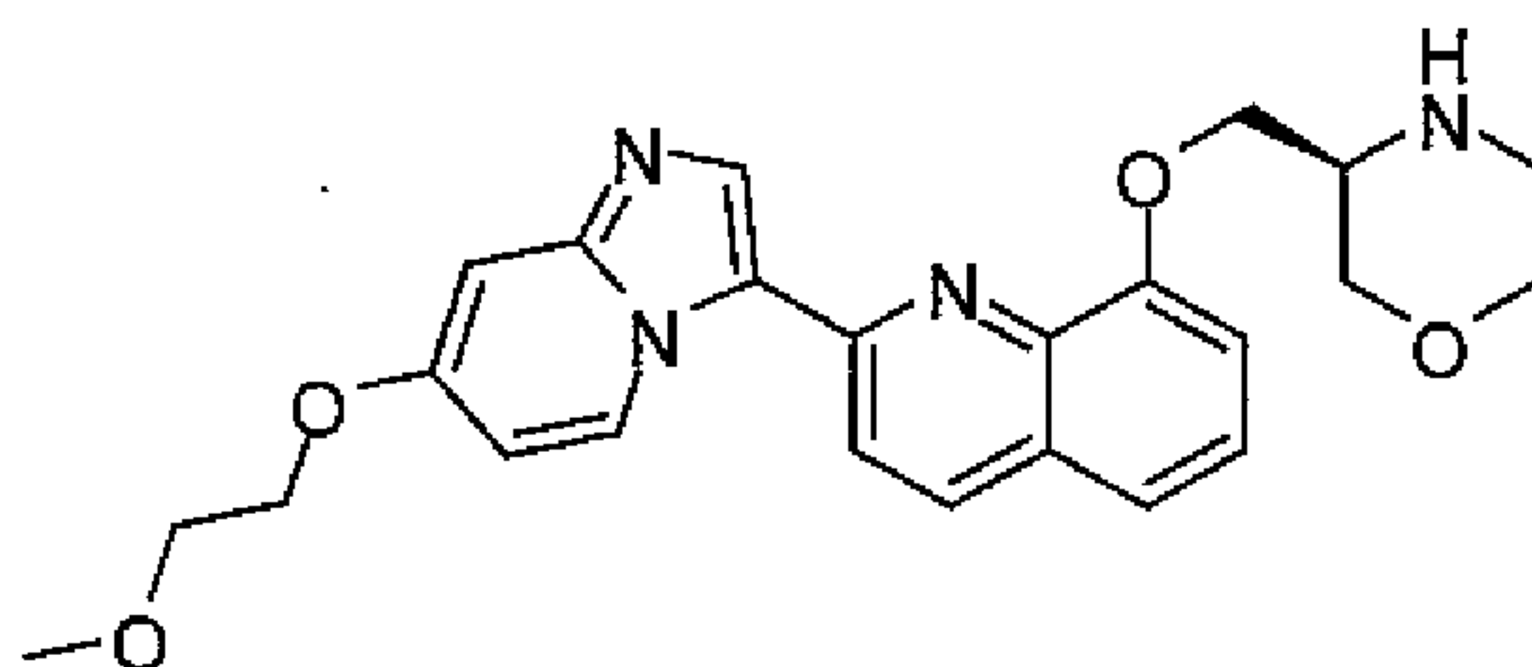
(S)-3-((2-(7-(2-Methoxyethoxy)imidazo[1,2-a]pyridin-3-yl)quinolin-8-yloxy)methyl)morpholine
