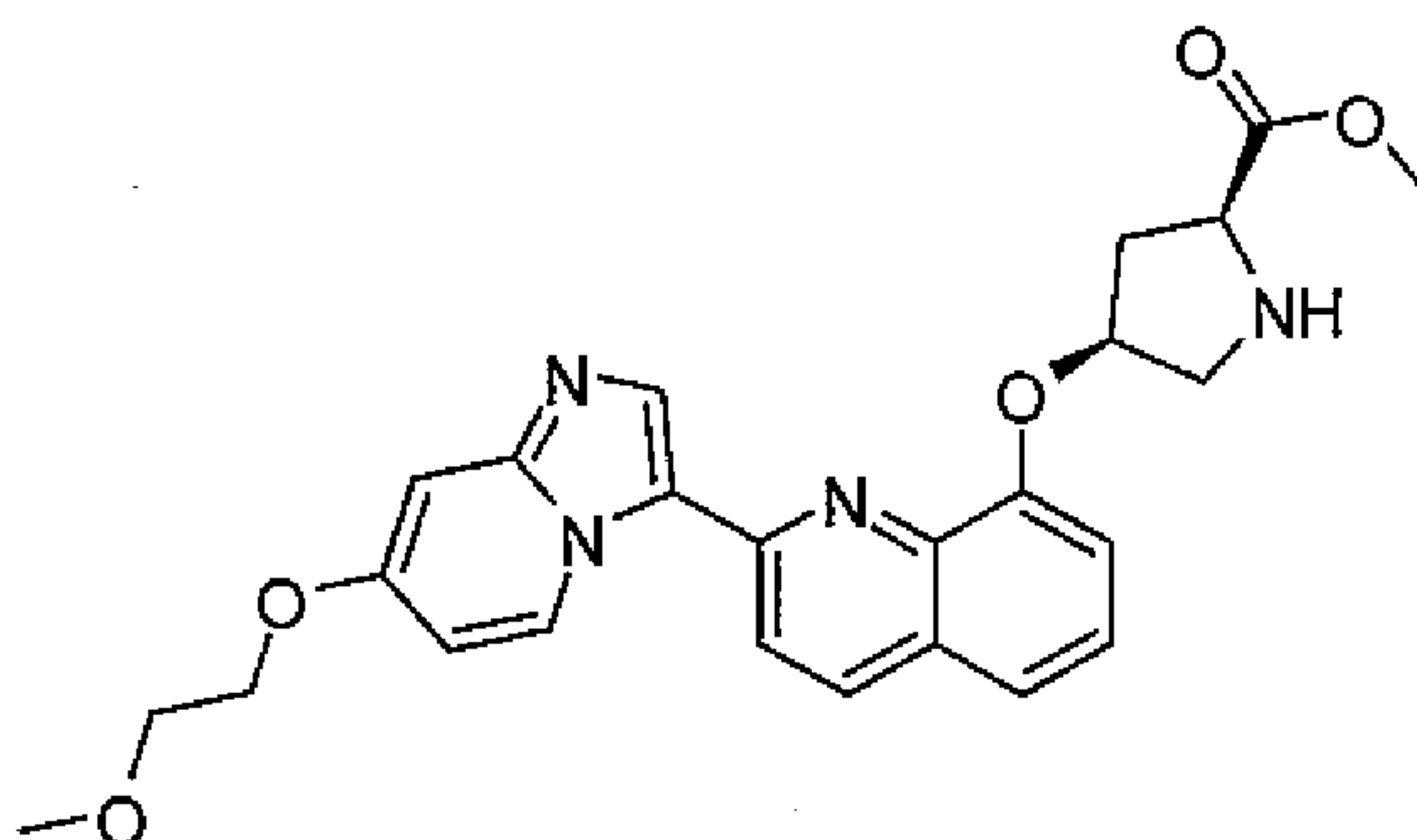
(2S,4S)-Methyl 4-(2-(7-(2-methoxyethoxy)imidazo[1,2-a]pyridin-3-yl)quinolin-8-yloxy)pyrrolidine-2-carboxylate
