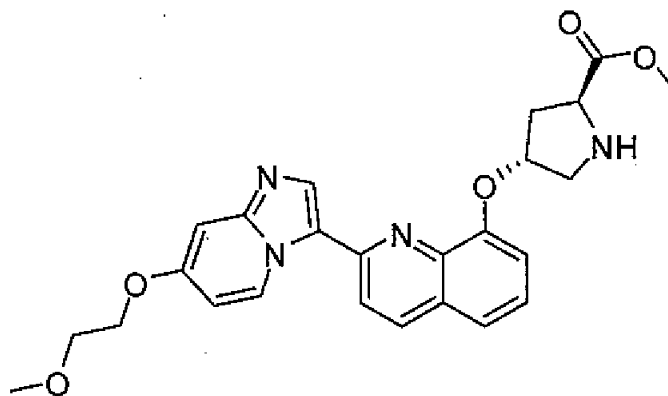
(2S,4R)-Methyl 4-(2-(7-(2-methoxyethoxy)imidazo[1,2-a]pyridin-3-yl)quinolin-8-yloxy)pyrrolidine-2-carboxylate
