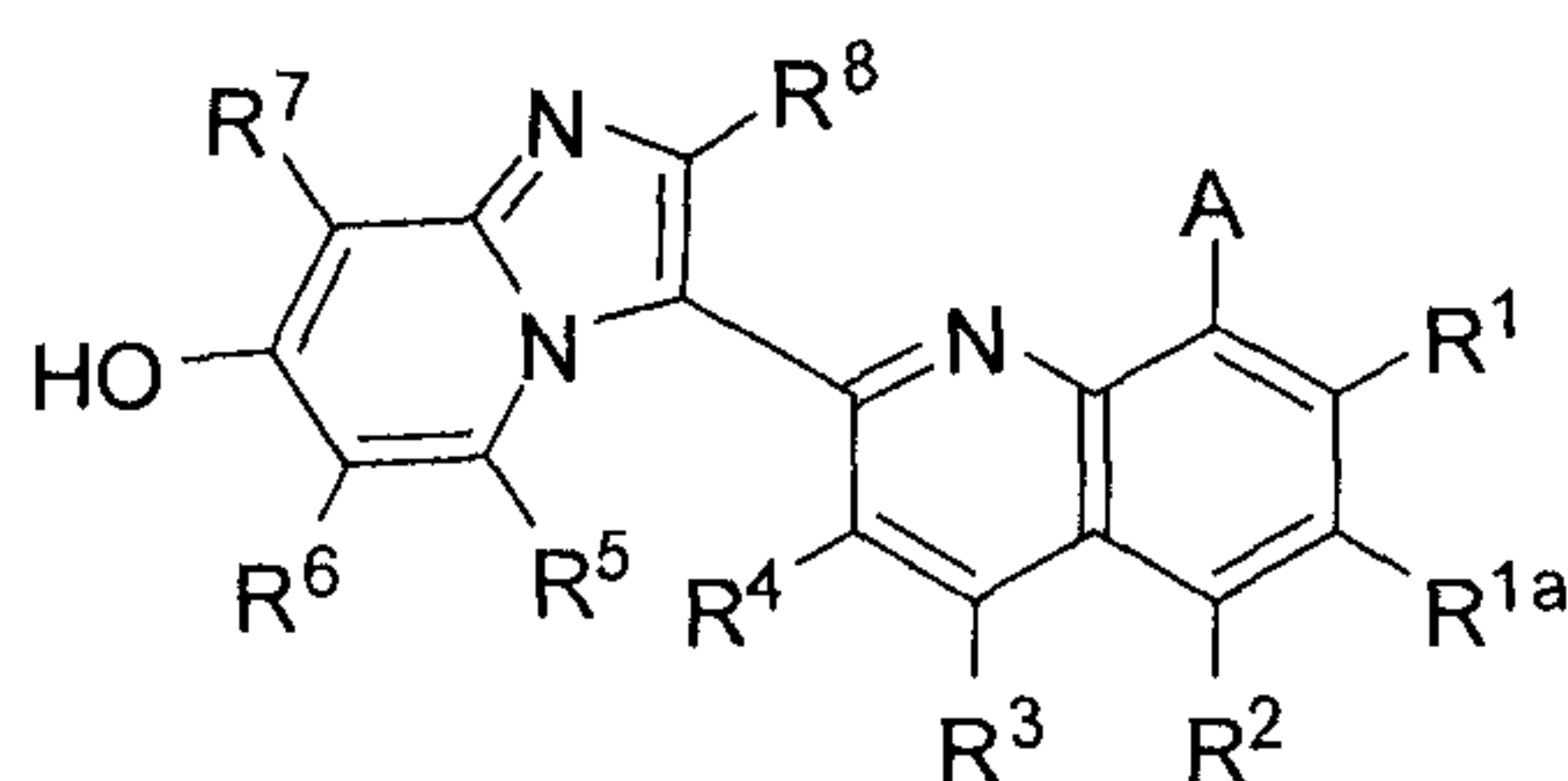
III
