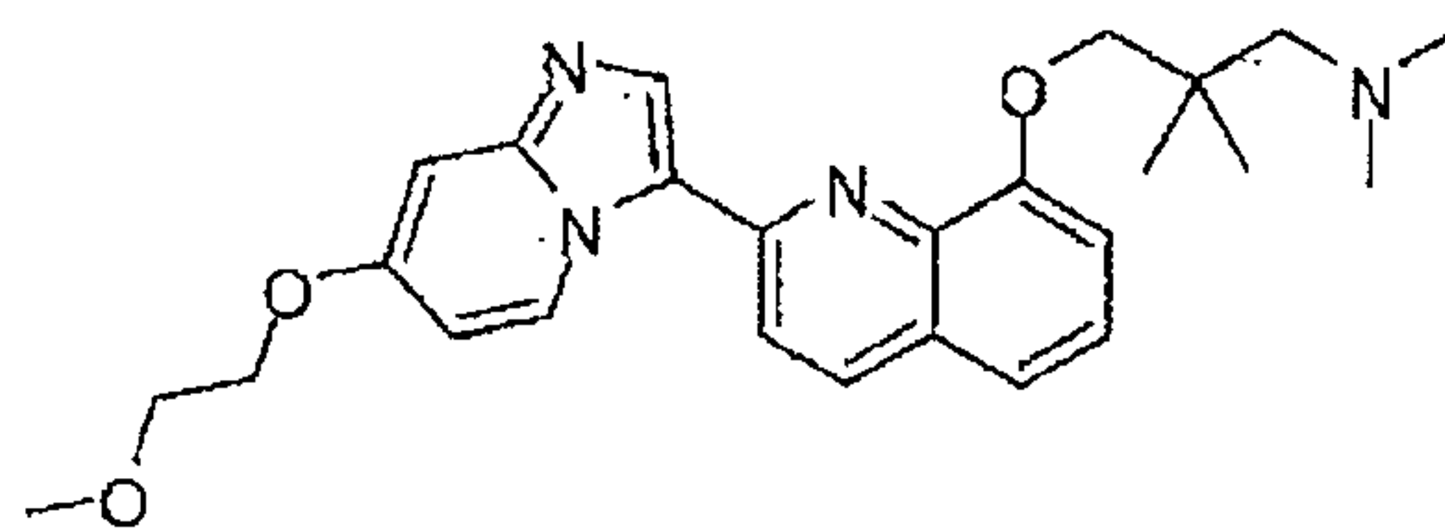
3-(2-(7-(2-methoxyethoxy)imidazo[1,2-a]pyridin-3-yl)quinolin-8-yloxy)-N,N,2,2-tetramethylpropan-1-amine
