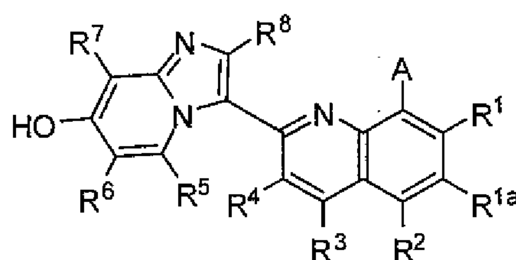
III
