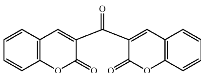
Chemical Formula 1
