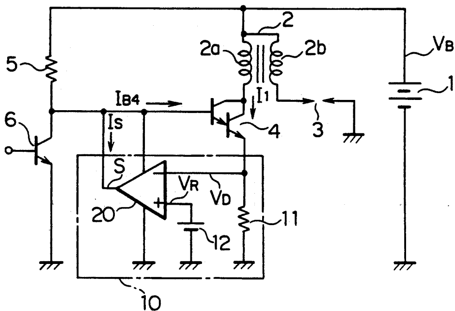
FIG. 3 PRIOR ART
