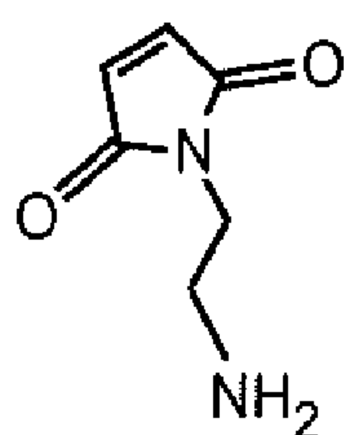
C2-Mal
