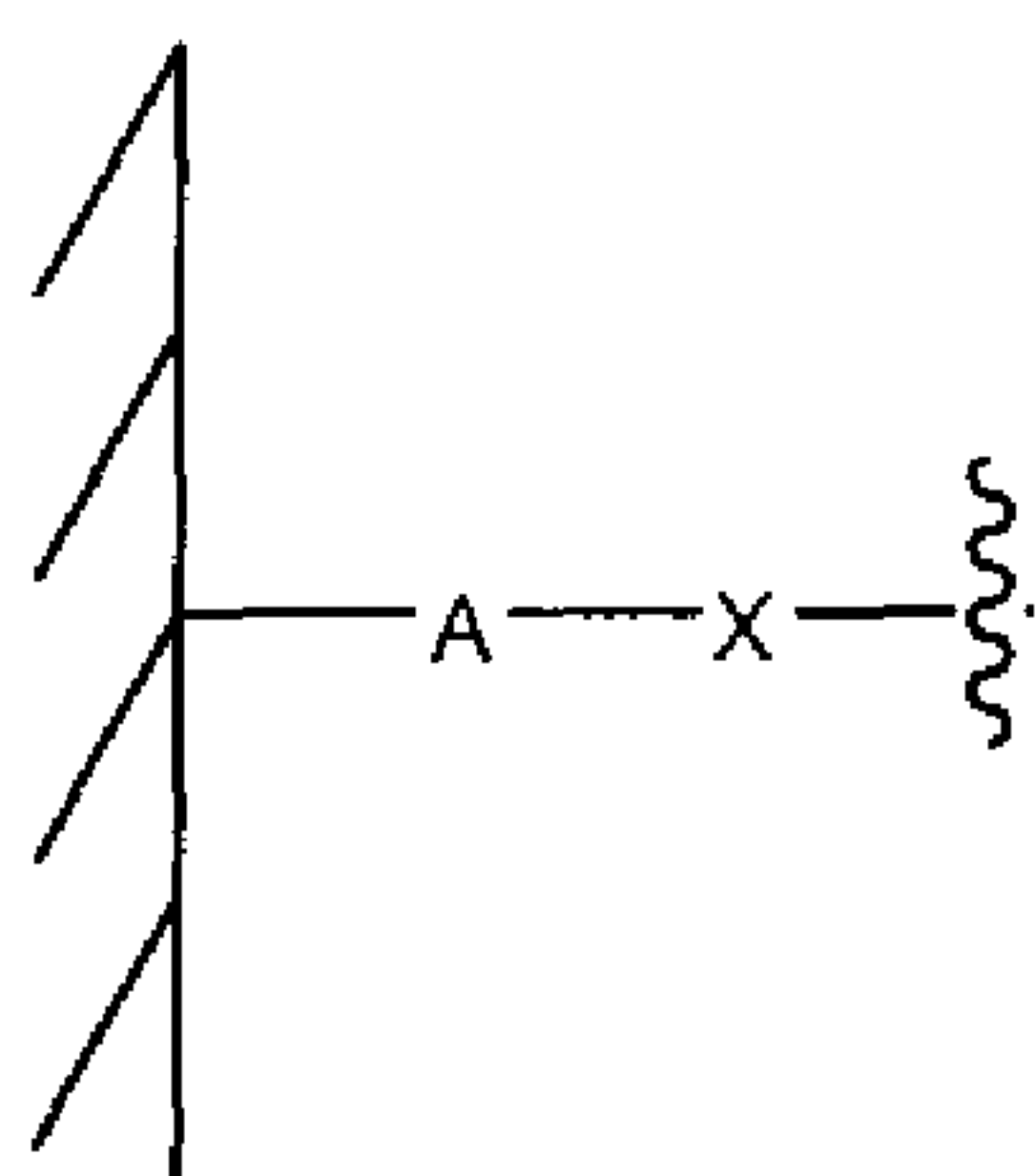
Structure 1
