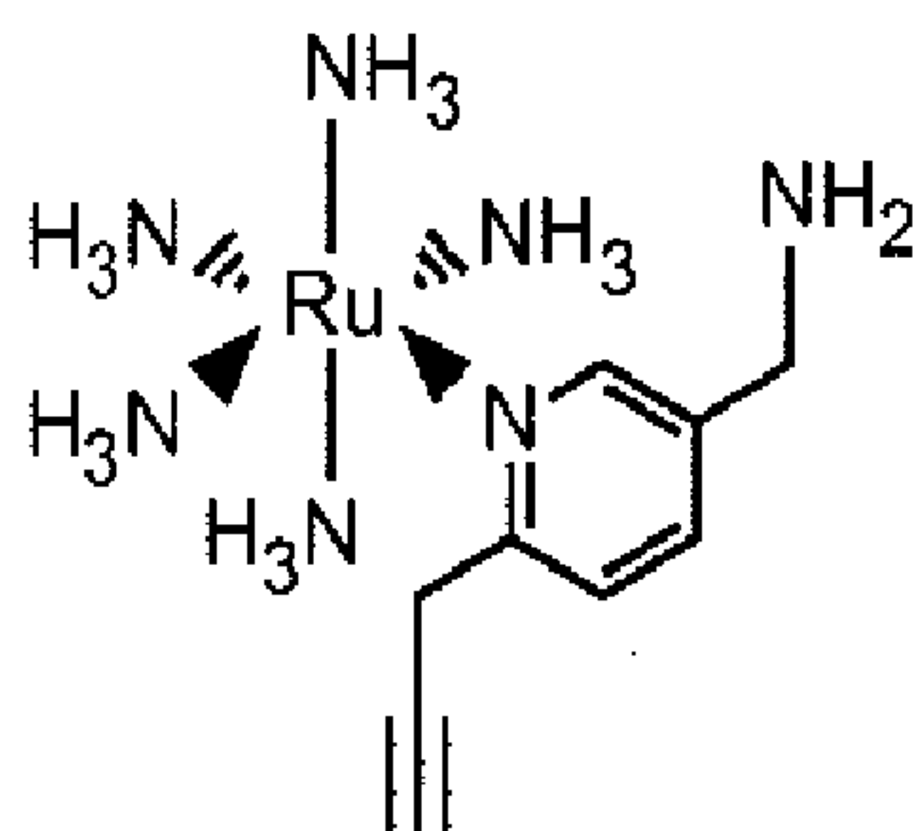
Monodentate
