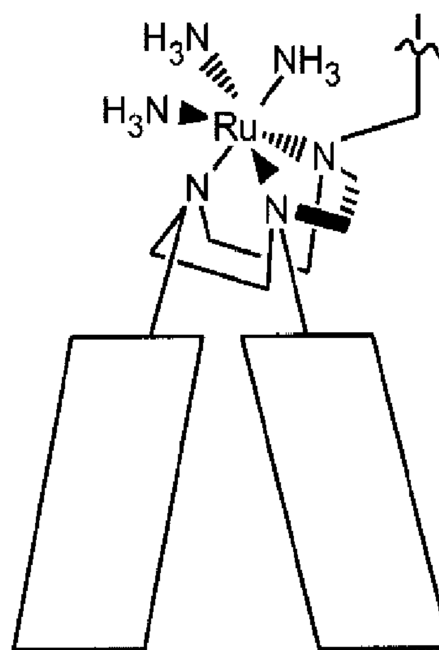
Multidentate
