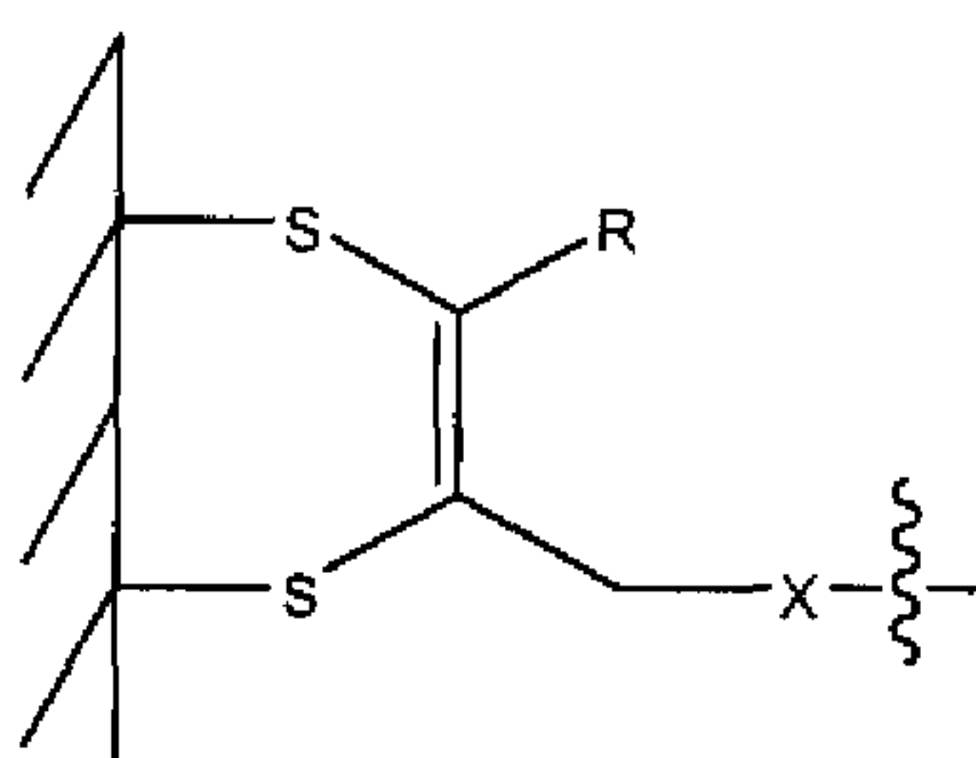
Structure 4
