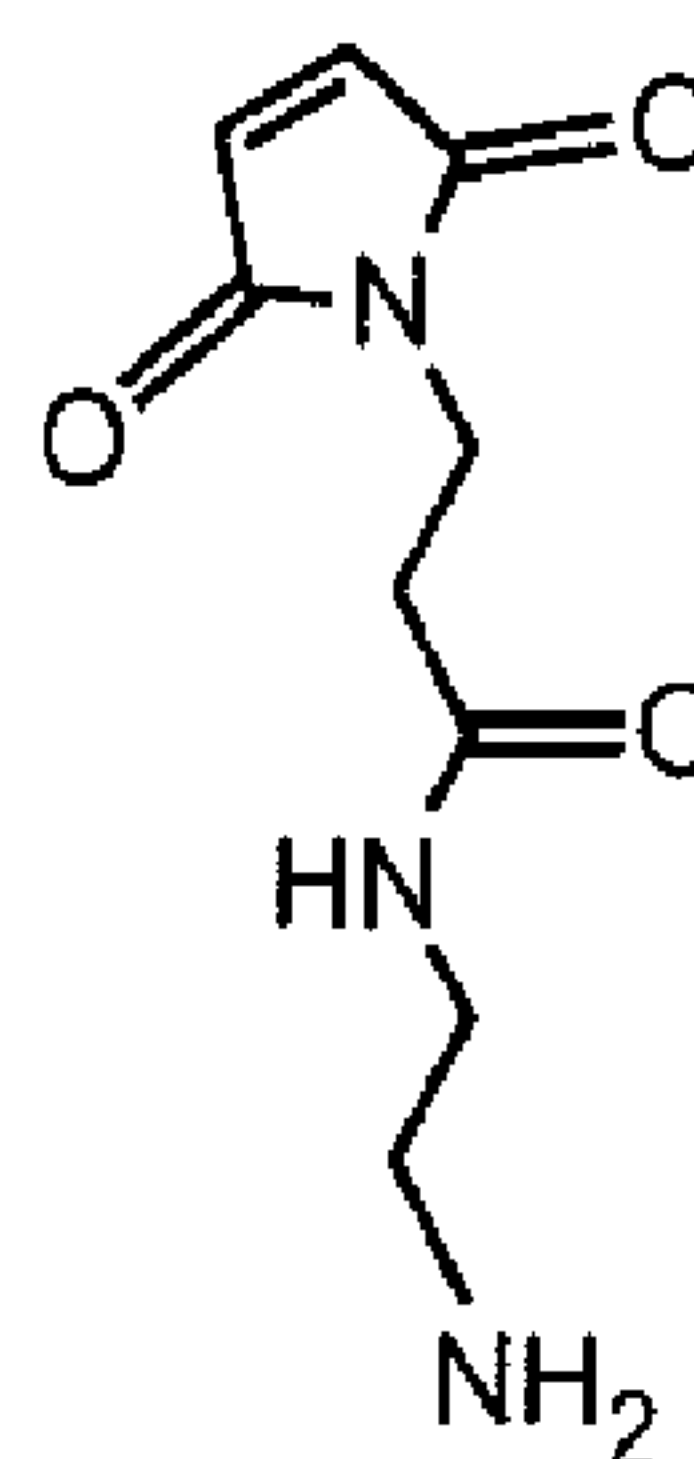
C6-Mal
