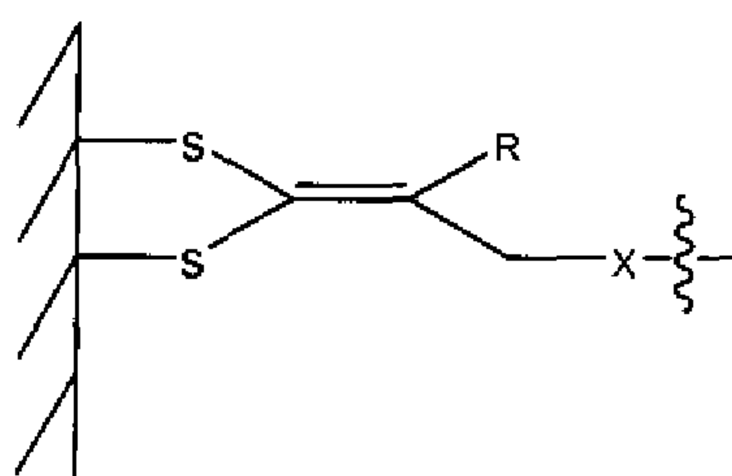
Structure 4
