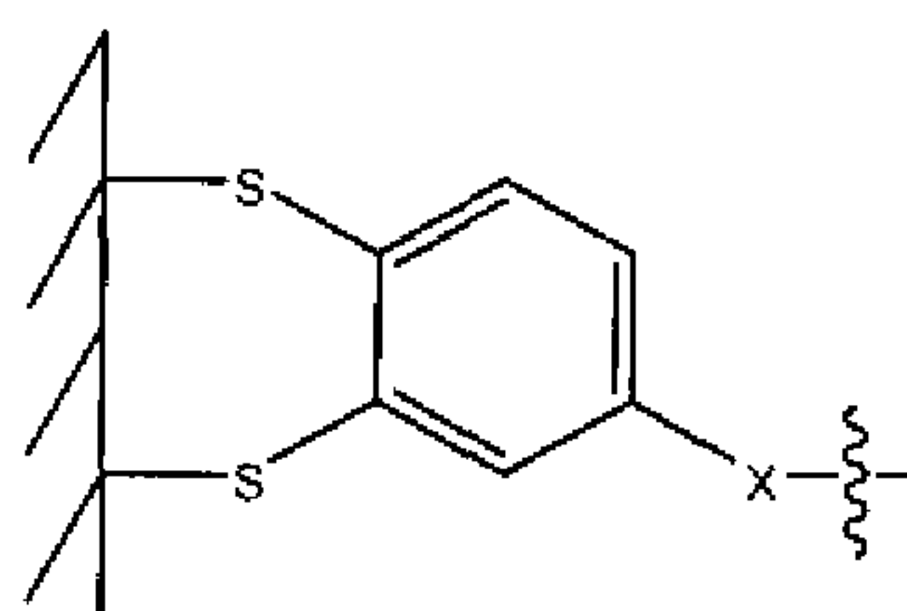
Structure 3
