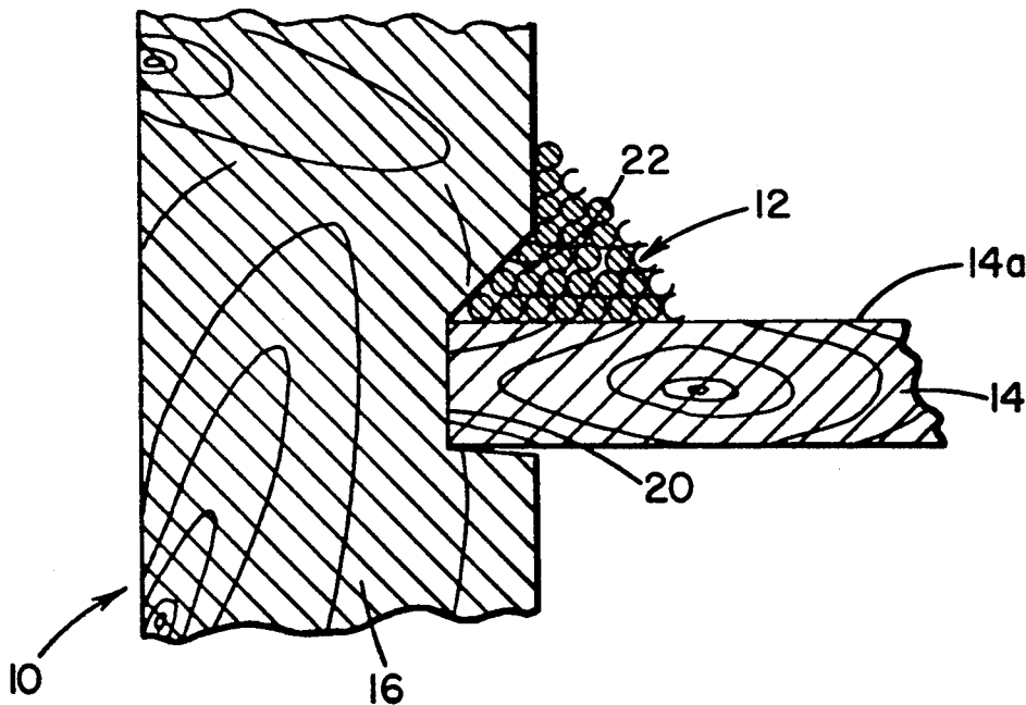
FIG. IIA (PRIOR ART)
